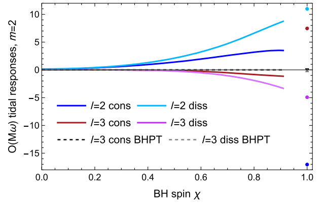
FIG. 3. Dependence on \ell of the O(M\omega) coefficients of the tensor responses for m = 2 . Blue tones indicate the quadrupole, red-pink the octupole, with darker/lighter hues corresponding to the conservative/dissipative coefficients. Dashed lines indicate the coefficients from black hole perturbation theory (BHPT). Circles indicate the values for extremal spins. Note that the conservative coefficient (darker blue and red curves) has a non-trivial behavior near extremality, including a change in sign.
