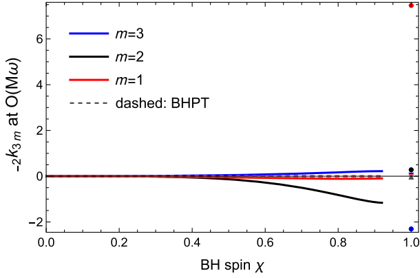
FIG. 2. The figure depicts Octupolar conservative tidal responses ( \ell = 3 ) for gravitational perturbation ( s = -2 ) for different choices of m . Dashed curves indicate the BHPT results (identical to the EFT for |m| = l , see Eq. (181)). The other conservative responses are obtained from EFT, and follow from substitution of Eq. (181) in Eq. (99) and then in Eq. (92), respectively. Dots indicate the values for extremal spins, obtained from the above procedure.
