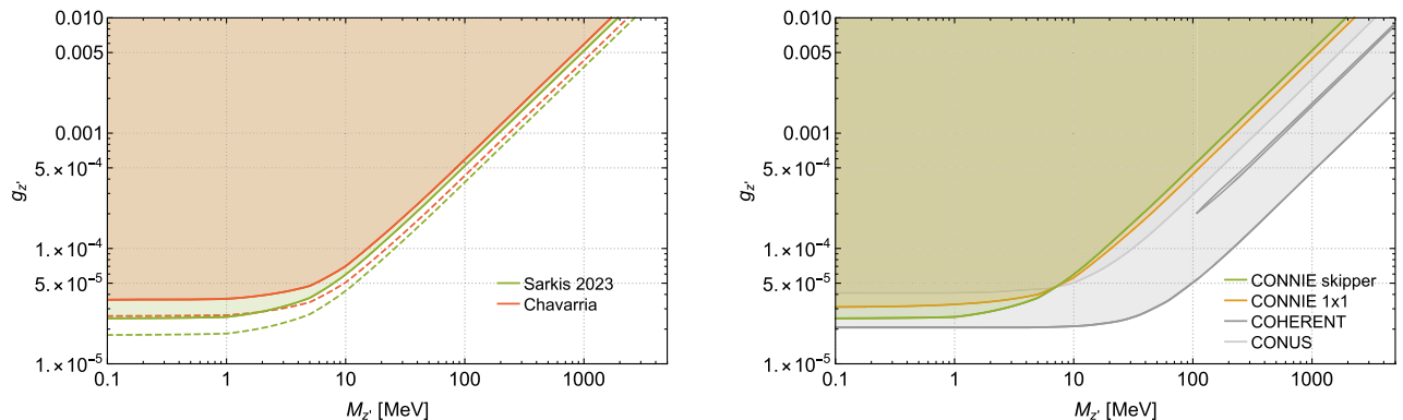
FIG. 7. (Left) CONNIE Skipper-CCD exclusion limits (solid lines) at 95% CL from the \text{CE}\nu\text{NS} detection channel for a light vector mediator Z' , assuming the simplified universal model [84], and considering quenching factors from Sarkis [71] (green) and Chavarria [74] (red); and projections of these limits (dashed) assuming a zero difference between the rates and a five times smaller statistical error. (Right) Comparison between CONNIE exclusion limits at 95% CL from Skipper-CCDs considering the quenching factor from Sarkis [71] (green) and the standard-CCD [46] (red). For comparison, limits at the 90% CL from COHERENT (CsI + Ar) [85] and CONUS ( k = 0.16 ) data [83] are also shown.
