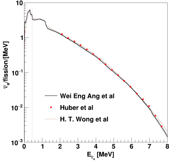
FIG. 9. Total reactor antineutrino spectrum per fission in the reactor per MeV for three models: (black) Wei Eng Ang et al. [66], (red) Huber et al. [95] and (brown) Wong [96]. The error band for Wei model is computed according to [68,75]. The dotted vertical line denotes the neutrino energy threshold for Skipper-CCDs at CONNIE.
