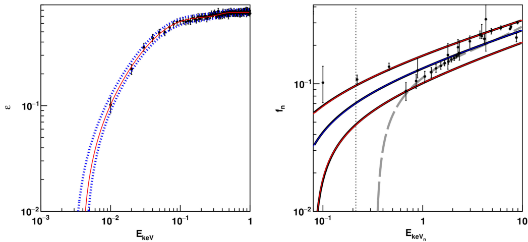
FIG. 10. (Left) Efficiency points with error bars compared with the fit function from Eq. (B1) (red). (Right) Ionization efficiency from [71] (blue), for the upper and lower curves (red) compared with the fit function from Eq. (B2) (black) and from Chavarria [65] (long dash). The vertical dotted line shows the threshold recoil energy (0.24 keV n ) for Skipper-CCDs using Eq. (B2). Also shown are the measurements extracted from Refs. [71,97].
