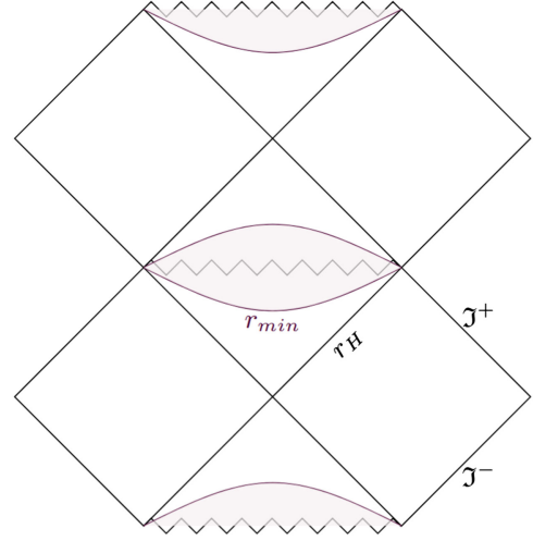
FIG. 3. Conformal diagram to illustrate the causal structure of our cyclic Kruskal universe. The purple region is “cut out” and the interior region of the black hole is glued to the interior region of the white hole along the hypersurface with coordinate r_{\min} . The exterior regions are disconnected. This chain of black and white holes can continue infinitely far above and below.
