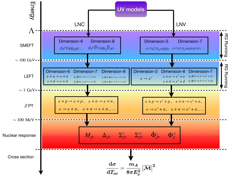
FIG. 1. Comprehensive effective field theory framework for evaluating the cross section of CE \nu NS.
