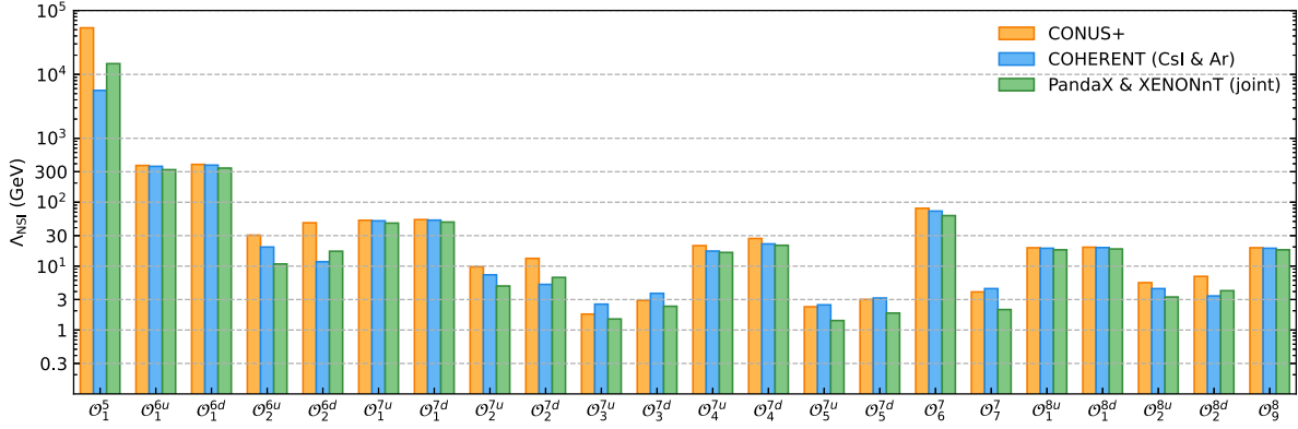
FIG. 3. For CE \nu NS processes initiated by an electron-flavor neutrino, we present lower bounds at 90% C.L. on the effective scale \Lambda_{\text{NSI}} (in GeV) associated with individual LEFT operators \mathcal{O}_1^S , \mathcal{O}_1^{6u} , \mathcal{O}_1^{6d} , \mathcal{O}_2^{6u} , \mathcal{O}_2^{6d} , \mathcal{O}_1^{7u} , \mathcal{O}_1^{7d} , \mathcal{O}_2^{7u} , \mathcal{O}_2^{7d} , \mathcal{O}_3^{7u} , \mathcal{O}_3^{7d} , \mathcal{O}_4^{7u} , \mathcal{O}_4^{7d} , \mathcal{O}_5^{7u} , \mathcal{O}_5^{7d} , \mathcal{O}_6^7 , \mathcal{O}_7^7 , \mathcal{O}_1^{8u} , \mathcal{O}_1^{8d} , \mathcal{O}_2^{8u} , \mathcal{O}_2^{8d} , and \mathcal{O}_9^8 . The limits are obtained by turning on one operator at a time. The orange, blue, and green bars correspond to constraints from CONUS+, COHERENT (CsI and Ar combination), and the PandaX-4T and XENONnT combination, respectively.
