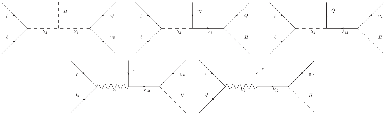
FIG. 6. Contributions to \mathcal{O}_{QuLLH} from the UV completions with S_2 , S_4 , F_8 , F_{12} , V_5 , and V_9 particles.
