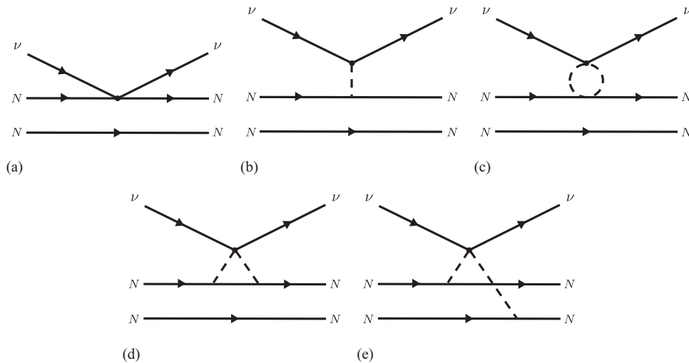
FIG. 2. Diagrams (a) and (b) show the leading-order one-body current contributions. Diagrams (c) and (d) show loop corrections to the one-body currents. Diagram (e) shows the two-body current contribution.
