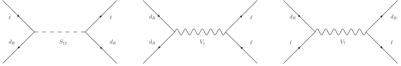
FIG. 5. Contributions to \mathcal{O}_{ld} from the UV completions with S_{12} , V_1 , and V_7 particles.
