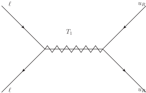
FIG. 7. Contribution to \mathcal{O}_{\ell^2 u^2 D^2}^{(2)} from the UV completions with T_1 particle.
