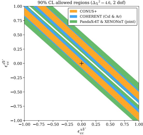
FIG. 4. The 90% C.L. allowed regions in the (\epsilon_{ee}^{uV}, \epsilon_{ee}^{dV}) plane are derived from the CONUS+ (orange) and COHERENT (CsI & Ar) CE \nu NS measurements together with the combined constraint from the PandaX-4T + XENONnT (green) solar ^8\text{B} analysis.
