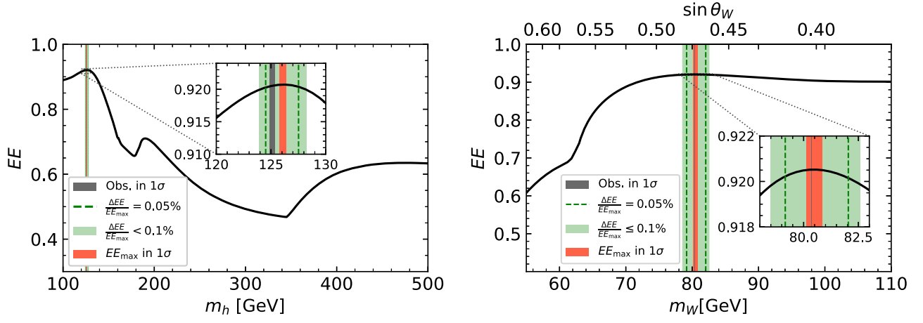
FIG. 2. Entanglement entropy of Higgs boson decays as a function of the Higgs boson mass (left) and m_W (right). The gray band marks the experimentally observed SM values ( 1\sigma ), the red band shows the EE_{\max} yield with its 1\sigma uncertainty from SM inputs and theory, and the green band (dashed lines) indicates the near-maximal-EE region with \Delta EE/EE_{\max} < 0.1\% ( 0.05\% ).
