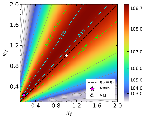
FIG. 6. Gibbs-Shannon entropy [Eq. (E3)] as a function of Standard Model parameters. Upper left: dependence on the Higgs boson mass m_h . Upper right: dependence on the W boson mass m_W . Bottom: distribution in the (\kappa_f, \kappa_V) plane. Color coding follows the same definition as in Fig. 2.
