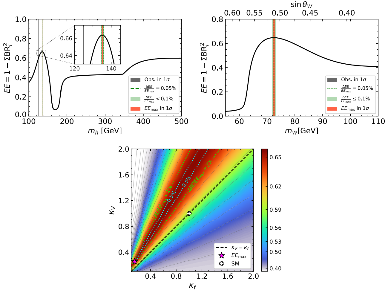
FIG. 5. Entanglement-entropy distribution for Standard Model parameters using EE = 1 - \sum_i BR_i^2 . Upper left: EE as a function of Higgs boson mass m_h . Upper right: EE as a function of W boson mass m_W . Bottom: EE distribution in the (\kappa_f, \kappa_V) plane. Color coding follows the same convention as in Fig. 2.
