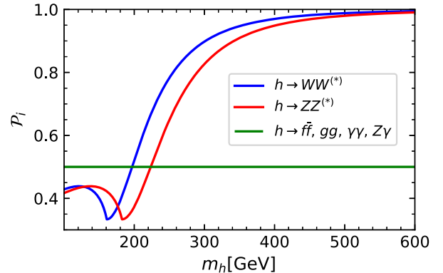
FIG. 1. Spin factors \mathcal{P}_i for each Higgs boson decay channel as a function of m_h .
