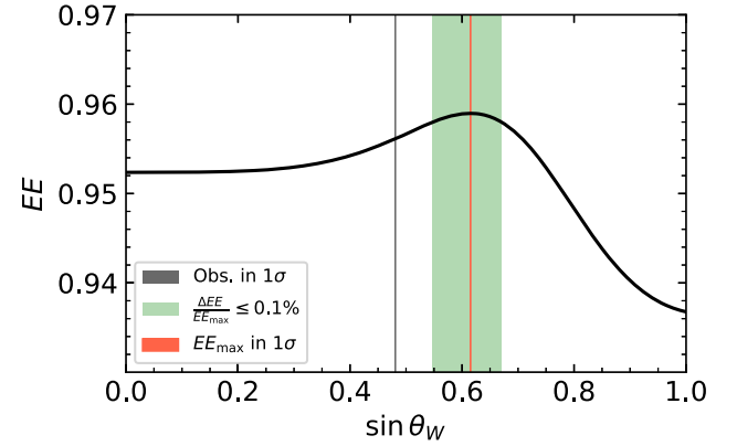
FIG. 7. Dependence of the entanglement entropy on the weak mixing angle for Z boson decays. Color regions follow the same convention as in Fig. 2.
