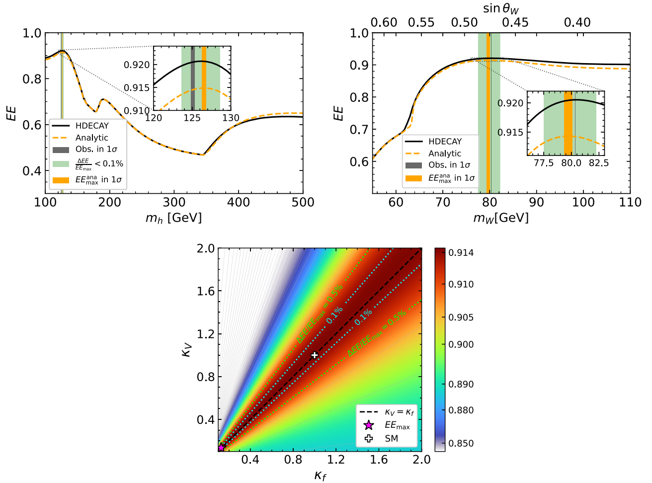
FIG. 4. Distributions of the entanglement entropy using analytical formulas for the Higgs boson decay widths. Upper left: dependence of the EE on the Higgs boson mass m_h . The black solid line shows results from HDECAY, while the orange dashed line represents the EE calculated using analytical formulas. The orange band indicates EE_{\max} with its 1\sigma uncertainty from SM inputs and theoretical uncertainties. Other colored codes follow the same definition as in Fig. 2. Upper right: dependence of the EE on the W boson mass m_W . Bottom: EE distribution in the (\kappa_f, \kappa_V) plane.
