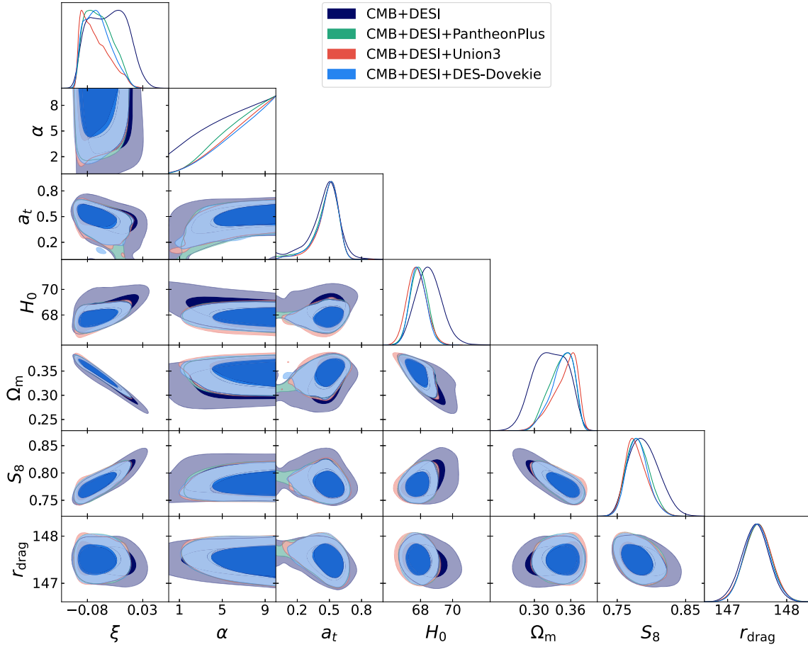
FIG. 10. One-dimensional posterior distributions and two-dimensional joint contours for the most relevant parameters of the IPEDGen scenario from different combinations of cosmological datasets.
