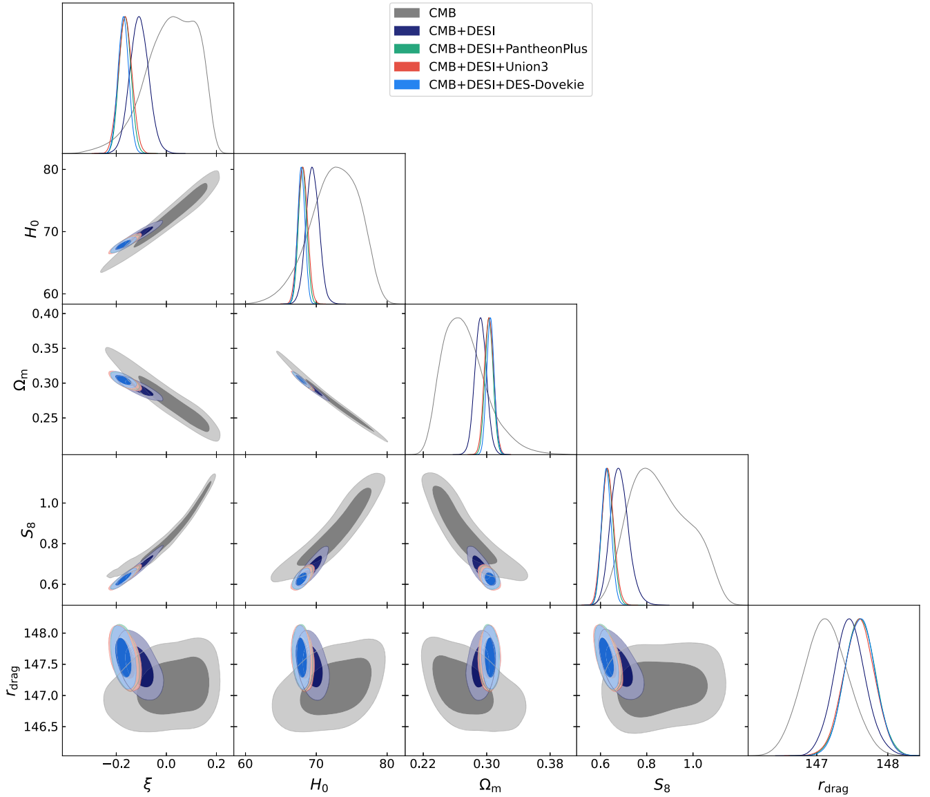
FIG. 7. One-dimensional posterior distributions and two-dimensional joint contours for the most relevant parameters of the IPeDE scenario from different combinations of cosmological datasets.
