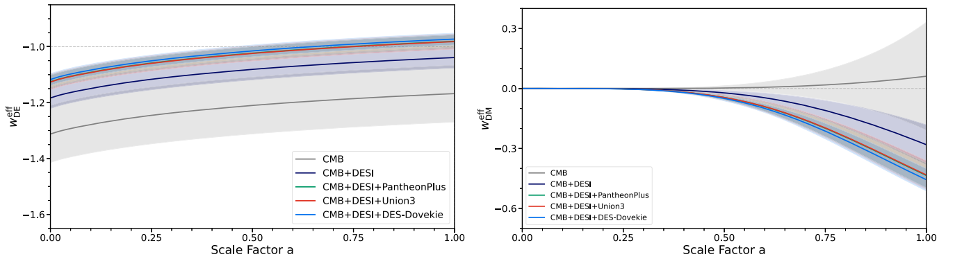
FIG. 9. Evolution of the effective EOS parameters, including their 68% CL credible regions, as a function of the scale factor for IPEDe scenario. The left panel shows w_{\text{DE}}^{\text{eff}} , while the right panel shows w_{\text{DM}}^{\text{eff}} . In both plots, the curve obtained from CMB + DESI + PantheonPlus (green) is indistinguishable from that of CMB + DESI + Union3 (red), since the constraints from these combined datasets are nearly identical.
