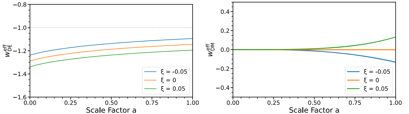
FIG. 2. Evolution of the effective EOS parameters for different values of the coupling parameter \xi for the IPEDE model. The left panel shows w_{\text{DE}}^{\text{eff}} , while the right panel shows w_{\text{DM}}^{\text{eff}} .
