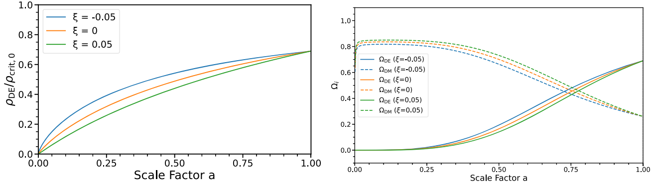
FIG. 1. Evolution of \rho_{\text{DE}}/\rho_{\text{crit},0} (left panel) and evolution of the DE and CDM density parameters, \Omega_{\text{DE}} and \Omega_{\text{CDM}} (right panel) for the IPEDE model.
