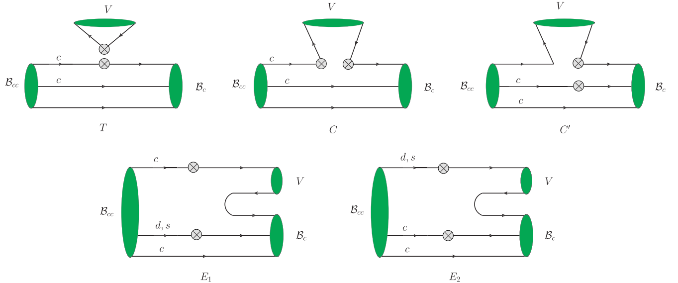
FIG. 1. The five tree-level topological diagrams for two-body nonleptonic decays \mathcal{B}_{cc} \rightarrow \mathcal{B}_c V of the doubly charmed baryons \mathcal{B}_{cc} = (\Xi_{cc}^{++}, \Xi_{cc}^+, \Omega_{cc}^+) .
