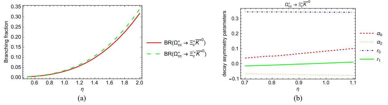
FIG. 3. The dependence of the branching ratios and decay parameters on the model parameter \eta .
