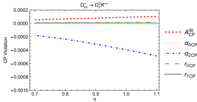
FIG. 4. The dependence of the CP violations on the model parameter \eta .
