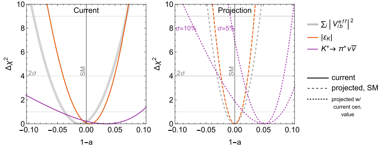
FIG. 1. Values of \Delta\chi^2 as a function of the deviation in the scaling of the CKM b column, (1-a) . In the left panel, the solid gray, orange, and purple curves show the current bounds from \sum_i |V_{ib}|^2 (Eq. (5)), |\epsilon_K| , and \mathcal{B}(K^+ \rightarrow \pi^+ \nu \bar{\nu}) , respectively. In the right panel, the dashed and dotted curves are future projections under the assumptions detailed in Table I. Agreement with the SM is assumed for the \sum_i |V_{ib}|^2 and |\epsilon_K| projected curves, while scenarios where the current slight excess in \mathcal{B}(K^+ \rightarrow \pi^+ \nu \bar{\nu}) persists are shown in dotted purple, for uncertainties of \mathcal{O}(5\%, 10\%) .
