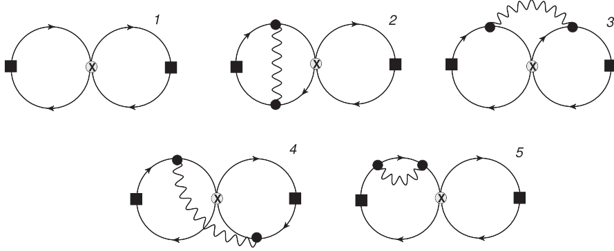
FIG. 3. Feynman diagrams contributing to \langle \mathcal{O}_{\Gamma'}(x) \mathcal{O}_{\Gamma\Gamma}(0) \mathcal{O}_{\Gamma''}(y) \rangle , to order \mathcal{O}(g^0) (diagram 1) and \mathcal{O}(g^2) (the remaining diagrams). Wavy (solid) lines represent gluons (quarks). A circled cross denotes the insertion of the four-quark operator, and the solid squares denote the quark bilinear operators. Diagrams 2–5 have also mirror variants.
