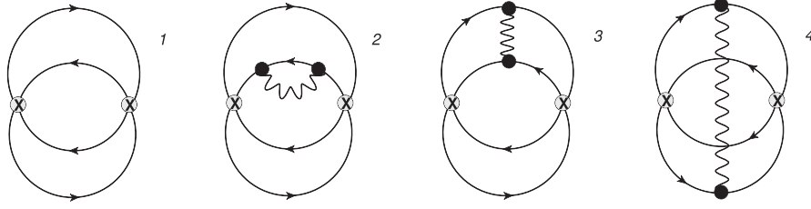
FIG. 2. Feynman diagrams contributing to \langle \mathcal{O}_{\Gamma\Gamma}(x) \mathcal{O}_{\Gamma\Gamma}^\dagger(y) \rangle , to order \mathcal{O}(g^0) (diagram 1) and \mathcal{O}(g^2) (the remaining diagrams). Wavy (solid) lines represent gluons (quarks). Diagrams 2 and 4 have also mirror variants.
