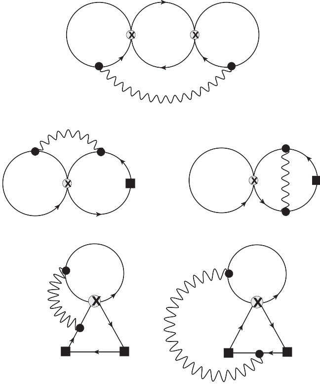
FIG. 4. Representative Feynman diagrams contributing to two-point and three-point Green's functions at the next-to-leading order, \mathcal{O}(g^2) . Wavy (solid) lines represent gluons (quarks). The four-quark operator \mathcal{O}_{\Gamma\Gamma'} is indicated by a circled cross. Bilinear operators, \mathcal{O}_{\Gamma} are denoted by solid squares, while solid circles correspond to interaction vertices from the action. The first row shows examples of two-point Green's functions of the form \langle \mathcal{O}_{\Gamma\Gamma'}(x) \mathcal{O}_{\Gamma\Gamma'}^\dagger(y) \rangle . The second row includes diagrams for two-point Green's functions between a four-quark operator and a bilinear, \langle \mathcal{O}_{\Gamma\Gamma'}(x) \mathcal{O}_{\Gamma}^\dagger(y) \rangle . The last row illustrates three-point Green's functions involving one four-quark and two bilinear operators: \langle \mathcal{O}_{\Gamma}(x) \mathcal{O}_{\Gamma\Gamma'}(y) \mathcal{O}_{\Gamma'}^\dagger(z) \rangle . All these diagrams do not vanish in dimensional regularization (DR) or by color algebra (e.g., by Fierz rearrangements), but they do vanish when the four-quark operator is traceless due to the presence of partial traces over a traceless operator.
