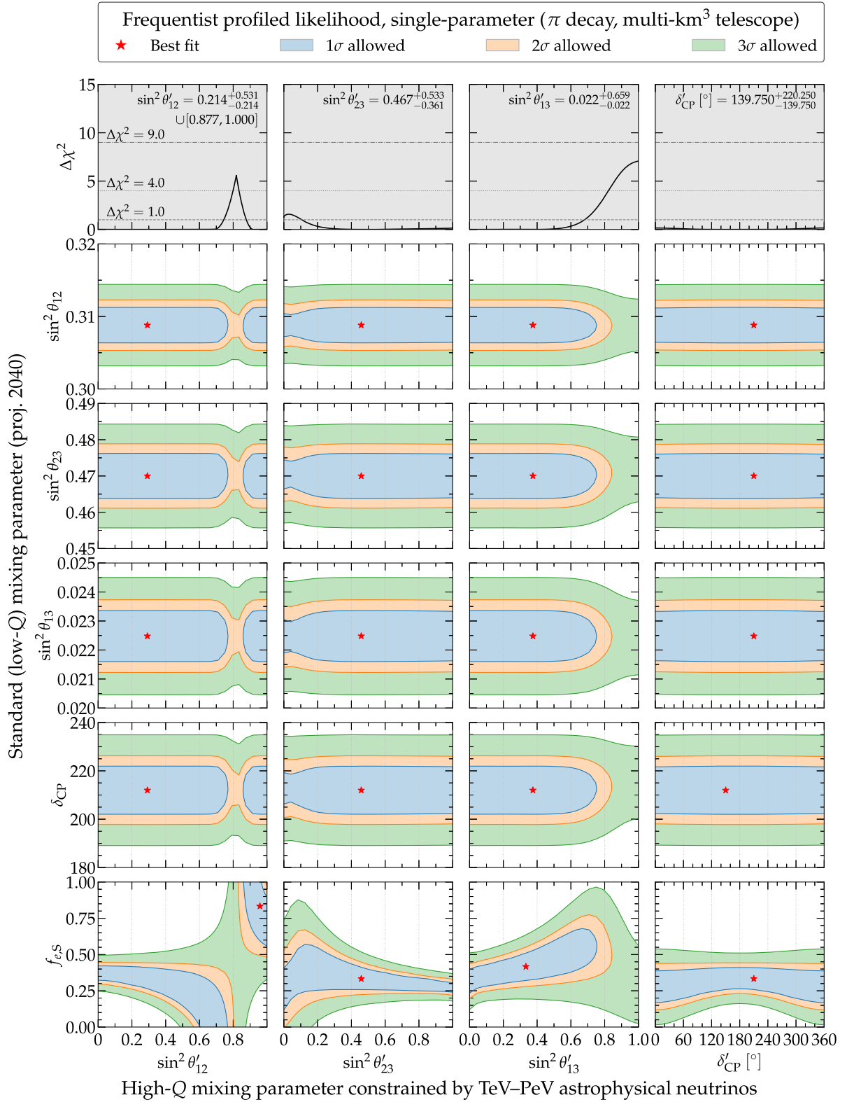
FIG. 20. Future TeV–PeV pairwise profiled likelihood using km 3 -scale detectors. The flavor-measurement likelihood uses the combined exposure of IceCube, Baikal-GVD, and KM3NeT to the year 2040, assuming neutrino production via full pion decay and f_{\tau,S} = 0 . See Appendix E for details.
