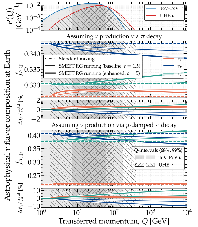
FIG. 7. Example renormalization-group running of the flavor composition at Earth. The RG evolution of the flavor fractions f_{\alpha\oplus} and their relative deviations from standard oscillations ( \Delta f_{\alpha\oplus}/f_{\alpha\oplus}^{\text{std}} ) are shown as a function of the momentum transfer, Q , under our example SMEFT scheme (Sec. IV E). Top panel: probability distribution of momentum transfer in \nu N DIS for TeV–PeV and UHE astrophysical neutrinos, indicating their respective 68% and 99% containment intervals. Lower panels: RG running assuming neutrino production via full and muon-damped pion decay, evaluated with baseline [ c_{\text{SMEFT}} = 1.5 in Eq. (19)] and enhanced ( c_{\text{SMEFT}} = 5.0 ) benchmark SMEFT couplings.
