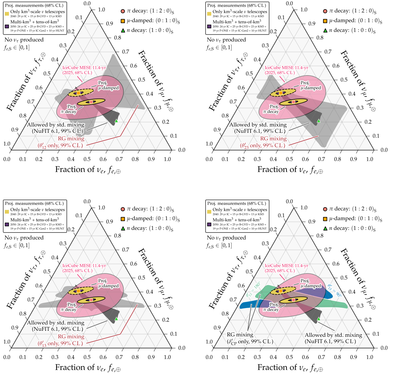
FIG. 19. Impact of individual high- Q mixing parameters on the expected flavor composition at Earth. Each panel displays the 99% CL allowed region when only one high- Q parameter is varied (top left: \theta'_{12} , top right: \theta'_{23} , bottom left: \theta'_{13} , bottom right: \delta'_{CP} ), while the others remain fixed to their standard values. The initial source composition is generalized as f_{e,S} \in [0, 1] and f_{\tau,S} = 0 . The projections of future km 3 -scale and tens-of-km 3 -scale detector sensitivities are overlaid to demonstrate diagnostic potential.
