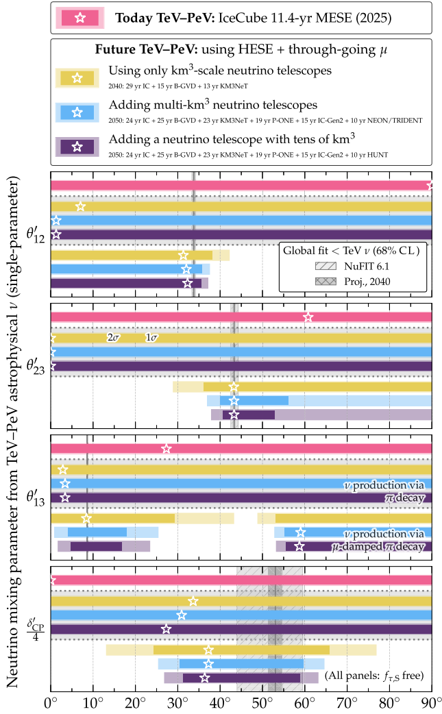
FIG. 23. Constraints on the high- Q neutrino mixing parameters with TeV–PeV astrophysical neutrinos, with f_{\tau,S} free. Same as Fig. 11 in the main text, but allowing for \nu_\tau production at the astrophysical sources, i.e., allowing f_{\tau,S} \in [0, 1] to float when constraining the mixing parameters.
