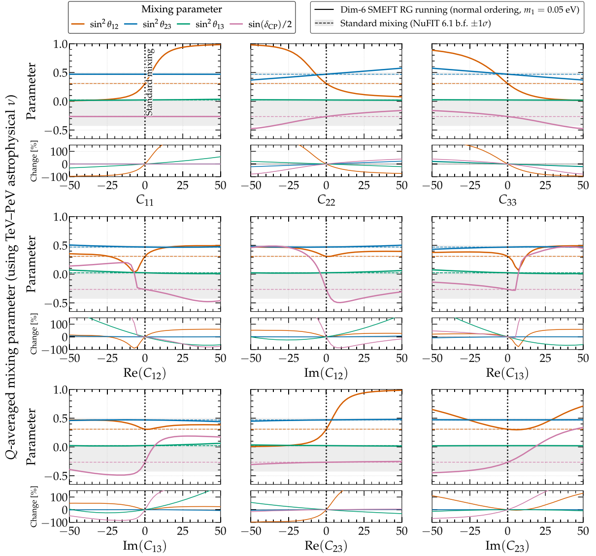
FIG. 6. Evolution of the Q -averaged neutrino mixing parameters with the SMEFT couplings. The physical parameters are integrated over the momentum distribution accessible by a typical TeV–PeV astrophysical neutrino energy spectrum ( \propto E_\nu^{-2.5} ), with subpanels detailing the relative change from standard mixing expectations. The pronounced volatility of the solar sector ( \theta_{12} , \delta_{CP} ), contrasted against the comparative rigidity of the reactor and atmospheric angles, illustrates how the Standard Model mass hierarchy intrinsically throttles anomalous flavor transitions. In this figure, we fix c_{\text{SMEFT}} = 1 and \Lambda_{\text{SMEFT}} = 1 TeV. See Sec. IV G for details.
