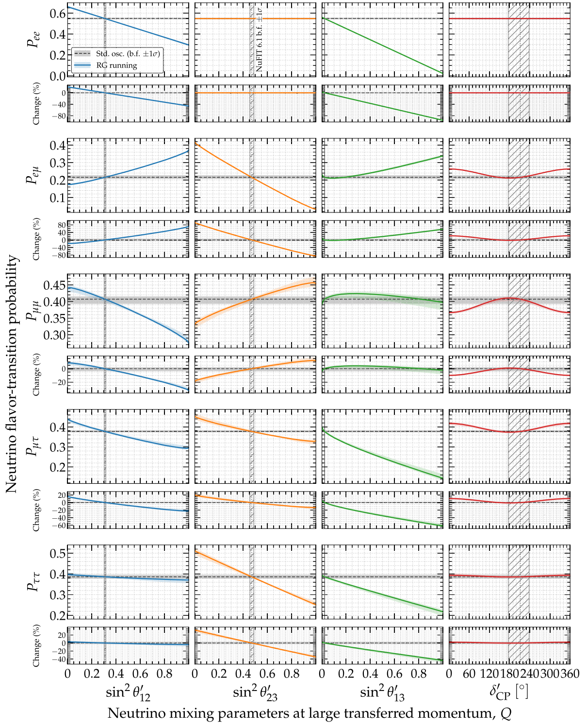
FIG. 2. Neutrino flavor-transition probabilities as a function of the modified high- Q mixing parameters. Rows display P_{ee} , P_{e\mu} , P_{\mu\mu} , P_{\mu\tau} , and P_{\tau\tau} computed via Eq. (3). Columns show independent variations of the high-energy parameters \sin^2 \theta'_{12} , \sin^2 \theta'_{23} , \sin^2 \theta'_{13} , and \delta'_{CP} , with the remaining parameters fixed to their standard low-energy values. We compare these RG-modified probabilities against the standard case [Eq. (2)]. Probability bands denote 1\sigma uncertainties. Vertical bands indicate NuFIT 6.1 best fit (“b.f.”) and 1\sigma intervals for the varied parameter, assuming normal mass ordering and including Super-Kamiokande data. Subpanels quantify the relative change, (P_{\alpha\beta} - P_{\alpha\beta}^{\text{std}})/P_{\alpha\beta}^{\text{std}} . See Sec. III B for details.
