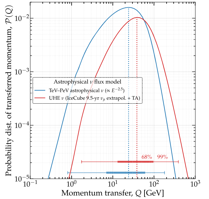
FIG. 17. Probability distribution of transferred momentum in \nu N deep inelastic scattering. The Q -distribution shown, \mathcal{P}(Q) in Eq. (B8), is computed by weighing the distributions corresponding to individual neutrino energies by the energy spectrum of high-energy astrophysical neutrinos, separately for the TeV–PeV and UHE ( > 100 PeV) ranges, as shown in Fig. 16.
