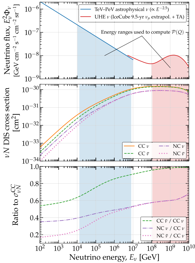
FIG. 16. Ingredients to compute the probability distribution of transferred momentum. Top: high-energy astrophysical neutrino flux models to compute the energy weighing in TeV–PeV and UHE ranges, \mathcal{P}(Q) in Eq. (B8). Middle: total cross section for neutrino and antineutrino charged-current (CC) and neutral-current (NC) deep inelastic scattering on nucleons, computed using the CT18NNLO parton distribution functions. Bottom: ratios between the different interaction channels, used when computing the channel-combined Q -distribution, \mathcal{P}_{\text{comb}} in Eq. (B6).
