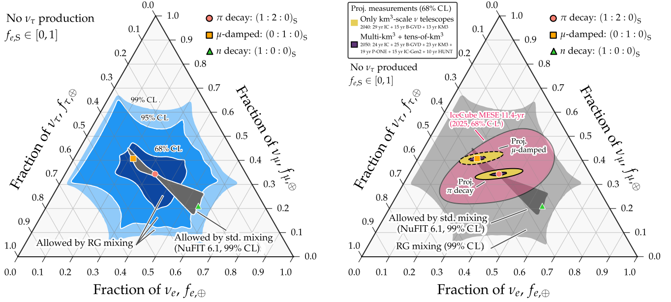
FIG. 4. Standard and RG-modified allowed regions of flavor composition at Earth. The region of flavor composition accessible by standard mixing is obtained by varying the standard mixing parameters within their allowed intervals from NuFIT 6.1 (99% CL) and the flavor composition at the sources f_{e,S} \in [0, 1] (assuming f_{\tau,S} = 0 ). The region accessible by RG-modified mixing is obtained by varying, in addition, the high- Q mixing parameters within their physically allowed regions. Left: the RG-modified allowed regions at 68%, 95%, and 99% CL regions. Right: the 99% CL RG-allowed theoretical space juxtaposed with current and projected experimental sensitivities. Current 68% CL constraints from IceCube (11.4-yr MESE) are shown in gray. Projected 68% CL contours for 2040 (combining IceCube, Baikal-GVD, and KM3NeT) and 2050 (adding IceCube-Gen2, P-ONE, and HUNT) are shown for benchmark pion-decay and muon-damped source scenarios.
