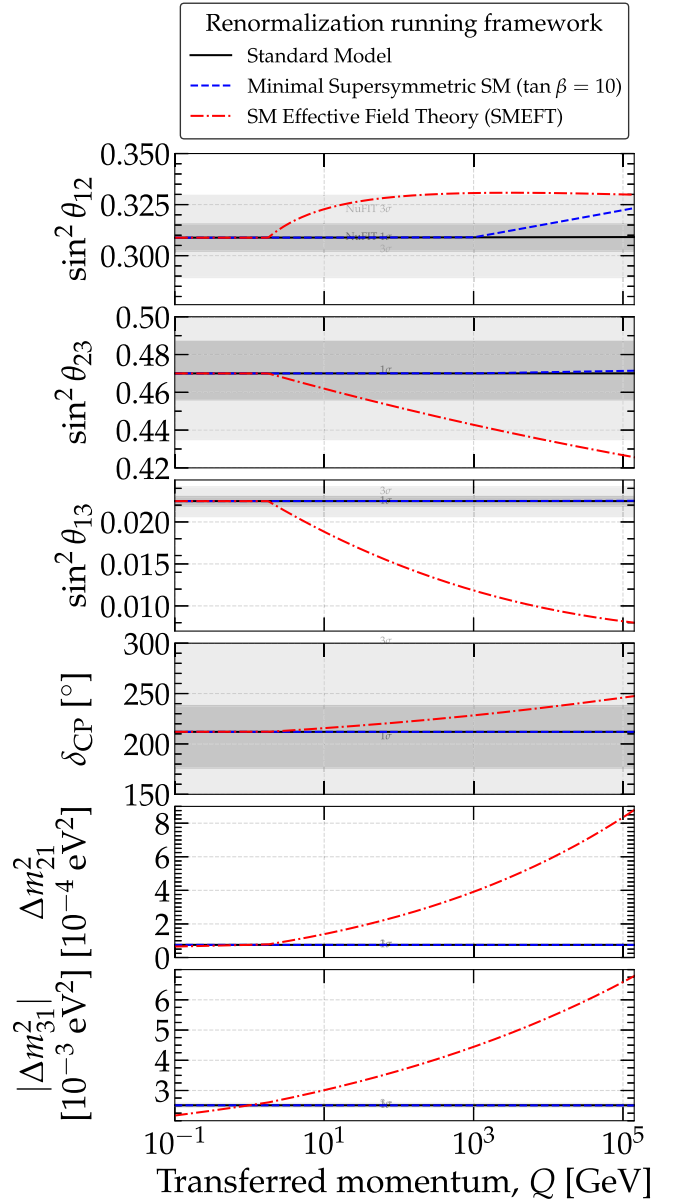
FIG. 5. Renormalization group (RG) evolution of the neutrino mixing parameters. The mixing angles ( \theta_{12} , \theta_{23} , \theta_{13} ) and CP -violation phase ( \delta_{CP} ) evolve as a function of the transferred momentum, Q , depending on the RG scheme chosen. The Standard Model (SM) expectation exhibits negligible running (Sec. IV C). The Minimal Supersymmetric Standard Model (MSSM) with \tan \beta = 10 (Sec. IV D) exhibits limited evolution, while the phenomenological dimension-6 SMEFT exhibits appreciable evolution that makes it possible to place constraints on the RG-modified mixing parameters using high-energy astrophysical neutrino measurements.
