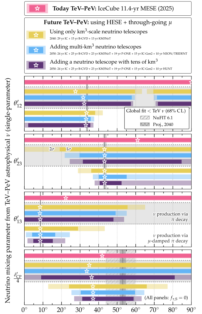
FIG. 11. Constraints on the high- Q neutrino mixing parameters from TeV–PeV astrophysical neutrinos. Present constraints from the 11.4-yr IceCube MESE sample [112] are consistent with three-flavor mixing but cannot constrain individual parameters. Projected measurements from multitelescope observations show sensitivity to \theta_{23} and \theta'_{13} (and \delta'_{CP} under neutrino production via muon-damped pion decay). For comparison, we show current [5] and projected [41] sub-TeV global-fit ranges. These results represent the first rigorous assessment of mixing parameter sensitivity at a representative Q \approx 20 GeV (see Fig. 1).
