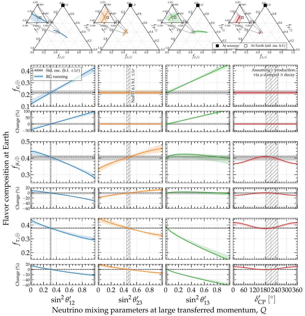
FIG. 18. Flavor composition of high-energy astrophysical neutrinos at Earth as a function of the modified high- Q mixing parameters. Same as Fig. 3 in the main text, but assuming neutrino production via muon-damped pion decay instead, i.e., the flavor composition at the sources is (0, 1, 0)_S . See Appendix C and Sec. III D in the main text for details.
