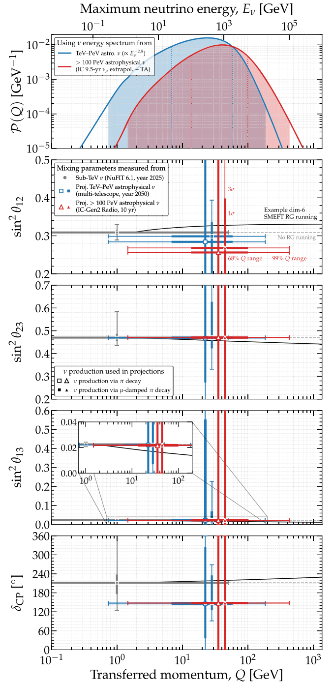
FIG. 1. Evolution of neutrino mixing parameters with transferred momentum, Q . Top panel: probability distribution of Q in the deep inelastic scattering of high-energy (TeV–PeV) and ultrahigh-energy (UHE, > 100 PeV) astrophysical neutrinos on nucleons. The maximum neutrino energy is E_\nu = Q^2/(2m_N) , where m_N \approx 1 GeV is the nucleon mass. Lower panels: variation of the mixing parameters with Q . Present measurements reflect the NuFIT 6.1 global oscillation fit [5]. Projections are for TeV–PeV multidetector observations and UHE detection in the radio array of IceCube-Gen2, assuming astrophysical neutrino production via full or muon-damped pion decay. Evolution under a specific SMEFT RG running scheme is shown for illustration (Sec. IV E).
