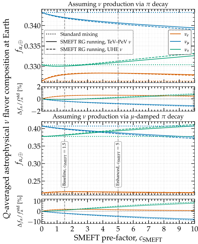
FIG. 8. Example renormalization-group running of the Q -averaged flavor composition at Earth. The evolution of the flavor fractions \tilde{f}_{\alpha,\oplus} [Eq. (34)] and their relative deviations from standard oscillations ( \Delta\tilde{f}_{\alpha,\oplus}/\tilde{f}_{\alpha,\oplus}^{\text{std}} ) are shown as a function of the prefactor c_{\text{SMEFT}} of our example SMEFT scheme (see Sec. IV E). Neutrino production is assumed to occur via full pion decay (top two panels) or muon-damped pion decay (bottom two panels). The Q -averaged SMEFT RG running is shown for two assumed astrophysical neutrino fluxes: a TeV–PeV flux and a UHE flux. Vertical dashed lines highlight our baseline (1.5) and enhanced (5.0) c_{\text{SMEFT}} benchmarks. See Fig. 7 for the explicit running with Q .
