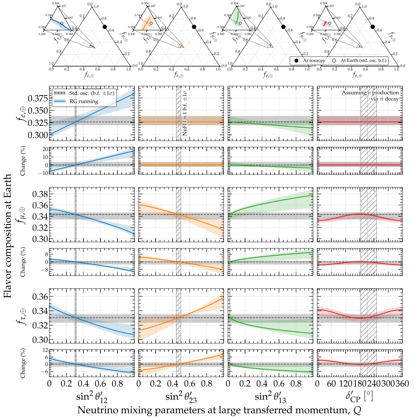
FIG. 3. Flavor composition of high-energy astrophysical neutrinos at Earth as a function of the modified high- Q mixing parameters. Neutrino production is assumed to occur via full pion decay, i.e. , the flavor composition at the sources is (\frac{1}{3}, \frac{2}{3}, 0)_S . The top row shows the trajectory of the flavor composition, (f_e, f_\mu, f_\tau)_\oplus , spanned by varying a single high-energy parameter, compared against the region allowed by standard oscillations. Underneath, rows display f_{e,\oplus} , f_{\mu,\oplus} , and f_{\tau,\oplus} individually, computed via Eq. (4). Columns show independent variations of the high-energy parameters \sin^2 \theta'_{12} , \sin^2 \theta'_{23} , \sin^2 \theta'_{13} , and \delta'_{CP} , with the remaining parameters fixed to their standard low-energy values. We compare these RG-modified ratios against the standard case, where U' = U in Eq. (2). Bands denote 1\sigma uncertainties. Vertical bands indicate NuFIT 6.1 best fit (“b.f.”) and 1\sigma intervals for the varied parameter, assuming normal mass ordering and including Super-Kamiokande data, as in Fig. 2. Subpanels quantify the relative change, (f_{\alpha,\oplus} - f_{\alpha,\oplus}^{\text{std}})/f_{\alpha,\oplus}^{\text{std}} . See Sec. IIID for details and Fig. 18 in Appendix C for the case of neutrino production via muon-damped pion decay.
