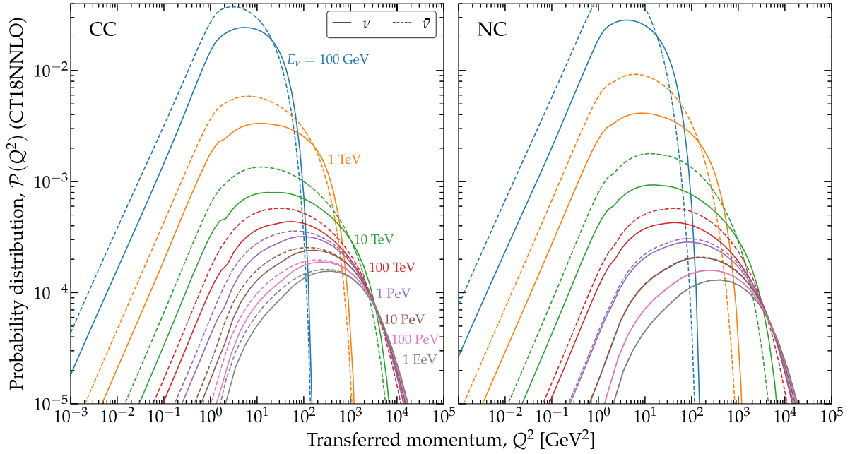
FIG. 15. Distribution of transferred momentum for fixed neutrino energies. The distributions are of Q , the transferred momentum in neutrino-nucleon ( \nu N ) deep inelastic scattering (DIS). They are computed for different representative choices of fixed neutrino energy via Eq. (B4), using the CT18NNLO PDFs [178] to calculate the \nu N DIS cross section. Left: for charged-current (CC) interactions. Right: for neutral-current (NC) interactions.
