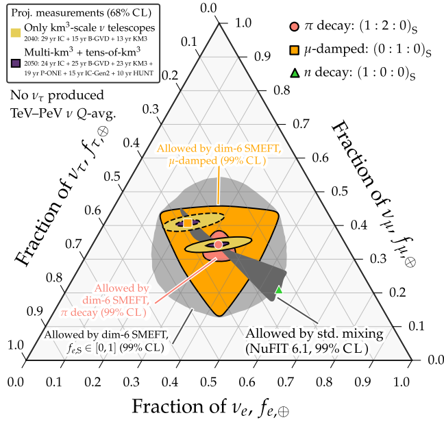
FIG. 10. Effect of the flavor composition at the sources on the SMEFT RG running. Similar to Fig. 9, but now showing three separate scenarios of the flavor composition at the sources (all assuming no \nu_\tau production): varying f_{e,S} \in [0, 1] , fixing f_{e,S} = 1/3 from neutrino production from full pion decay, and fixing f_{e,S} = 0 from neutrino production from muon-damped pion decay. In each case, the RG-regions of flavor composition are generated by varying simultaneously all of the C_{ij} SMEFT coefficients in Eq. (16) (with fixed c_{\text{SMEFT}} = 1 and \Lambda_{\text{SMEFT}} = 1 TeV). Projected 68% CL contours for 2040 (combining IceCube, Baikal-GVD, and KM3NeT) and 2050 (adding IceCube-Gen2, P-ONE, and HUNT) are shown for benchmark pion-decay and muon-damped source scenarios.
