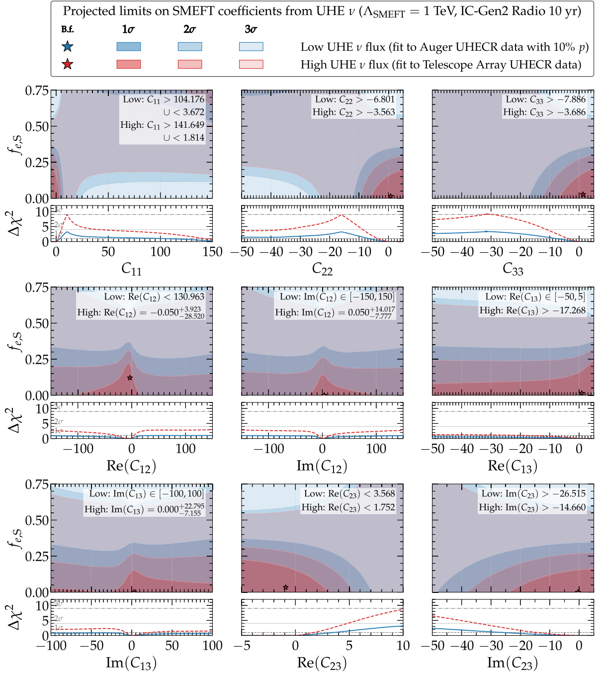
FIG. 14. Projected constraints on dimension-6 SMEFT coefficients using ultrahigh-energy astrophysical neutrinos. Similar to Fig. 13, but for neutrinos of >100 PeV. Limits are derived under the single-operator assumption, where only one SMEFT coefficient is nonzero at a time. Neutrino production is assumed to be via muon-damped pion decay. Flavor-measurement projections are for 10 years of the radio array of IceCube-Gen2, as presented in Ref. [133]. When computing constraints, we assume no \nu_\tau production (i.e., f_{\tau,S} = 0 ). See Sec. VIC for details, Table IV for one-dimensional parameter constraints, and Fig. 13 for constraints from TeV–PeV neutrinos. Constraints from UHE neutrinos are weaker than from TeV–PeV neutrinos because UHE flavor measurements are more uncertain.
