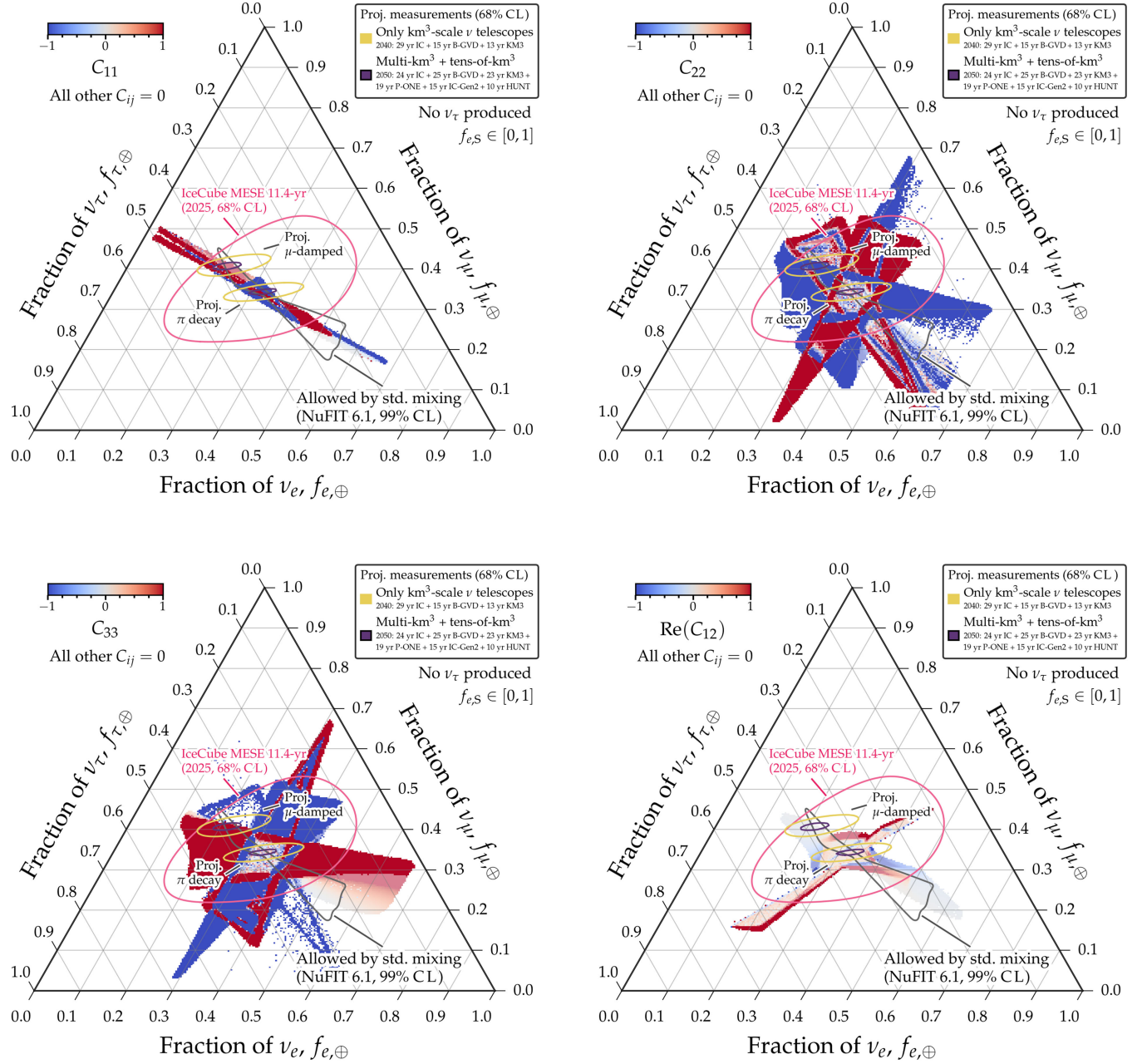
FIG. 24. Dimension-6-SMEFT allowed regions of flavor composition at Earth. The regions are obtained by varying a single SMEFT coefficient at a time, while keeping all other coefficients fixed to zero. This figure should be compared to the all-coefficient Fig. 9 in the main text. See Appendix H for details. Flavor regions for the remaining SMEFT coefficients.
