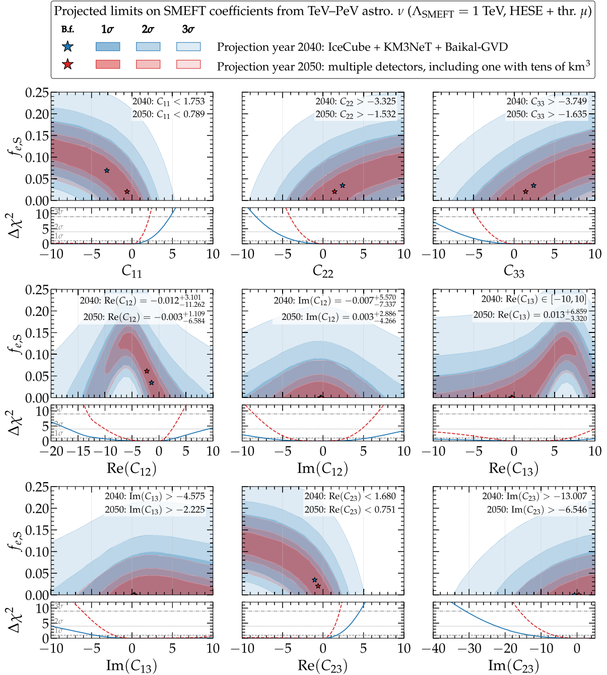
FIG. 13. Projected constraints on dimension-6 SMEFT coefficients using TeV–PeV astrophysical neutrinos. Projections are for 2040, combining only existing neutrino telescopes IceCube, KM3NeT, and Baikal-GVD, and for 2050, combining them with future telescopes P-ONE, IceCube-Gen2, and HUNT. Neutrino production is assumed to be via muon-damped pion decay. Constraints use the neutrino flavor composition inferred from HESE plus through-going muons. For each parameter, the upper panels show the 2D allowed regions at the 1\sigma , 2\sigma , and 3\sigma CL in the plane of the coupling versus the source electron flavor fraction, f_{e,S} . The corresponding 1D profiled \Delta\chi^2 distributions are displayed in the lower panels. The numerical bounds shown in each panel are at 1\sigma CL. The limits assume a reference new physics scale of \Lambda_{\text{SMEFT}} = 1 \text{ TeV} (see the main text to transform to other scales). Limits are derived under the single-operator assumption, where only one SMEFT coefficient is nonzero at a time. When computing constraints, we assume no \nu_\tau production (i.e., f_{\tau,S} = 0 ). See Sec. VIC for details, Table III for one-dimensional parameter constraints, and Fig. 14 for constraints from UHE neutrinos. Meaningful, robust constraints can be placed even by 2040 using the network of existing neutrino telescopes.
