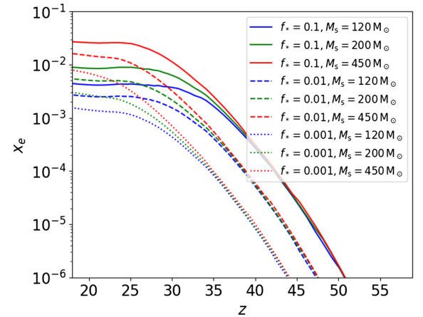
FIG. 8. The ionized fraction as a function of redshift. The line styles and colors correspond to the same parameter values as Fig. 3.
