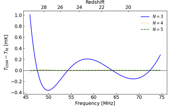
FIG. 9. Temperature residuals between the sky-averaged GSM2008 foreground spectrum and the best-fitting log-polynomial models, T_{\text{GSM}} - T_{\text{fit}} . The solid, dotted, and dashed curves correspond to polynomial orders N = 3, 4 , and 5 , respectively. The models are obtained by fitting \ln T_{\text{GSM}} with an N th-order polynomial in \ln(\nu/\nu_{\text{ref}}) , where \nu_{\text{ref}} is fixed at the center of the fitting band. The lower and upper horizontal axes show the observing frequency and the corresponding redshift, respectively.
