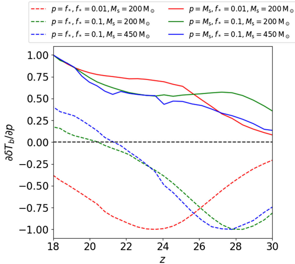
FIG. 12. The parameter derivatives of the global 21-cm brightness temperature as functions of redshift, normalized by its maximum absolute value. The dashed and solid curves show the derivatives with respect to f_* and M_s , respectively. The green and red curves show the derivatives around f_* = 0.1 and f_* = 0.01 , respectively; in all cases M_s = 200M_\odot . The blue curves show those around f_* = 0.1 and M_s = 450M_\odot .
