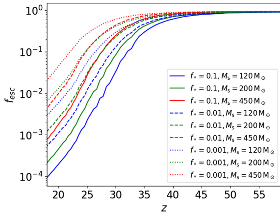
FIG. 5. The halo-mass-averaged escape fraction given by Eq. (9) as a function of redshift. The line styles and colors correspond to the same parameter values as Fig. 3.
