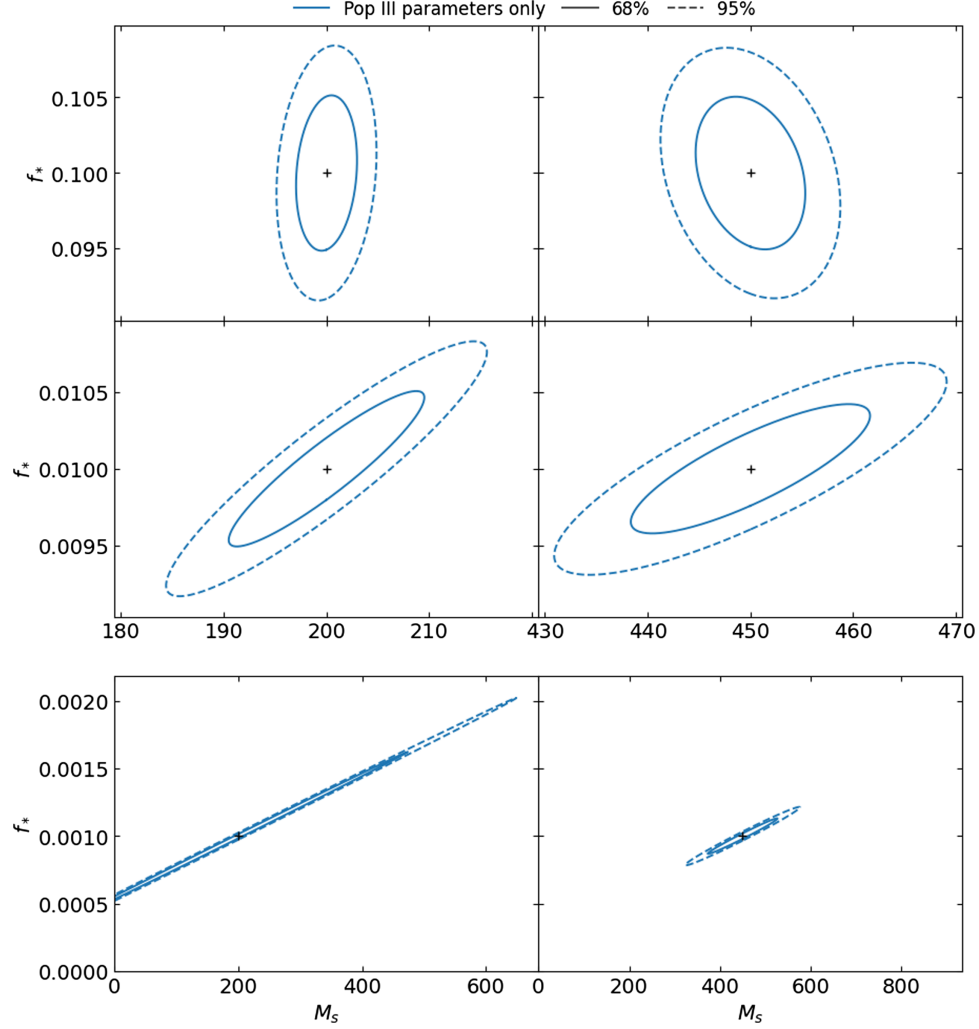
FIG. 10. Forecasted constraints on the Pop III star-formation efficiency, f_* , and stellar mass, M_s , with the foreground parameters fixed at their fiducial values, while the foreground temperature is included in the fiducial sky temperature. The rows correspond to f_* = 0.1 , 0.01, and 0.001 from top to bottom, and the left and right columns correspond to M_s = 200 and 450 M_\odot , respectively. The solid and dashed contours show the 68% and 95% confidence regions, and the black crosses indicate the fiducial parameter values. An integration time of 1000 h is assumed. The upper two rows share the same horizontal scale, whereas a wider M_s range is used for the bottom row.
