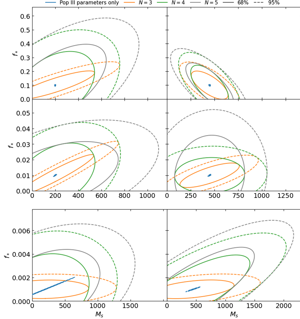
FIG. 11. Forecasted constraints on the Pop III parameters obtained by simultaneously including the foreground coefficients in the Fisher analysis. The foreground is modeled using the log-polynomial form given in Eq. (23), with the reference frequency \nu_{\text{ref}} fixed. The blue contours show the results with the foreground parameters fixed at their fiducial values, while the orange, green, and gray contours show the constraints after marginalizing over the foreground coefficients for N = 3, 4 , and 5 , respectively. These models contain four, five, and six foreground coefficients. The solid and dashed contours denote the 68% and 95% confidence regions. The rows correspond to f_* = 0.1, 0.01 , and 0.001 from top to bottom, and the left and right columns correspond to M_s = 200 and 450 M_\odot , respectively. An integration time of 1000 h is assumed.
