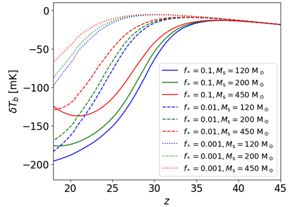
FIG. 3. The global 21-cm brightness temperatures as functions of redshift. The solid, dashed, and dotted lines are cases of f_* = 0.1, 0.01, 0.001 respectively. The red, green, and blue lines are cases of M_s = 450, 200, 120 M_\odot , respectively.
