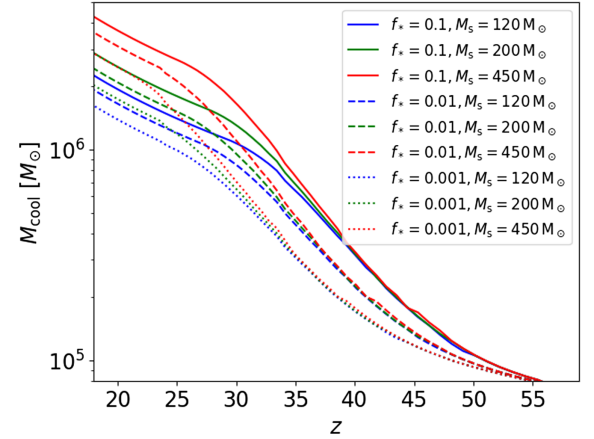
FIG. 7. The minimum halo mass, M_{\text{cool}} , as a function of redshift. The line styles and colors correspond to the same parameter values as Fig. 3.
