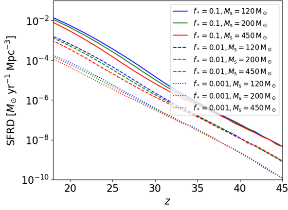
FIG. 4. The star formation rate density as a function of redshift. The line styles and colors correspond to the same parameter values as Fig. 3.
