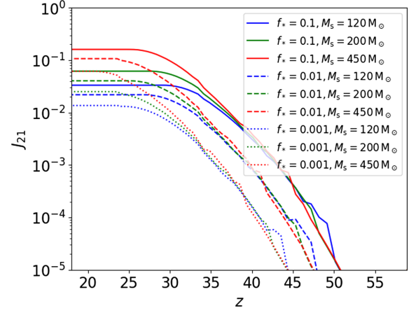
FIG. 6. The averaged LW intensity, J_{\text{LW}}(z) , as a function of redshift. The line styles and colors correspond to the same parameter values as Fig. 3.
