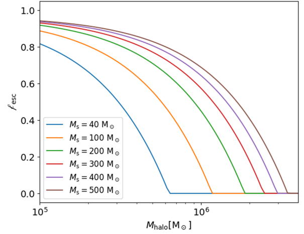
FIG. 1. Escape fraction–halo mass relation. Relationship between the ionizing photon escape fraction, f_{\text{esc}} , and halo mass, M_h , shown for several stellar masses, M_s . f_{\text{esc}} decreases with increasing M_h due to enhanced absorption by hydrogen within more massive haloes, while it increases with increasing M_s as stronger ionizing emission drives faster expansion of the ionized bubble inside the halo.
