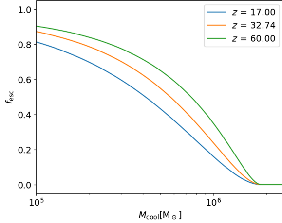
FIG. 2. Halo-mass-averaged escape fraction f_{\text{esc}} as a function of the threshold halo mass for star formation M_{\text{cool}} in the case of M_s = 200M_\odot . The escape fraction f_{\text{esc}} decreases with increasing M_{\text{cool}} because star formation becomes restricted to more massive haloes that individually exhibit smaller escape fractions, f_{\text{esc}} . It declines toward lower redshifts, reflecting the increasing contribution of massive haloes that form preferentially at later times.
