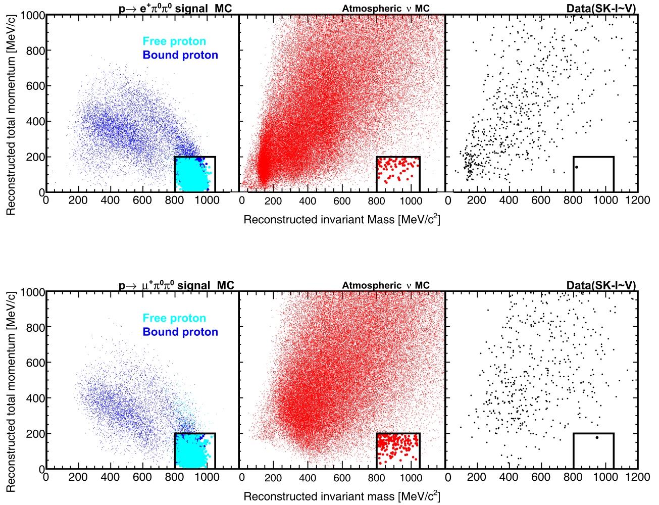
FIG. 3. Reconstructed invariant masses versus total momentum distribution for p \rightarrow e^+ \pi^0 \pi^0 (upper) and p \rightarrow \mu^+ \pi^0 \pi^0 (bottom) after applying all selection criteria except for the reconstructed invariant mass and total momentum cuts in SK-I to SK-V. Left: the signal MC samples. Center: the atm.- \nu background MC samples. Right: the data distributions. The black box in each panel represents the signal region and the markers in the signal region have been enlarged for visibility. In the signal MC samples, the cyan dots represent free protons, and the blue dots represent bound protons.
