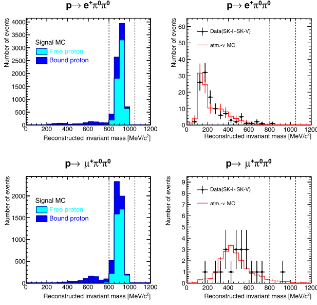
FIG. 1. The reconstructed invariant mass distributions after applying all the event selection criteria except for the reconstructed invariant mass cut, for the signal MC samples (left) and the atm.- \nu background MC samples and the data (right) in SK-I to SK-V, for p \rightarrow e^+\pi^0\pi^0 (upper) and p \rightarrow \mu^+\pi^0\pi^0 (bottom). The atm.- \nu background MC samples (red histogram) is scaled to the total live time for each SK phase. In the signal MC samples distribution, free protons are shown in cyan, and bound protons are shown in blue histograms. The signal region is defined between the two vertical dashed lines.
