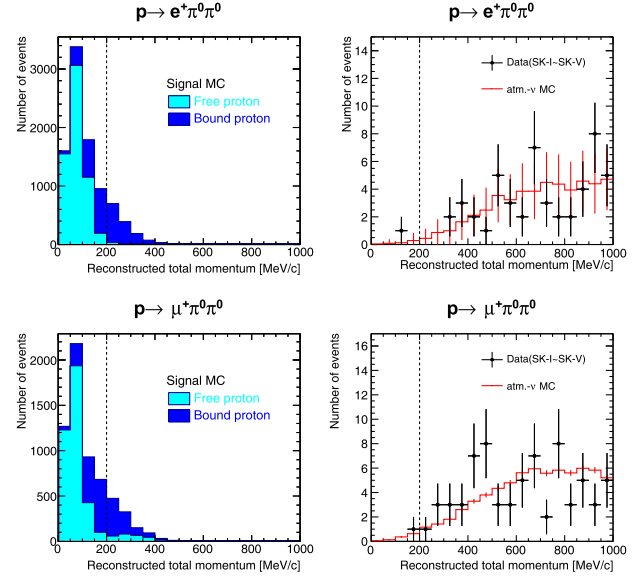
FIG. 2. The total momentum distribution after applying all event selection criteria except for the total momentum cut. Left: the signal MC samples. Right: the atm.- \nu background MC samples (red histogram) and the data in SK-I to SK-V (black crosses) for p \rightarrow e^+\pi^0\pi^0 (upper) and p \rightarrow \mu^+\pi^0\pi^0 (bottom). In the signal MC samples distribution, the cyan histogram represents free protons and the blue histogram represents bound protons. The atm.- \nu background MC samples (red histogram) is scaled to the total live time for each SK phase. The signal region is defined as to the left of the vertical dashed line.
