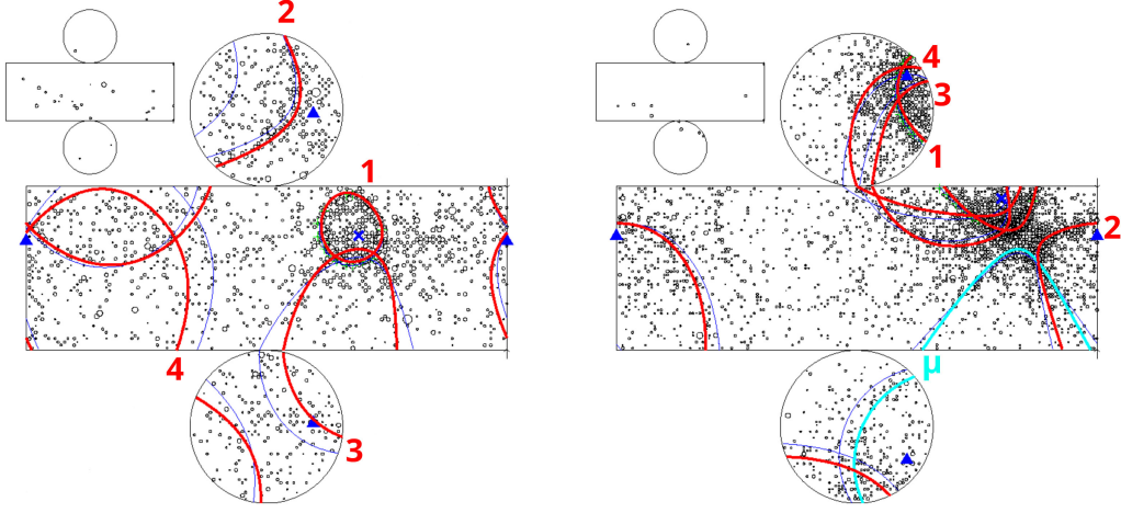
FIG. 5. Event displays for data candidates of p \rightarrow e^+ \pi^0 \pi^0 in SK-II (left) and p \rightarrow \mu^+ \pi^0 \pi^0 in SK-IV (right). These show expanded views of the vertical cylindrical SK tanks, with the ID (center) and OD (left top). Each open circle represents a hit PMT, with its diameter proportional to the detected photoelectrons. The blue filled triangles in ID mark the reconstructed vertex. The solid rings indicate reconstructed ring edges. The red reconstructed rings represent showering particle ( e -like), while the cyan reconstructed ring represents a nonshowering particle ( \mu -like). The numbering of the red rings corresponds to the reconstructed rings described in Sec. V.
