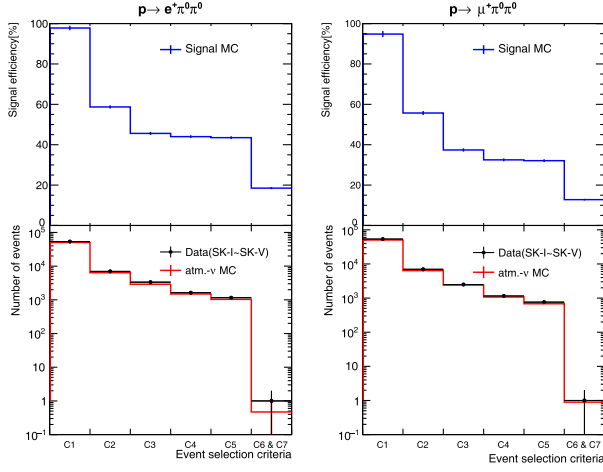
FIG. 4. The event reductions along the event selections for signal MC events (blue), the atm.- \nu background MC events (red), and data (black points) for p \rightarrow e^+\pi^0\pi^0 (left) and p \rightarrow \mu^+\pi^0\pi^0 (right). Shown are the signal efficiency, weighted by the live time, and the total number of background events from SK-I to SK-V. For the background, the MC for each SK phase was scaled to that phase's live time. The event selection criteria are defined in Sec. IV. The statistical errors on each bin are shown.
