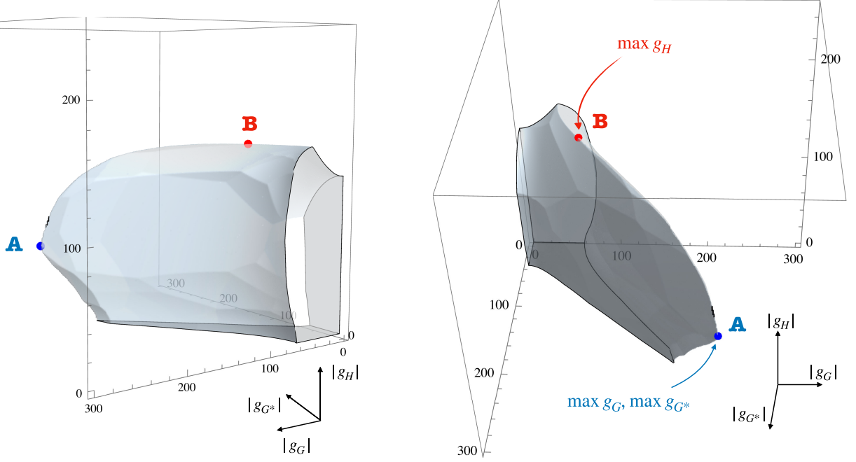
FIG. 4. The glue-hedron . Glueball couplings for SU(3) YM must be contained inside this 3D space. The black lines denote the boundaries of the glue-hedron on the planes where one of the couplings is zero.
