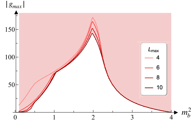
FIG. 3. Bound on the maximum residue |g_{\max}| at the spin-2 bound state of mass m_b^2 . The red region is rigorously excluded.
