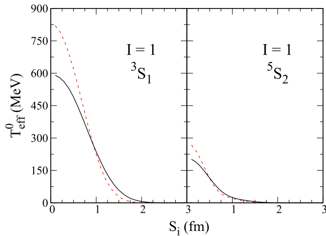
FIG. 7. Kinetic-energy contribution to the adiabatic interaction for the S -wave N\Delta system (isospin I = 1 ) as a function of the generator coordinate S_i in model II. Notations are the same as in Fig. 1.
