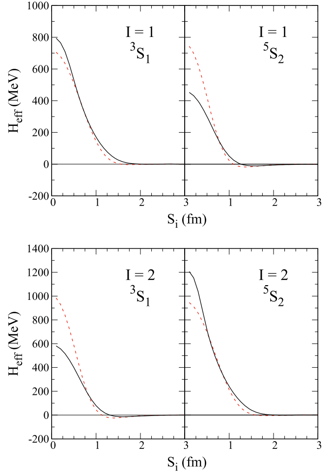
FIG. 10. Total Hamiltonian-induced adiabatic interactions for the S -wave N\Delta systems with I = 1 (upper panel) and I = 2 (lower panel) in model II. Notations are the same as in Fig. 1.
