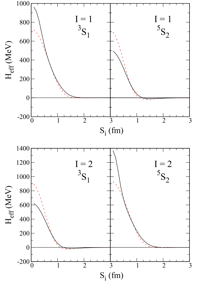
FIG. 4. Total Hamiltonian-induced adiabatic interactions for the S -wave N\Delta systems with I = 1 (upper panel) and I = 2 (lower panel) in model I. Notations are the same as in Fig. 1.
