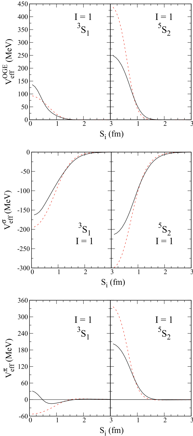
FIG. 9. Contributions from the OGE potential and from \sigma - and \pi -meson exchanges to the adiabatic interaction for the S -wave N\Delta system ( I = 1 ) in model II. Notations are the same as in Fig. 1.
