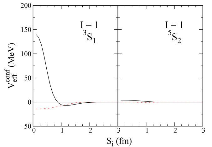
FIG. 8. Confinement potential contribution to the adiabatic interaction for the S -wave N\Delta system ( I = 1 ) in model II. Notations are the same as in Fig. 1.
