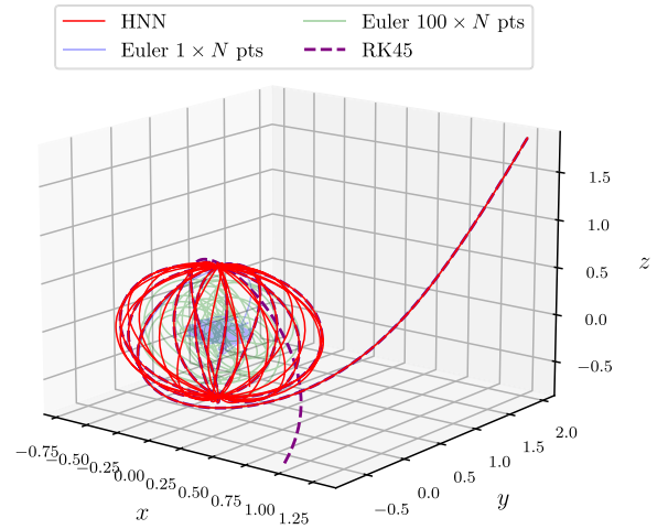
FIG. 34. Geodesics in the 3D Cartesian space for different methods in the nonplanar geometry.
