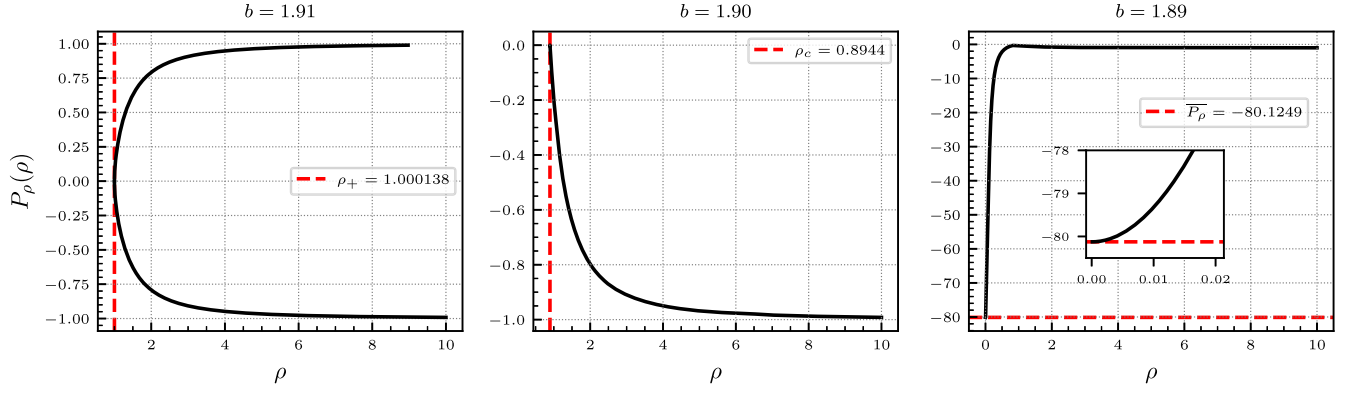
FIG. 36. Exact functions P_\rho(\rho) for the planar geometry. Left panel: overcritical case with b = 1.91 . The vertical dashed line represents \rho_+ = 1.000138 , which is the largest root of the radicand in Eq. (3.17). Central panel: critical case with b = b_c = 1.9 . The vertical dashed line is the critical radius \rho_c = 0.8944 , obtained from Eq. (3.19). Right panel: subcritical case with b = 1.89 . The horizontal dashed line represents \overline{P}_\rho \equiv P_\rho(0) = -80.1249 , computed from Eq. (C7). The small frame is a zoomed-in view of the region \rho \in [0, 0.02] and shows that P_\rho(\rho) has a vanishing derivative for \rho = 0 .
