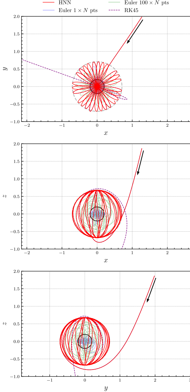
FIG. 33. Geodesics in the nonplanar case for different methods, projected onto the x - y , x - z , and y - z Cartesian planes, respectively, from top to bottom. The solid black line represents the fuzzball surface. The dashed light-gray lines represent the circumference and ellipses defined in Eqs. (5.10)–(5.12). The black arrow indicates the incoming direction of the particle.
