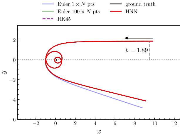
FIG. 23. Geodesics in the Cartesian plane obtained from different methods in the subcritical case with b = 1.89 and by applying the time-splitting approach. The ground truth is represented by the solid black line, while the small circle at the center (0,0) has radius a_f , and it represents the fuzzball. The black arrow indicates the incoming direction of the particle.
