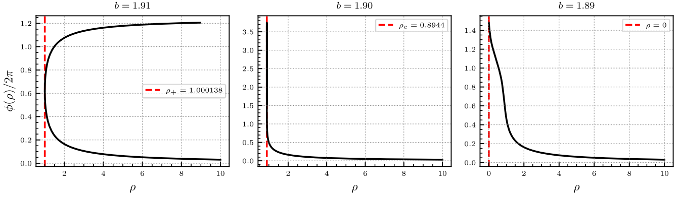
FIG. 35. Exact functions \phi(\rho)/2\pi for the planar geometry. Left panel: overcritical case with b = 1.91 . The vertical dashed line represents \rho_+ = 1.000138 , which is the largest root of the radicand in Eq. (3.17). Central panel: critical case with b = b_c = 1.9 . The vertical dashed line is the critical radius \rho_c = 0.8944 , obtained from Eq. (3.19). Right panel: subcritical case with b = 1.89 . The vertical dashed line is drawn for \rho = 0 , below which the motion has no physical sense.
