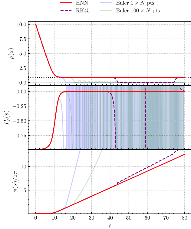
FIG. 15. From top to bottom: \rho(s) , P_\rho(s) , and \phi(s)/2\pi for different methods in the critical case with b = b_c = 1.9 and N = 800 . The horizontal black dotted line in the top panel represents the critical radius \rho_c = 0.8944 , on which the trajectory must settle. The trajectory predicted by the HNN is the only one among the different methods to correctly reproduce this feature.
