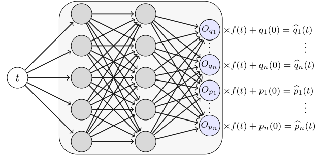
FIG. 2. The neural network architecture consists of one input node for the time t , an arbitrary number of hidden layers, and an output layer with a number of nodes (colored light blue) equal to the number of nontrivial Hamilton equations that constitute the system. The network outputs are multiplied by f(t) = 1 - e^{-t} and added to the initial conditions. Notice that f(0) = 0 is such that the initial conditions are exactly satisfied by the predicted solution.
