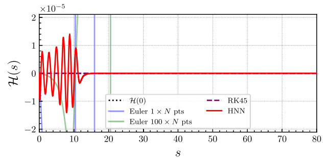
FIG. 14. Energy conservation over time in the critical case with b = b_c = 1.9 and N = 800 for different methods. The conserved value of the energy \mathcal{H}(0) = 0 is represented by the dotted black line.
