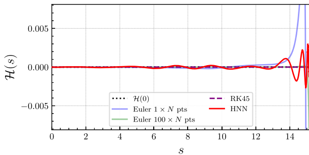
FIG. 26. Energy conservation for the subcritical case with b = 1.89 for the different methods and by following the preconditioning approach. The conserved value of the energy \mathcal{H}(0) = 0 is represented by the dotted black line.
