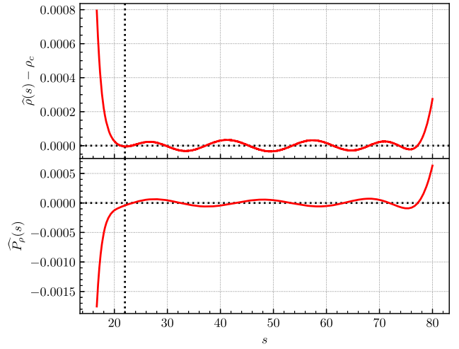
FIG. 16. Stability of the trajectory predicted by the HNN over a long timescale. The vertical dotted line is drawn at s \simeq 22 , the time at which the trajectory approximately reaches the critical circumference. Top panel: difference between \hat{\rho}(s) and \rho_c = 0.8944 . Bottom panel: predicted \widehat{P}_\rho(s) .
