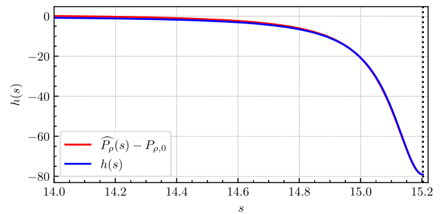
FIG. 24. Result of the fit (blue line) compared to the fitted quantity (red line). In this case, \widehat{P}_\rho(s) is the prediction of the HNN obtained from the time-splitting approach in Sec. IV C 1.
