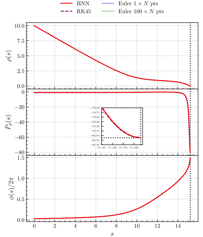
FIG. 27. From top to bottom: \rho(s) , P_\rho(s) , and \phi(s)/2\pi for the different methods in the subcritical case with b = 1.89 and N = 2400 obtained with the preconditioning approach. The vertical dotted line in the three panels represents \bar{s} for the HNN. In the middle panel, we also show a zoomed-in view of the region s \in [15.185, \bar{s}] .
