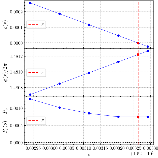
FIG. 19. From top to bottom, the interpolations of \rho(s) , \phi(s)/2\pi , and P_\rho(s) - \bar{P}_\rho at the time \bar{s} . The plot refers to the HNN with the time-splitting approach, for which \bar{s} = 15.2032 (vertical dashed line). In the top and bottom panels, we highlight the value 0 with a horizontal dotted line.
