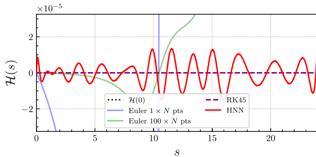
FIG. 7. Energy conservation over time in the overcritical case with b = 1.91 and N = 400 for different methods. The conserved value of the energy \mathcal{H}(0) = 0 is represented by the dotted black line.
