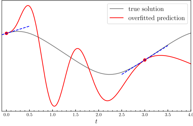
FIG. 3. Demonstrative example of overfitting for a HNN. In this case, the dynamical loss is minimized only for t = 0 and t = 3 (red points), in correspondence with which the predicted solution is accurate, while it rapidly deviates from the true one otherwise.
