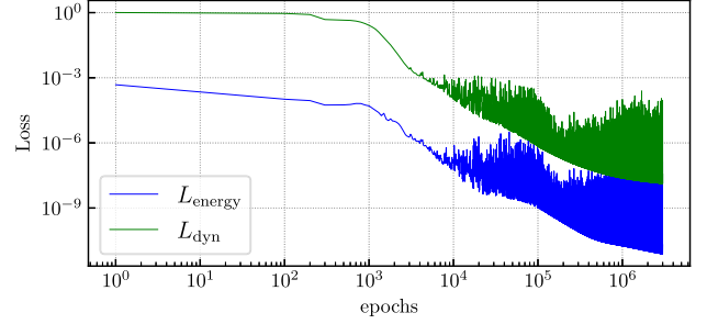
FIG. 13. Loss functions for the critical case with b = b_c = 1.9 . The training has been performed with \lambda = 0.99 , N_{\text{neurons}} = 48 , two hidden layers, and \tanh(x) as the activation function.
