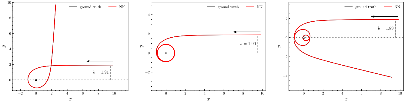
FIG. 39. Comparison between the geodesic predicted by the NN and the ground truth in the Cartesian plane. From left to right: overcritical case with b = 1.91 , critical case with b = b_c = 1.9 , and subcritical case with b = 1.89 . The small black circle has radius a_f = 0.1 , and it represents the fuzzball.
