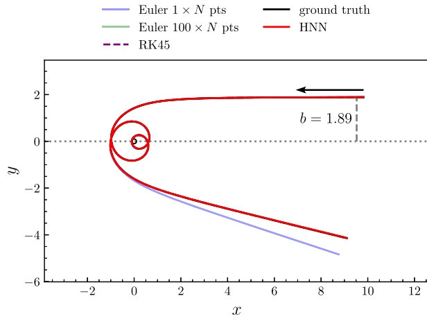
FIG. 29. Geodesics in the Cartesian plane obtained from different methods in the subcritical case with b = 1.89 and by applying the preconditioning approach. The ground truth is represented by the solid black line, while the small circle at the center (0,0) has radius a_f and represents the fuzzball. The black arrow indicates the incoming direction of the particle.
