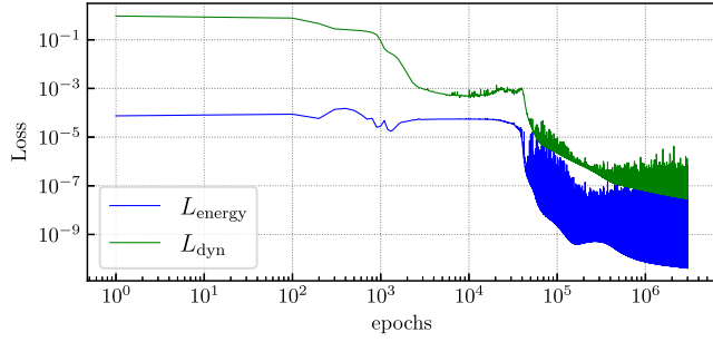
FIG. 6. Loss functions for the overcritical case with b = 1.91 . The training has been performed with \lambda = 0.99 , N_{\text{neurons}} = 32 , two hidden layers, and \tanh(x) as the activation function.
