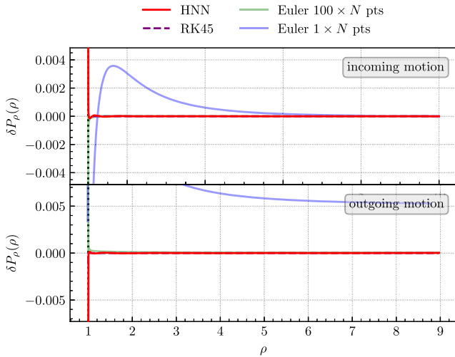
FIG. 10. Error on the variable P_\rho(\rho) for different methods and for the incoming motion (top panel) and the outgoing motion (bottom panel) in the overcritical case with b = 1.91 . The vertical dotted line represents \rho_+ = 1.000138 .
