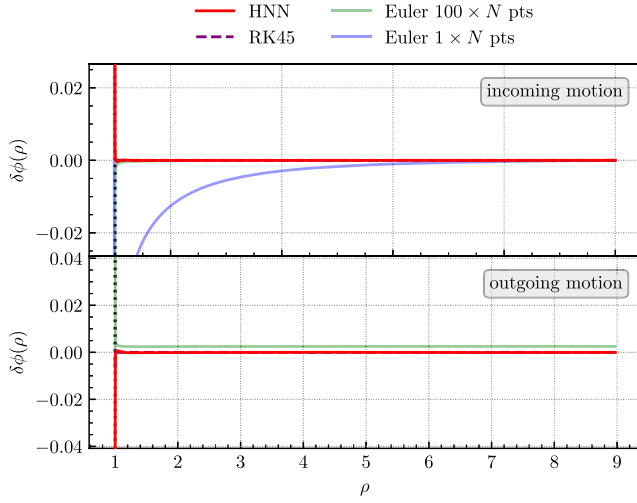
FIG. 9. Error on the function \phi(\rho) for different methods, and for the incoming motion (top panel) and the outgoing motion (bottom panel) in the overcritical case with b = 1.91 . The vertical dotted line represents \rho_+ = 1.000138 .
