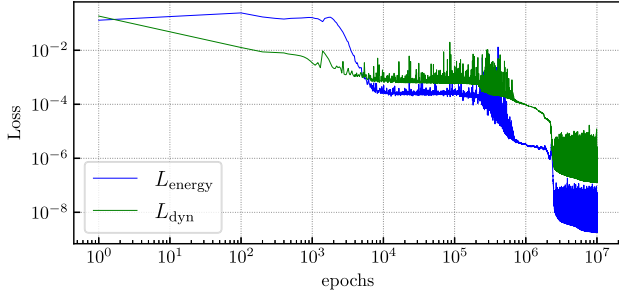
FIG. 30. Loss functions for the nonplanar case.
