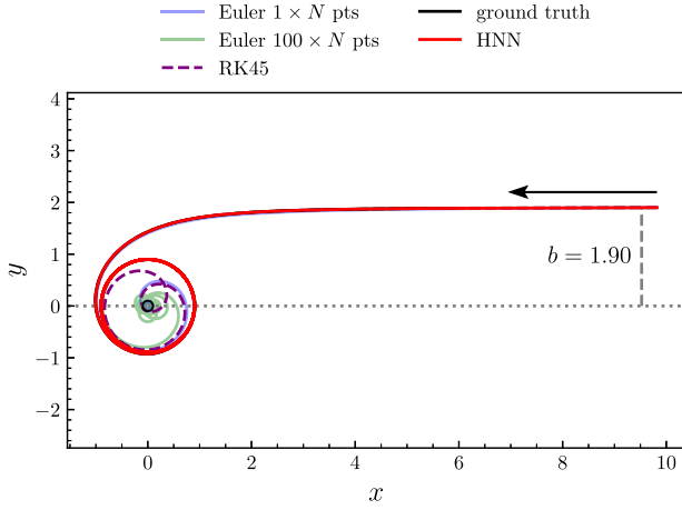
FIG. 17. Geodesics in the Cartesian plane obtained from different methods in the critical case with b = b_c = 1.9 and N = 800 . The ground truth is represented by the solid black line, while the small circle at the center (0,0) has radius a_f and represents the fuzzball. The black arrow indicates the incoming direction of the particle.
