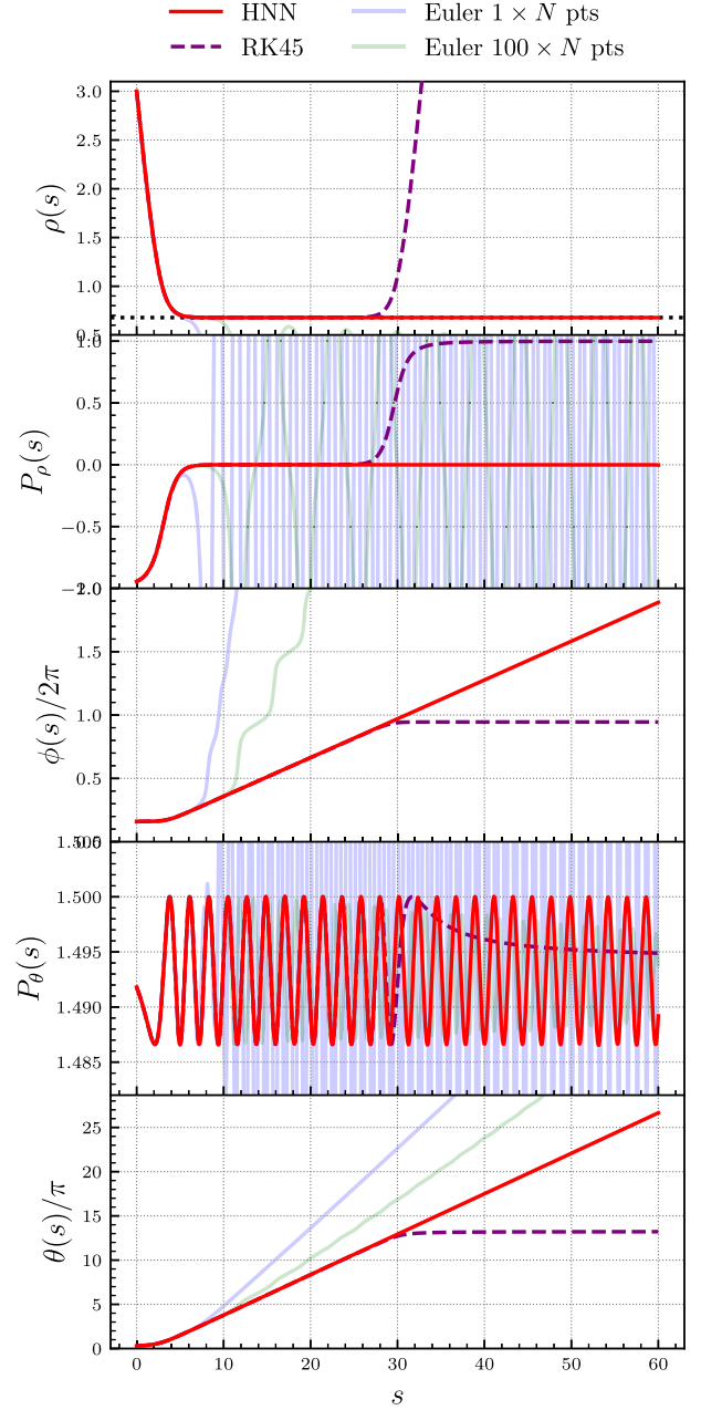
FIG. 32. From top to bottom: \rho(s) , P_\rho(s) , \phi(s)/2\pi , P_\theta(s) , and \theta(s)/\pi for the different methods in the nonplanar case. The horizontal black dotted line in the top panel represents the critical radius \rho_c = 0.6782 , on which the trajectory must settle. The trajectory predicted by the HNN is the only one among the different methods to correctly reproduce this feature.
