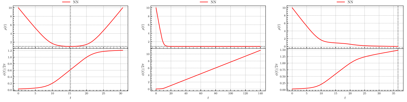
FIG. 38. Predicted \rho(t) (top panels) and \phi(t)/2\pi (bottom panels) corresponding to the equations of motion obtained by exploiting the separability of the geometry. Left panel: overcritical case with b = 1.91 . The vertical dashed line corresponds to t_+ = 15.3157 . The functions for t > t_+ (outgoing motion) are obtained from the reflection of the incoming phase. The horizontal dashed line in the top panel represents \rho_+ = 1.000138 . Central panel: critical case with b = b_c = 1.9 . The horizontal dashed line in the top panel represents \rho_c = 0.8944 . Right panel: subcritical case with b = 1.89 . The vertical dashed line corresponds to the collision time \bar{t} = 36.5417 .
