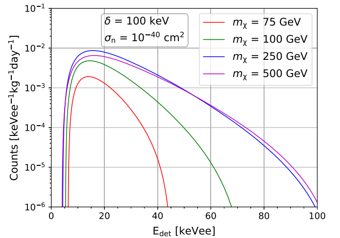
FIG. 3. Expected spectra of the inelastic scattering in the HPGe detector for m_\chi = 75, 100, 250 , and 500 GeV with \delta = 100 keV and \sigma_n = 10^{-40} cm 2 .
