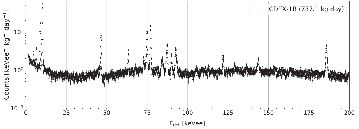
FIG. 4. Background spectrum with error bars based on the 737.1 kg · day dataset of the CDEX-1B experiment [15]. The spectrum is processed using anti-Compton veto and bulk-surface event discrimination [15]. The bin width is 100 eVee and the energy range is 1.5–200 keVee.
