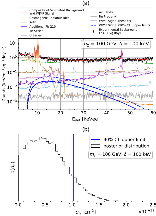
FIG. 7. (a) Background and inelastic WIMP spectra corresponding to the best-fit result and the inelastic WIMP spectrum corresponding to the 90% CL upper limits at m_\chi = 100 GeV, \delta = 100 keV. The black dots with error bars represent the experimental background spectrum. The red solid line represents the composite spectrum of the simulated background and the WIMP signal. The blue solid line represents the WIMP spectrum corresponding to the best-fit result, while the blue dashed line represents the WIMP spectrum corresponding to the 90% CL upper limit. Solid lines in other colors indicate the simulated spectra of each background component. Each peak region defined by the identified peaks in the experimental spectrum is merged into a single composite bin. Consequently, the peaks in the simulated spectra within these regions exhibit a triangular rather than a Gaussian profile in the figure. (b) The posterior distribution of \sigma_n at m_\chi = 100 GeV, \delta = 100 keV. The blue vertical line indicates the 90% CL upper limit on \sigma_n .
