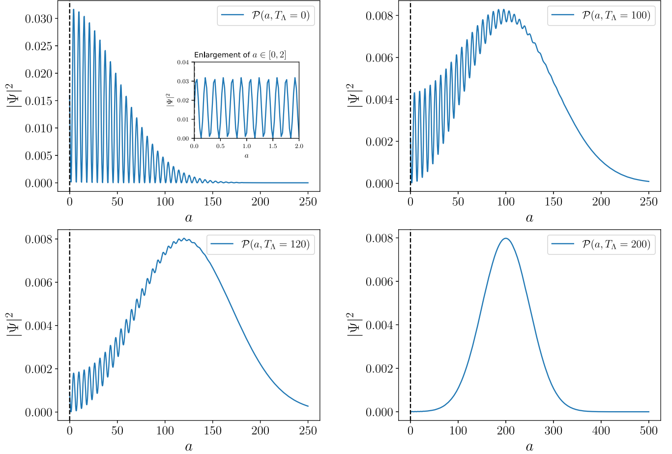
FIG. 2. Probability \mathcal{P}(a, \phi, T_\Lambda) , according to Eq. (76), for times T_\Lambda = 0, 100, 120 , and 200 , with \sigma_T = 0.01 and \phi = 100 . For |T_\Lambda| \sim \sigma_T the probability has many oscillations inside the envelope, but these disappear as |T_\Lambda| increases, as illustrated. We see that, for increasing |T_\Lambda| \gg \sigma_T , the width of the probability decreases; that is, the uncertainty in a decreases.
