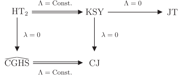
FIG. 1. Diagram illustrating various reductions of the general HT 2 gravity theory. The double arrows indicate the gauge formulations of the KSY and CJ gravity models.
