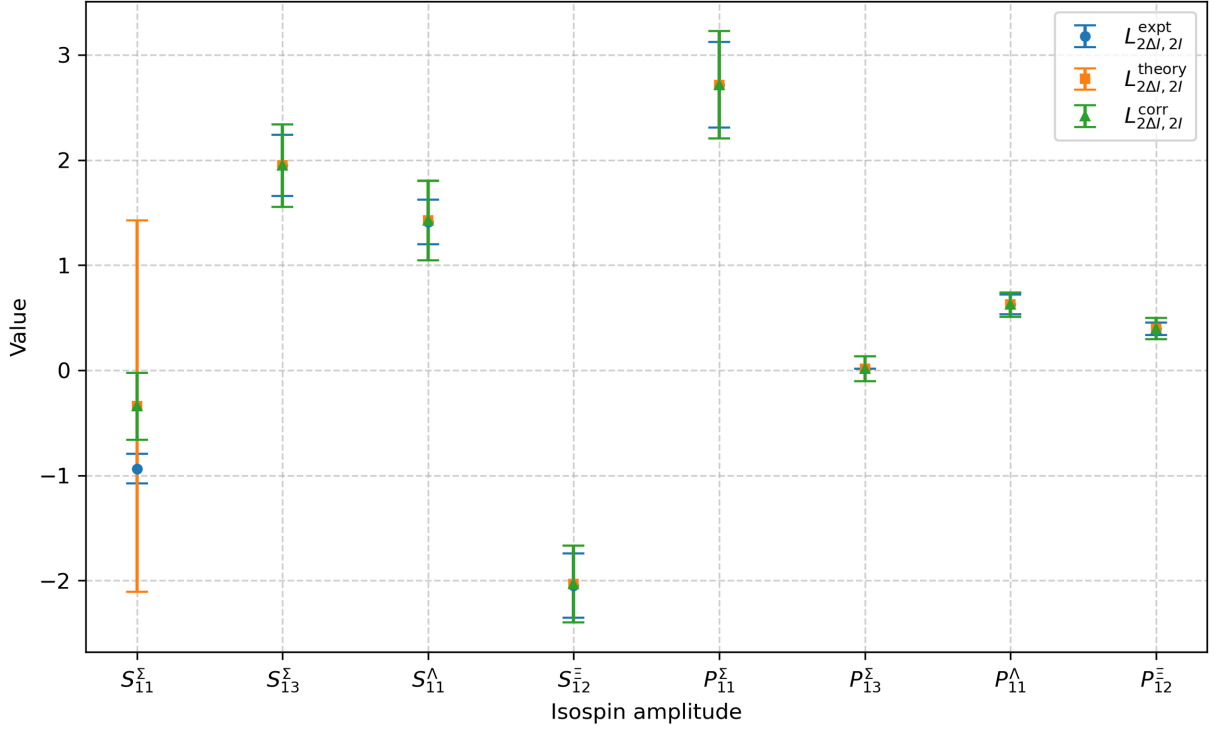
FIG. 7. Results of the combined fit to the s and p waves for the isospin amplitudes L_{2\Delta I, 2I} . See also Fig. 4 and Sec. II C 3 for details about the uncertainties.
