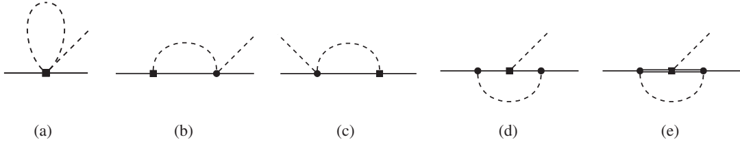
FIG. 2. Loop diagrams contributing to the s -wave amplitude. The types of lines and LECs are the same as in Fig. 1, except for the double line, representing states from the baryon decuplet ( T ), mediated by h_C from (13). Tadpole (a), bubble (b, c), and triangle (d, e) loop diagrams contributing to the s -wave amplitude.
