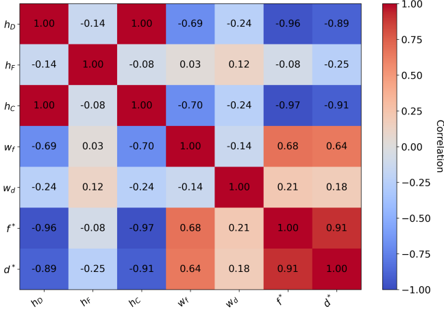
FIG. 5. Correlation matrix for the combined fit to s and p waves including tree-level diagrams with resonances.
