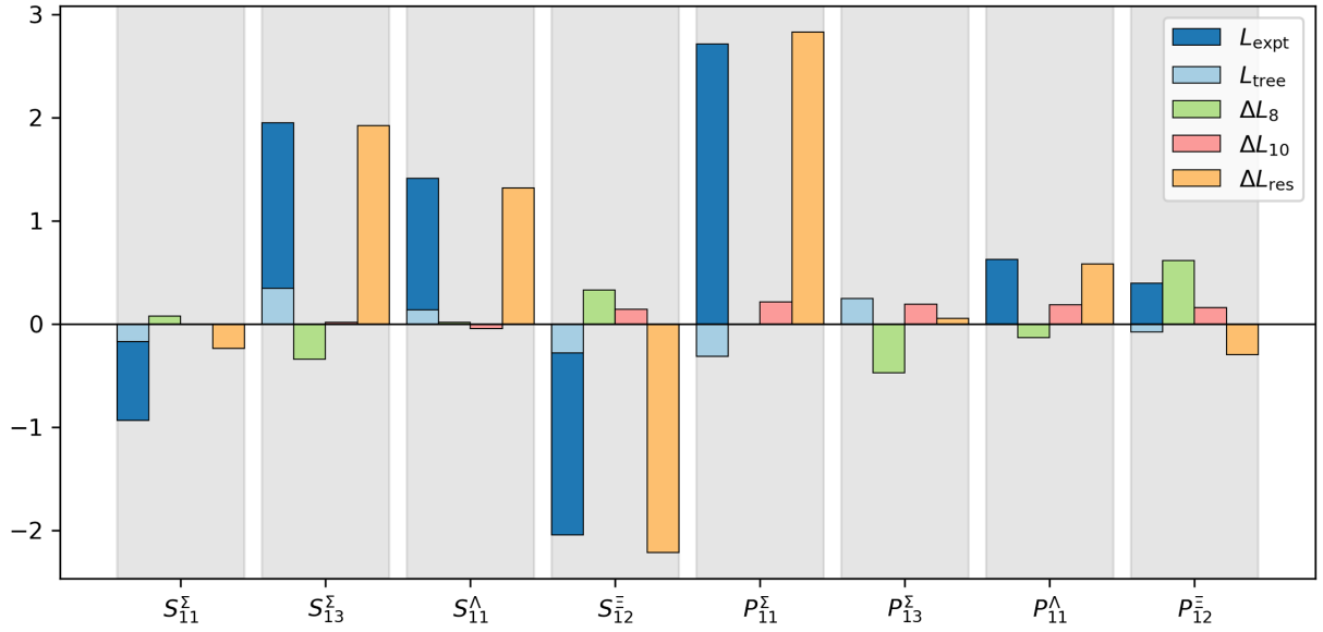
FIG. 8. Size comparison of L_{\text{expt}} to the various LO and NLO contributions to the isospin amplitudes, corresponding to the values in the top half of Table VII.
