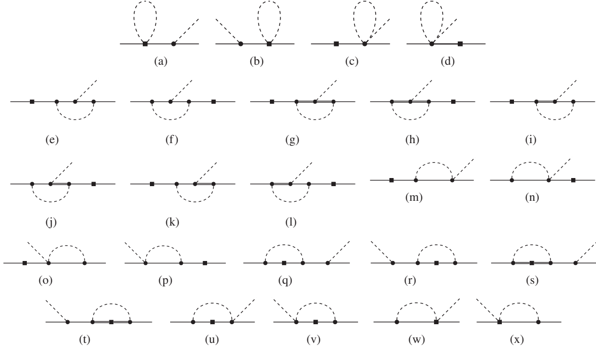
FIG. 3. Loop diagrams that contribute to the p -wave amplitude. The types of lines are the same as in Figs. 1 and 2. Tadpole (a–d), bubble (m–p, w, x), and triangle (e–l, q–v) loop diagrams contributing to the p -wave amplitude.
