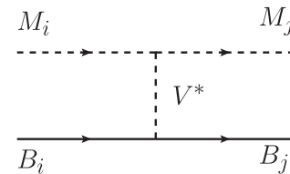
FIG. 1. The t-channel of the meson-baryon interaction in the LHGA.
