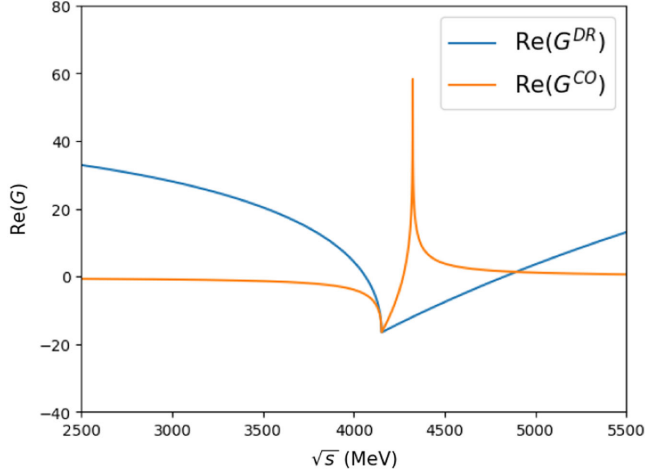
FIG. 3. Typical behavior of the real part of the loop function in the dimensional (blue line) and cutoff (orange line) regularization schemes.
