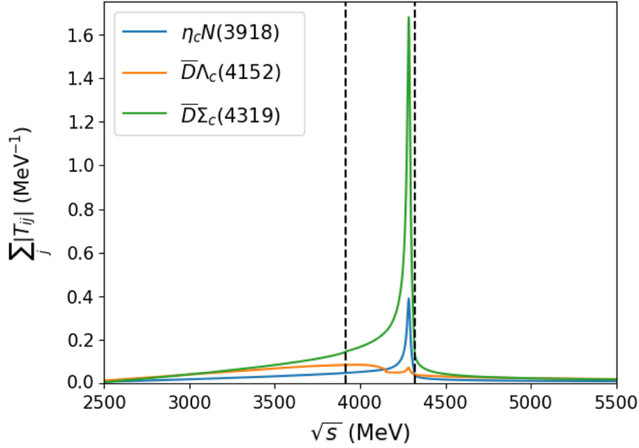
FIG. 4. From left to right, the panels illustrate the scattering amplitude obtained with G^{\text{DR}} , G^{\text{CO}} , and G^{\text{HY}} for the PB interaction in the S = 0, I = 1/2 sector. All three plots share the same y-axis scale and color legend. Each line represents the sum of the moduli of the transition amplitudes to the i th final channel. Vertical black dashed lines indicate the thresholds of the lightest and heaviest channels.
