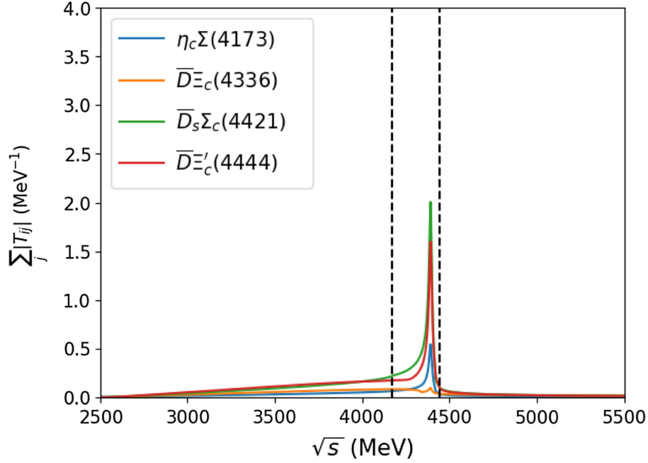
FIG. 9. From left to right, the panels illustrate the scattering amplitude results obtained with G^{\text{DR}} , G^{\text{CO}} , and G^{\text{HY}} for the PB interaction in the S = -1, I = 1 sector. All three plots share the same y-axis scale and color legend. Each line represents the sum of the modulus of the transition amplitudes to the i th final channel. Vertical black dashed lines indicate the thresholds of the lightest and heaviest channels.
