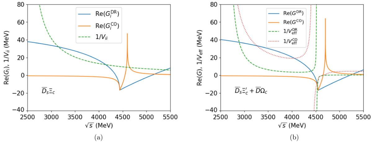
FIG. 13. (a) Real part of the loop function in the DR (blue solid line) and CO (orange solid line) regularization schemes, and the inverse potential in the \bar{D}_s \Xi_c channel. (b) Real part of the loop function in the DR (blue solid line) and CO (orange solid line) schemes for the \bar{D}_s \Xi'_c channel, and inverse \bar{D}_s \Xi'_c - \bar{D} \Omega_c effective potential built with the DR loop (dashed green line) or the CO one (dotted red line).
