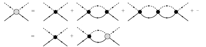
FIG. 2. Diagrammatic representation of the Bethe-Salpeter equation. The gray circle corresponds to the scattering amplitude T , the black circles represent the interaction kernel V and the internal lines correspond to the meson-baryon propagator G .
