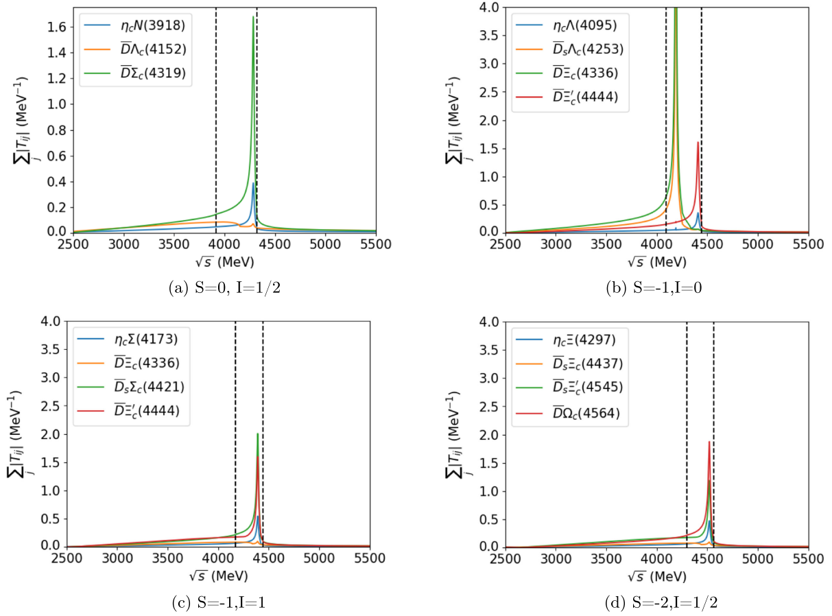
FIG. 15. PB scattering amplitudes for different strange and isospin sectors within the LHGA-WF method. Vertical black dashed lines indicate the thresholds of the lightest and heaviest channels.
