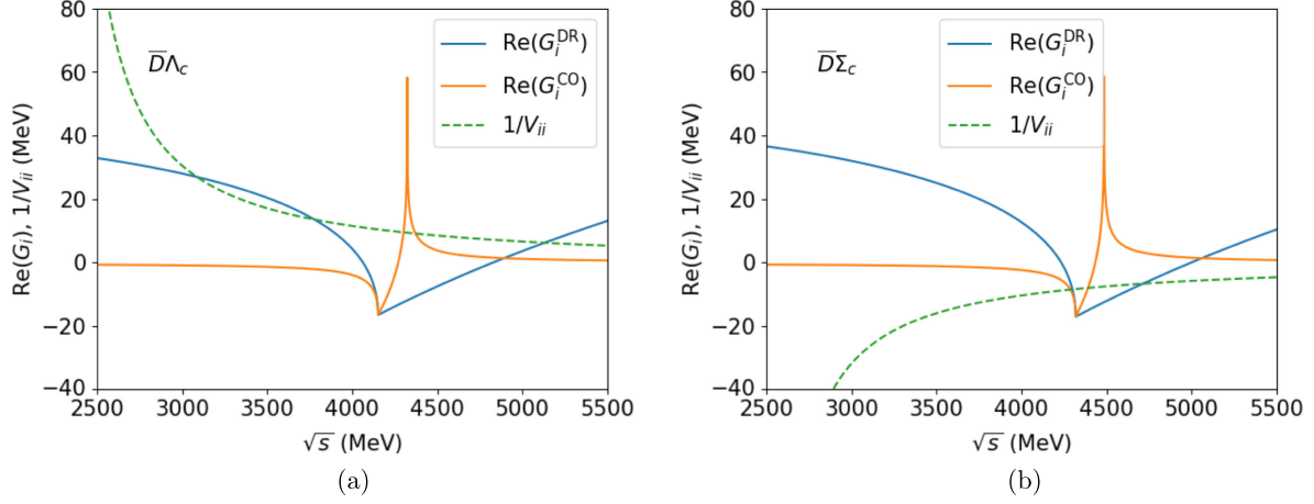
FIG. 5. Real part of the loop function in the dimensional (blue solid line) and cutoff (orange solid line) regularization scheme. The inverse potential 1/V_{ii} is also plotted. The subindex i stands for the corresponding channel: \bar{D}\Lambda_c [panel (a)] and \bar{D}\Sigma_c [panel (b)].
