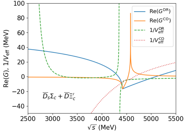
FIG. 11. Effective potential constructed with the channels \bar{D}_s \Sigma_c and \bar{D} \Xi'_c employing the DR loop (dashed green line) or the CO one (dotted red line). The real part of the loop functions for the \bar{D}_s \Sigma_c channel, \text{Re } G^{\text{DR}} (blue line) and \text{Re } G^{\text{CO}} (orange line), are also shown.
