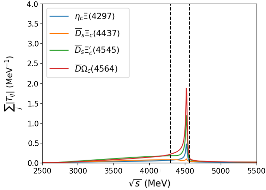
FIG. 12. From left to right, the panels illustrate the scattering amplitude results obtained with G^{\text{DR}} , G^{\text{CO}} , and G^{\text{HY}} for the PB interaction in the S = -2, I = 1/2 sector. All three plots share the same y-axis scale and color legend. Each line represents the sum of the moduli of the transition amplitudes to the i th final channel. Vertical black dashed lines indicate the thresholds of the lightest and heaviest channels.
