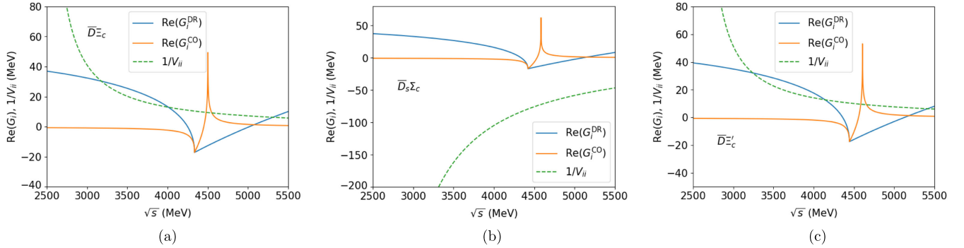
FIG. 10. Real part of the loop function in the dimensional (blue solid line) and cutoff (orange solid line) regularization scheme. The inverse potential 1/V_{ii} is also plotted. The subindex i stands for the corresponding channel: \bar{D} \Xi_c [panel (a)], \bar{D}_s \Sigma_c [panel (b)], and \bar{D} \Xi'_c [panel (c)].
