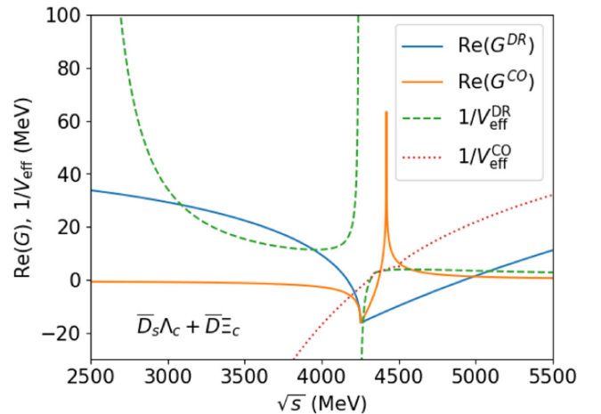
FIG. 8. Effective potential constructed with the channels \bar{D}_s\Lambda_c and \bar{D}\Xi_c employing the DR loop (dashed green line) or the CO one (dotted red line). The real part of the loop functions for the \bar{D}_s\Lambda_c channel, \text{Re } G^{\text{DR}} (blue line) and \text{Re } G^{\text{CO}} (orange line), are also shown.
