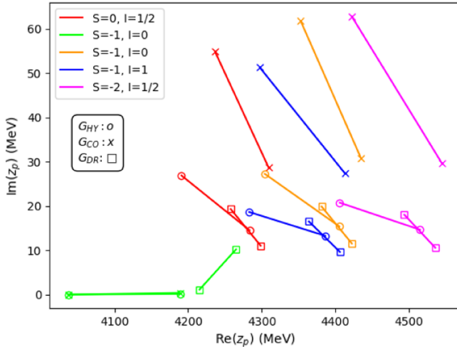
FIG. 14. Results of the pole positions for the PB interaction. The marker is related to the type of regularization employed for the loop function and the color is related to the sector. Results with q_{\text{max}} = 600 and 800 MeV are connected by a straight line of the same color.
