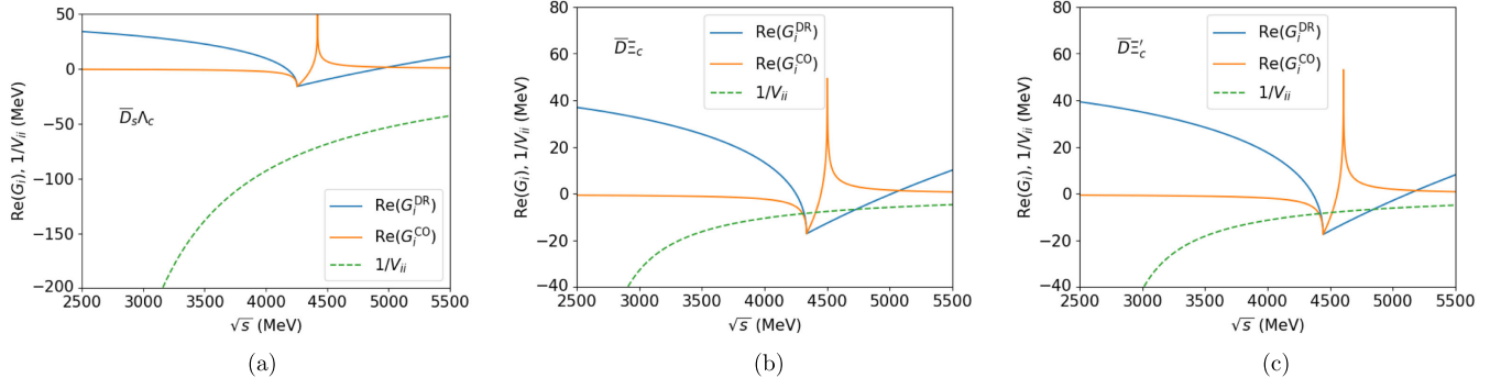
FIG. 7. Real part of the loop function in the dimensional (blue solid line) and cutoff (orange solid line) regularization scheme. The inverse potential 1/V_{ii} is also plotted. The subindex i stands for the corresponding channel: \bar{D}_s\Lambda_c [panel (a)], \bar{D}\Xi_c [panel (b)] and \bar{D}\Xi'_c [panel (c)].
