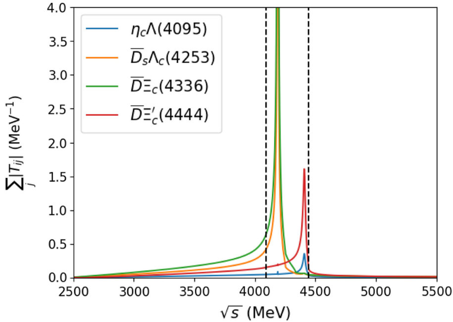
FIG. 6. From left to right, the panels illustrate the scattering amplitude results obtained with G^{\text{DR}} , G^{\text{CO}} , and G^{\text{HY}} for the PB interaction in the S = -1, I = 0 sector. All three plots share the same y-axis scale and color legend. Each line represents the sum of the moduli of the transition amplitudes to the i th final channel. Vertical black dashed lines indicate the thresholds of the lightest and heaviest channels.
