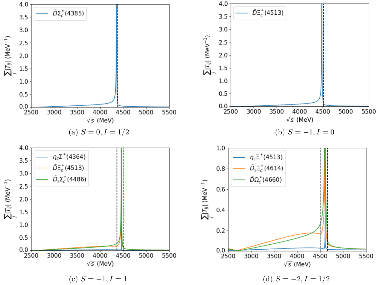
FIG. 16. PB* scattering amplitudes for different strange and isospin sectors within the LHGA-WF method. Vertical black dashed lines indicate the thresholds of the lightest and heaviest channels, or the single channel in cases (a) and (b).
