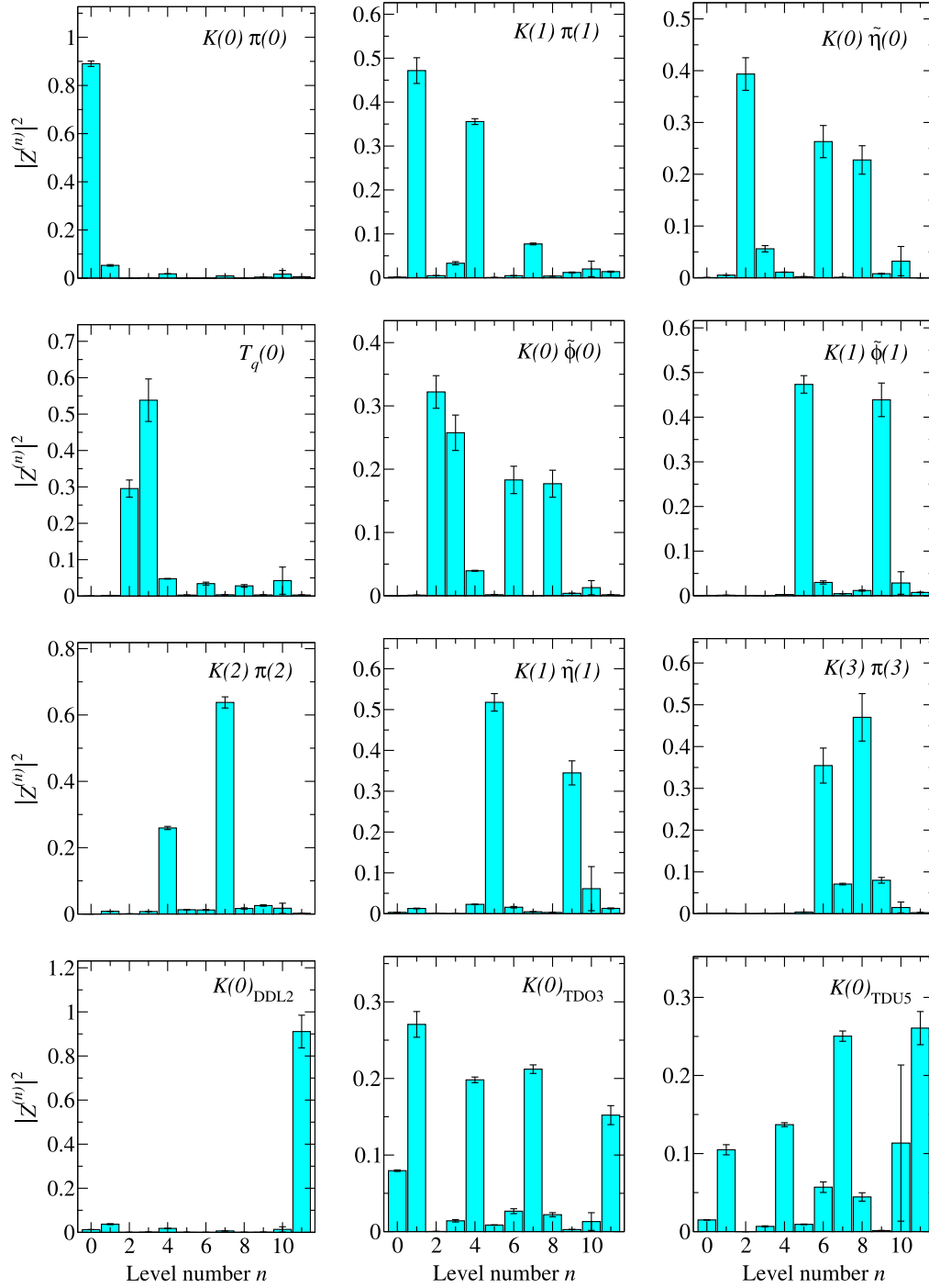
FIG. 5. Overlap factors |Z_j^{(n)}|^2 for the twelve operators used in the correlator matrix corresponding to the isodoublet strange zero-momentum A_{1g} channel. Each plot shows the factors for a single operator, with horizontal axis labeled by n , the index identifying the stationary states. The factors for the tetraquark operator are shown in the left-most plot in the second row from the top. Levels 3 and 2 have significant tetraquark, K\tilde{\eta} , and K\tilde{\phi} content, where \tilde{\eta} means \bar{u}u + \bar{d}d and \tilde{\phi} means \bar{s}s .
