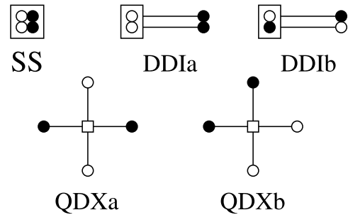
FIG. 1. Our tetraquark operators consist of two gauge-covariantly displaced quarks (open circles) and two displaced antiquarks (solid circles) arranged in the spatial configurations shown above. The boxes indicate locations where color and spin indices are connected. The different spatial configurations we use are single-site operators (SS), doubly displaced operators in an I configuration (DDIa and DDIb), and quadruply displaced operators in a cross configuration (QDXa and QDXb). The letters “a” and “b” in the labels denote the different orderings of displacing the quarks and antiquarks. For each label, there are two color structures, given by Eqs. (12) and (13).
