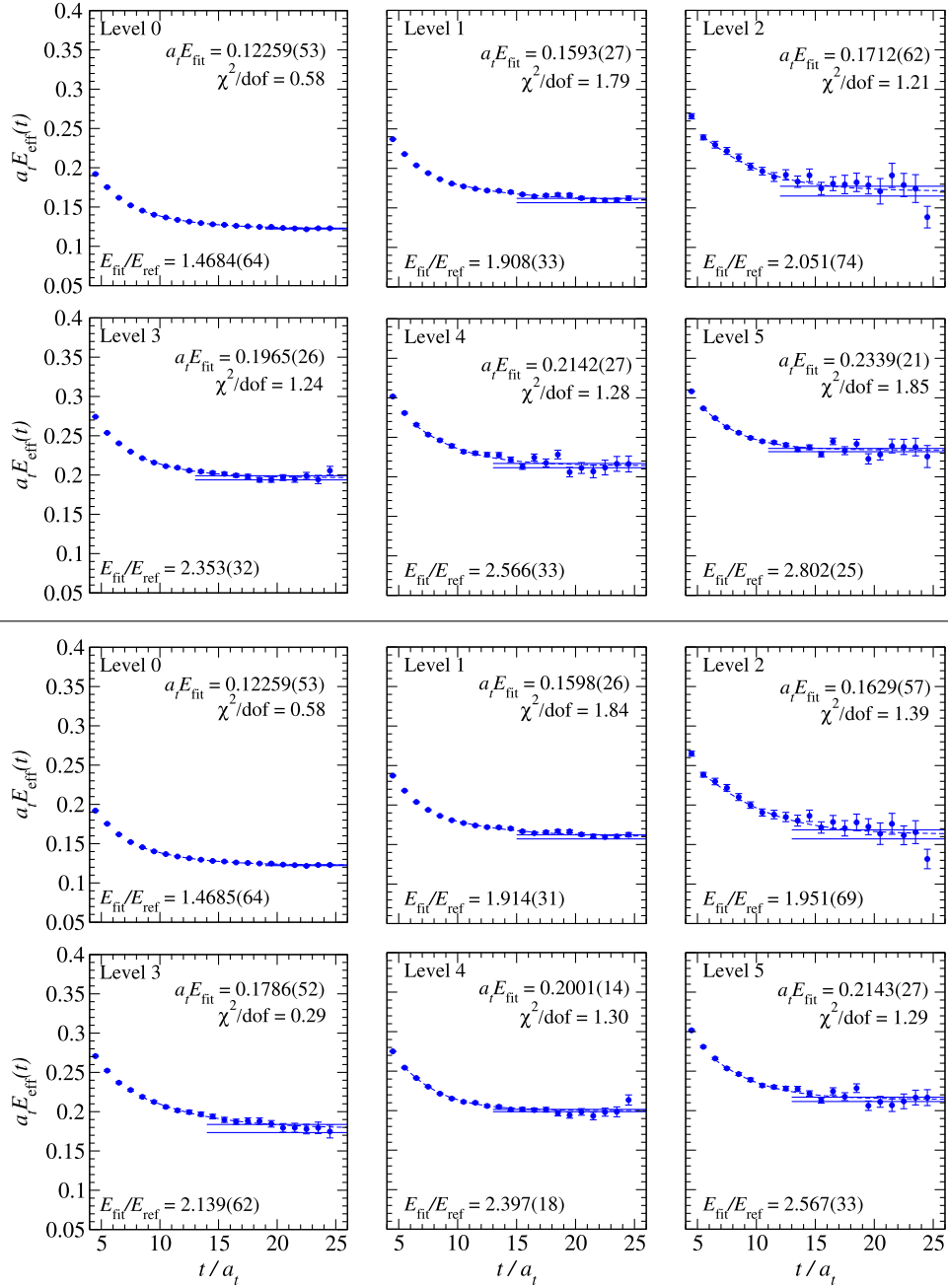
FIG. 3. Effective energies for the lowest six levels in the isodoublet, strangeness 1, zero-momentum, A_{1g} channel. Top two rows: results obtained using only the operators in Tables IV and V, excluding the tetraquark operator. Bottom two rows: results obtained using the operators in Tables IV and V and also including the tetraquark operator in Table VI. Effective energy curves calculated from correlator fits are overlaid, and fit results are shown. Note that level 3 in the bottom row corresponds to the additional level found using the tetraquark operator.
