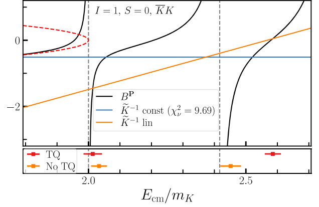
FIG. 13. Study of the Lüscher quantization condition for the I = 1, S = 0, A_{1g} channel with zero total momentum, restricted to relative orbital angular momentum \ell = 0 and the \bar{K}K decay channel. Upper panel: the black curve shows the box matrix B^{(P)} function against center-of-mass energy over kaon mass, with its singularities at the noninteracting energies indicated by vertical dashed lines. Blue and orange curves show the behavior of \tilde{K}^{-1} for constant and linear forms, respectively. Intersections of these curves with the black curves indicate the energies that satisfy the quantization condition. Vertical dashed lines indicate the noninteracting energies, and the red dashed curve is \pm\sqrt{-(k_{\bar{K}K}/m_K)^2} . In the legend, \chi^2_\nu = \chi^2/N_{\text{dof}} . Lower panel: finite-volume energies for the predominantly \bar{K}K states from the lattice QCD computations which include (exclude) the tetraquark operator are shown by the red (orange) points.
