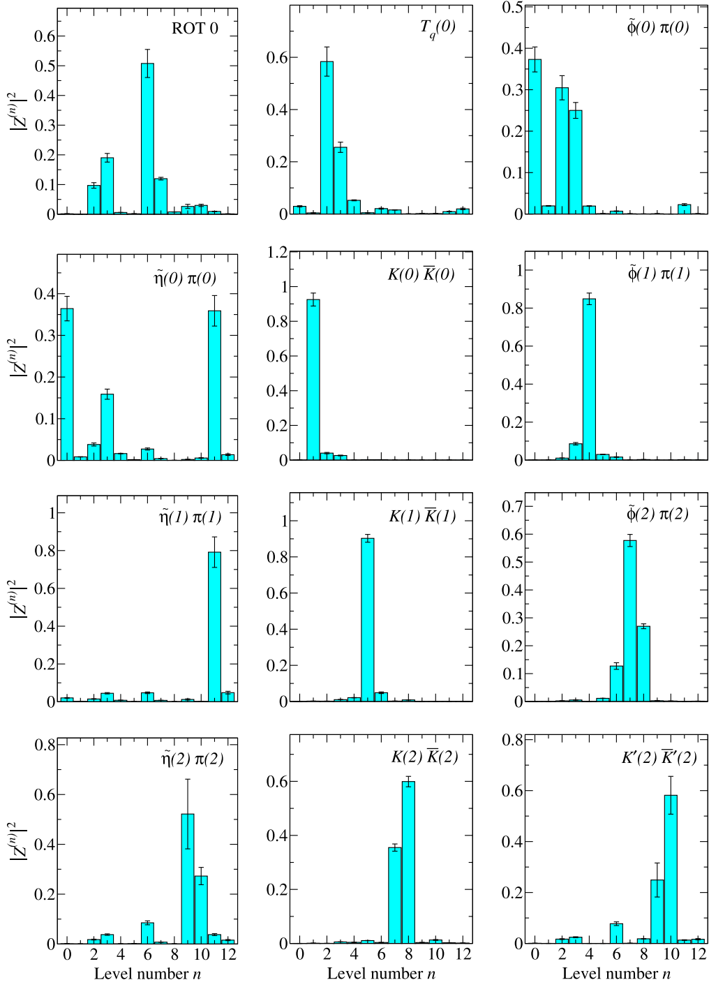
FIG. 8. Overlap factors |Z_j^{(n)}|^2 for twelve of the thirteen operators used in the correlator matrix corresponding to the isotriplet nonstrange zero-momentum A_{1g}^- channel. Each plot shows the factors for a single operator, with horizontal axis labeled by n , the index identifying the stationary states. The factors for the tetraquark operator are shown in the center plot in the top row. Operators labeled by ROT N denote our variationally improved single-hadron operators, as discussed in Sec. III C. K(2) , K'(2) refer to SS0 , SS1 operators, respectively, and similarly for \bar{K}(2) , \bar{K}'(2) (see Table V). The factors for ROT 1 (not shown) are all very small except for level 12.
