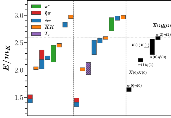
FIG. 9. Left: estimate of isotriplet, strangeness 0, zero-momentum, A_1^- spectrum using operators in Tables IV and V, excluding the tetraquark operator. Center: estimate of the spectrum obtained using operators in Tables IV, V, and VI, which includes the tetraquark operator. Right: two-particle noninteracting energies. Statistical errors of the energy determinations are shown by the vertical extents of the boxes. The horizontal gray line indicates the four-particle \pi\pi\pi\eta threshold (there are no three-particle states in this channel in this energy range). The flavor contents of the 13 basis operators are indicated by colors as shown in the legend. Levels predominantly created by a single operator are indicated by a single color corresponding to the flavor of the operator. Dual colored levels are predominantly created by two of the basis operators with comparable overlap factors. Levels created mostly by a single operator but with significant overlaps from one or more other operators are indicated by a hatched box.
