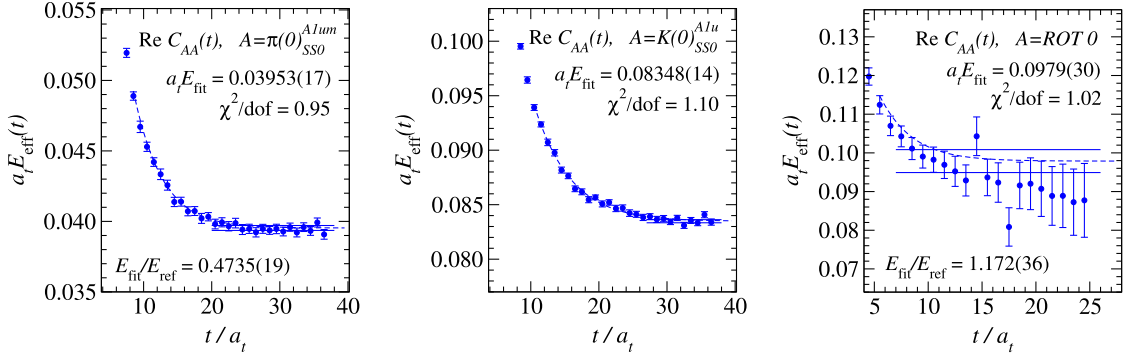
FIG. 2. Effective energies for the at-rest pion (left), kaon (center), and \eta meson (right). The symbols with error bars indicate the Monte Carlo estimates of the effective energy functions, and fitting information is provided by the dashed and solid blue curves, which are explained in the text. Fit results for the dimensionless products of the temporal lattice spacing a_t times the meson masses are shown, along with fit quality \chi^2/N_{\text{dof}} . Fits to the correlators are done using a sum of two exponentials as the fit model. The vertical displacements of the effective energy points for the \eta meson at time separations 14.5 a_t and 17.5 a_t is caused by using an interlace-16 time dilution scheme for the disconnected contributions. Energies were also obtained for these mesons at a variety of different momenta. The operators used to obtain the single-meson masses are discussed in the text in Sec. III A. The reference energy E_{\text{ref}} is taken to be the mass of the kaon.
