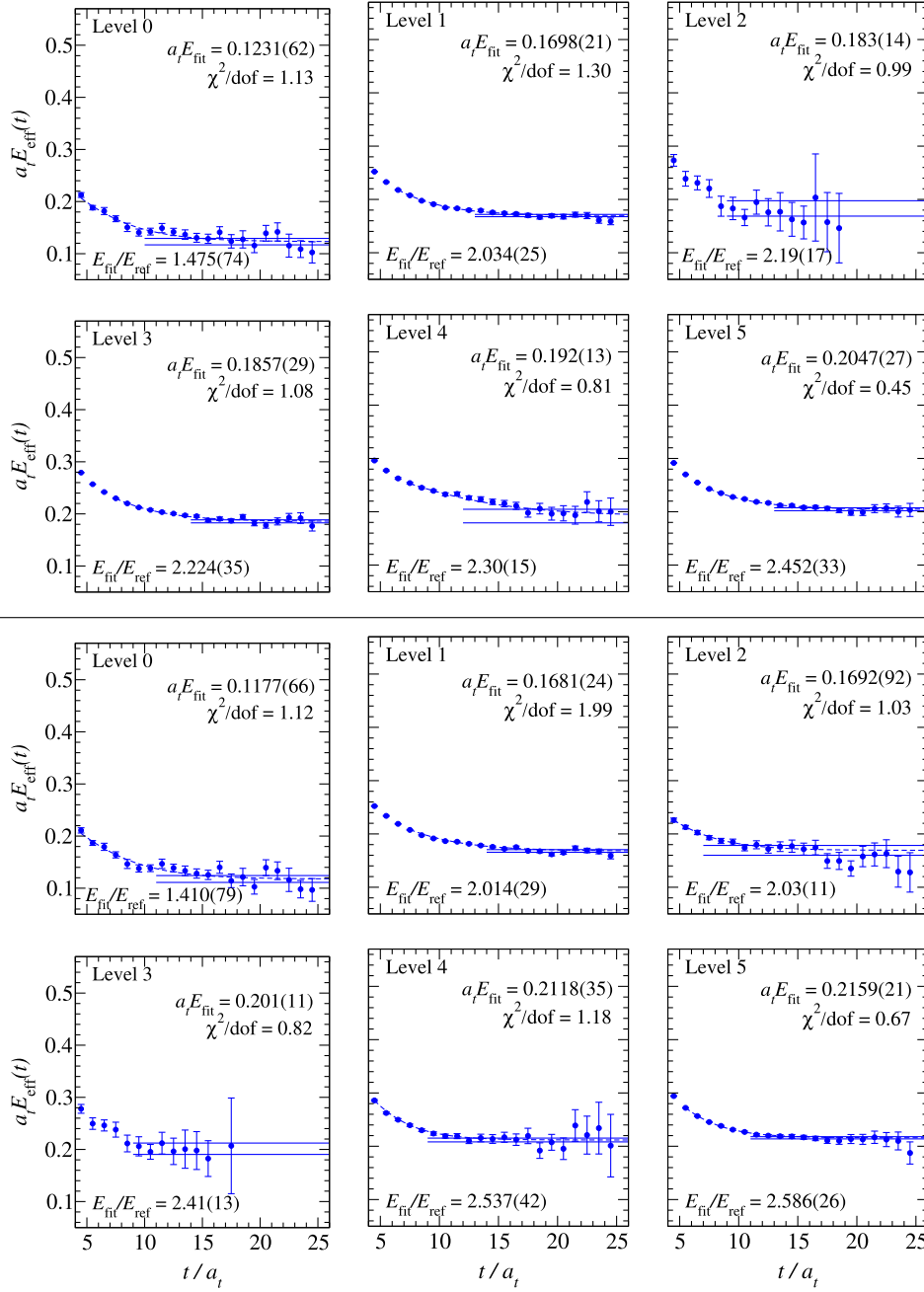
FIG. 7. Effective energies for the lowest six levels in the isotriplet, nonstrange, zero-momentum A_{1g}^- channel. Top two rows: results obtained using only the operators in Tables IV and V, excluding the tetraquark operator. Bottom two rows: results obtained using the operators in Tables IV and V and also including the tetraquark operator in Table VI. Effective energy curves calculated from correlator fits are overlaid, and fit results are shown.
