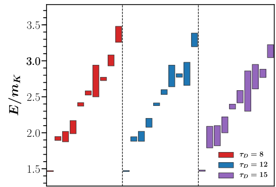
FIG. 4. Determinations of the spectrum in the isodoublet strange zero-momentum A_{1g} channel obtained using three different diagonalization times \tau_D = 8 (left), \tau_D = 12 (center), and \tau_D = 15 (right) for the operator basis given in Tables IV, V, and VI, which includes the tetraquark operator. The metric times \tau_0 are chosen as \tau_D/2 , rounded up. Good agreement is found, but a significant increase in statistical uncertainties is evident for \tau_D = 15 .
