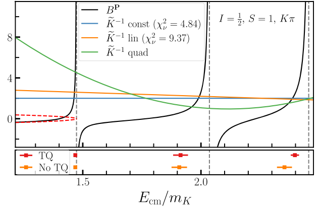
FIG. 10. Study of the Lüscher quantization condition for the I = \frac{1}{2}, S = 1, A_{1g} channel with zero total momentum, restricted to relative orbital angular momentum \ell = 0 and the K\pi decay channel. Upper panel: the black curve shows the box matrix B^{(P)} function against center-of-mass energy over kaon mass, with its singularities at the noninteracting energies indicated by vertical dashed lines. Blue, orange, and green curves show the behavior of \tilde{K}^{-1} for constant, linear, and quadratic forms, respectively. Intersections of these curves with the black curves indicate the energies that satisfy the quantization condition. Vertical dashed lines indicate the noninteracting energies, and the red dashed curve is \pm\sqrt{-(k_{K\pi}/m_K)^2} . In the legend, \chi_\nu^2 = \chi^2/N_{\text{dof}} . Lower panel: finite-volume energies for the predominantly K\pi states from the lattice QCD computations which include (exclude) the tetraquark operator are shown by the red (orange) points.
