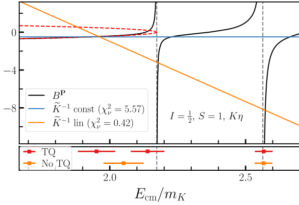
FIG. 11. Study of the Lüscher quantization condition for the I = \frac{1}{2}, S = 1, A_{1g} channel with zero total momentum, restricted to relative orbital angular momentum \ell = 0 and the K\eta decay channel. Upper panel: the black curve shows the box matrix B^{(P)} function against center-of-mass energy over kaon mass, with its singularities at the noninteracting energies indicated by vertical dashed lines. Blue and orange curves show the behavior of \tilde{K}^{-1} for constant and linear forms, respectively. Intersections of these curves with the black curves indicate the energies that satisfy the quantization condition. Vertical dashed lines indicate the noninteracting energies, and the red dashed curve is \pm\sqrt{-(k_{K\pi}/m_K)^2} . In the legend, \chi^2_\nu = \chi^2/N_{\text{dof}} . Lower panel: finite-volume energies for the predominantly K\eta states from the lattice QCD computations which include (exclude) the tetraquark operator are shown by the red (orange) points.
