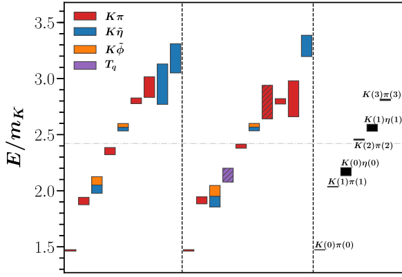
FIG. 6. Left: estimate of isodoublet, strangeness 1, zero-momentum, A_{1g} spectrum using operators in Tables IV and V, excluding the tetraquark operator. Center: estimate of the spectrum obtained using operators in Tables IV, V, and VI, which includes the tetraquark operator. Right: two-particle noninteracting energies. Statistical errors of the energy determinations are shown by the vertical extents of the boxes. The horizontal gray line indicates the four-particle K\pi\pi\pi threshold (there are no three-particle states in this channel in this energy range). The four flavor contents of the twelve basis operators are indicated by colors as shown in the legend. Levels predominantly created by a single operator are indicated by a single color corresponding to the flavor of the operator. Dual colored levels are predominantly created by two of the basis operators with comparable overlap factors. Levels created mostly by a single operator but with significant overlaps from one or more other operators are indicated by a hatched box.
