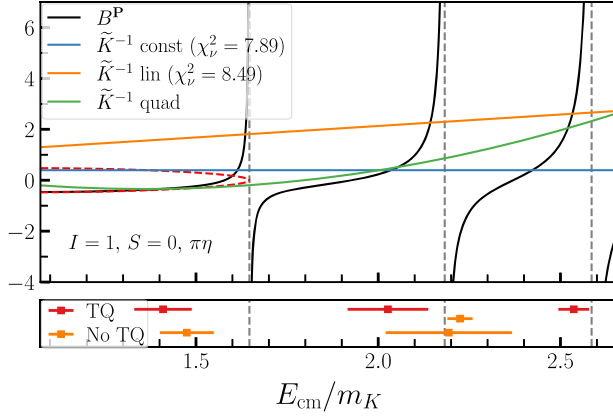
FIG. 12. Study of the Lüscher quantization condition for the I = 1, S = 0, A_{1g} channel with zero total momentum, restricted to relative orbital angular momentum \ell = 0 and the \pi\eta decay channel. Upper panel: the black curve shows the box matrix B^{(P)} function against center-of-mass energy over kaon mass, with its singularities at the noninteracting energies indicated by vertical dashed lines. Blue, orange, and green curves show the behavior of \tilde{K}^{-1} for constant, linear, and quadratic forms, respectively. Intersections of these curves with the black curves indicate the energies that satisfy the quantization condition. Vertical dashed lines indicate the noninteracting energies, and the red dashed curve is \pm\sqrt{-(k_{\pi\eta}/m_K)^2} . In the legend, \chi^2_\nu = \chi^2/N_{\text{dof}} . Lower panel: finite-volume energies for the predominantly \pi\eta states (see text) from the lattice QCD computations which include (exclude) the tetraquark operator are shown by the red (orange) points.
