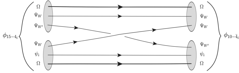
FIG. 1. Preon exchange diagram inducing the \phi_{15-4_i}^\dagger \phi_{10-\bar{4}_i} bilinear terms in the scalar potential, which are responsible for vacuum alignment along the SU(4)_{\text{PS}} \times SU(2)_{\text{R}} space. Gray bubbles represent the prebaryons (see Table II): \mathcal{P}_{15} and \mathcal{P}_4^i form the \phi_{15-4_i} di-prebaryons, while \mathcal{P}_{10} and \mathcal{P}_4^i form the \phi_{10-\bar{4}_i} di-prebaryons.
