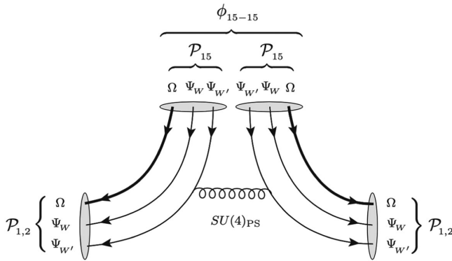
FIG. 3. Effective Yukawa interaction of the \phi_{15-15} di-prebaryon (a gauge-singlet bound state of two \mathcal{P}_{15} prebaryons) to a pair of \mathcal{P}_{1,2} prebaryons, induced by an SU(4)_{\text{PS}} gauge boson exchange.
