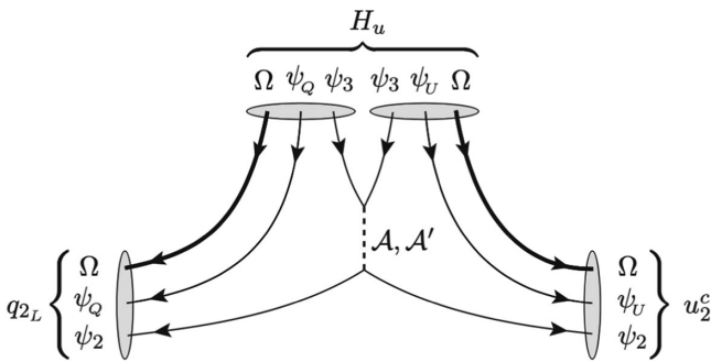
FIG. 5. Effective Yukawa coupling induced by preon interactions: the H_u Higgs doublet (a six-preon bound state) couples to the second-generation SM quark doublet ( q_{2L} ) and up-type quark singlet ( u_2^c ), producing the charm quark mass. The antisymmetric scalars \mathcal{A} and \mathcal{A}' couple to different preon flavors as in Eq. (2.1). The preon \psi_Q is the color-triplet component of \Psi_W , while the preon \psi_U is the color-antitriplet and upper- SU(2)_R component of \Psi_{W'} .
