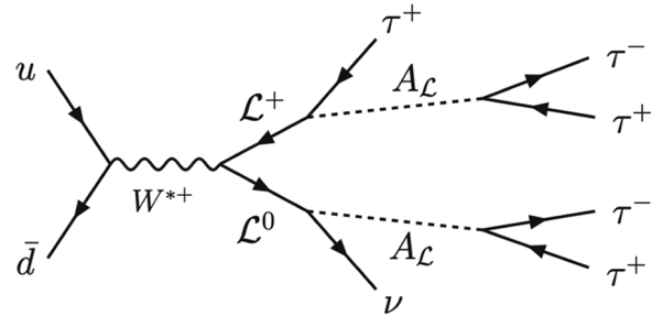
FIG. 4. Main process for pair production of composite vectorlike leptons at the LHC, yielding a 5\tau + E_{\text{f}} final state, provided that the mass of the composite pseudoscalar A_{\mathcal{L}} satisfies 2m_\tau < M_A < m_{\mathcal{L}} . For M_A < 2m_\tau , A_{\mathcal{L}} predominantly decays into \gamma\gamma or \mu^+ \mu^- , so similar diagrams lead to 4\gamma + \tau + E_{\text{f}} or 4\mu + \tau + E_{\text{f}} final states.
