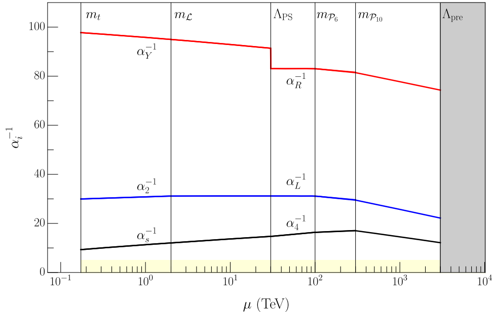
FIG. 6. Two-loop running of the inverse coupling constants ( \alpha^{-1} ) for SU(3)_c \times SU(2)_L \times U(1)_Y from the m_t scale up to \Lambda_{\text{PS}} , and for SU(4)_{\text{PS}} \times SU(2)_L \times SU(2)_R between \Lambda_{\text{PS}} and \Lambda_{\text{pre}} . Vertical lines mark various thresholds. Prebaryons \mathcal{P}_{10} , \mathcal{P}_{\bar{10}} , and \mathcal{P}_{15} , assumed to have same mass m_{\mathcal{P}_{10}} , reduce the three \alpha^{-1} near \Lambda_{\text{pre}} . Prebaryons \mathcal{P}_{6,3} and \mathcal{P}_{6,1} (of mass m_{\mathcal{P}_6} ), as well as the charged di-prebaryons and the composite vectorlike lepton (of mass m_{\mathcal{L}} ), have a similar but less notable impact. The two-loop effects of the composite singlet scalars are shown in each lower line fork near \Lambda_{\text{pre}} . The gray-shaded vertical band at \Lambda_{\text{pre}} represents the region of strongly coupled preonic SU(15)_p dynamics. The yellow-shaded horizontal band indicates the region where the three \alpha 's would no longer be perturbative.
