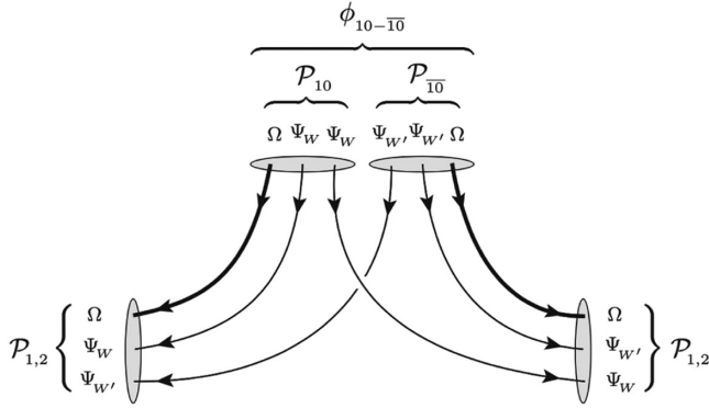
FIG. 2. Preon exchange diagram inducing the effective Yukawa interaction of the \phi_{10-\bar{10}} scalar (a gauge-singlet bound state of the \mathcal{P}_{10} and \mathcal{P}_{\bar{10}} prebaryons) to a pair of \mathcal{P}_{1,2} prebaryons.
