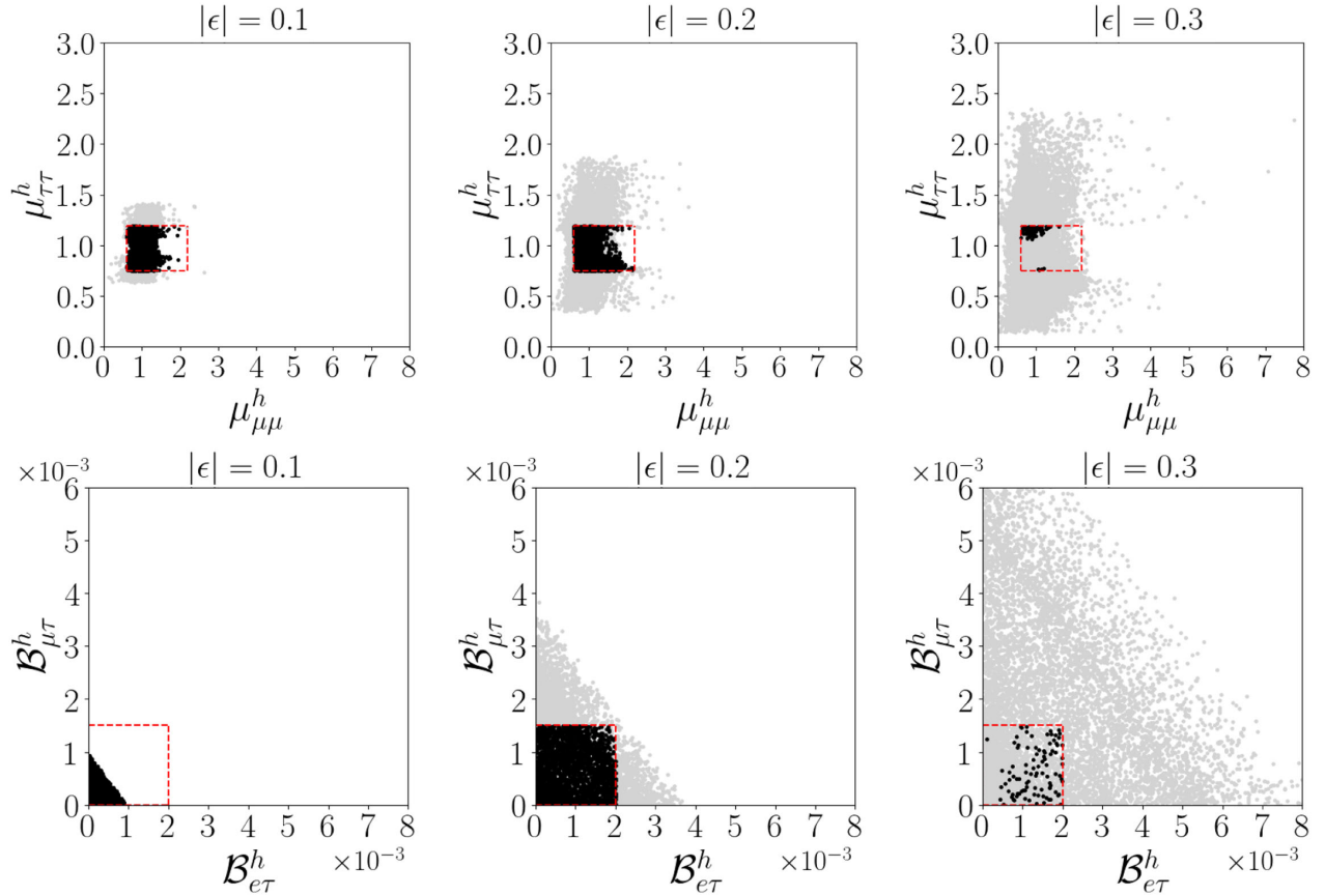
FIG. 2. The impact of the misalignment angle \epsilon on the LFC (top row) and LFV (bottom row) decays of h_{\text{SM}} . The dashed red box shows the experimental limits. The points which satisfy all six experimental limits are shown as black dots.
