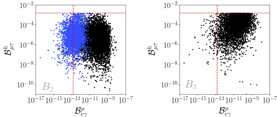
FIG. 7. The full and restricted Yukawa scans for the Yukawa scenarios B_2 (left plot) and B_3 (right plot), with the same color code as in Fig. 6.
