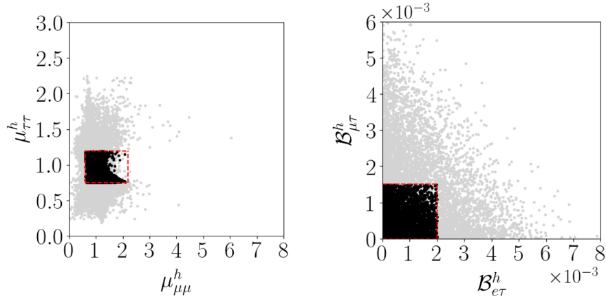
FIG. 4. A comprehensive numerical scan of h_{\text{SM}} lepton decay in high-mass region.
