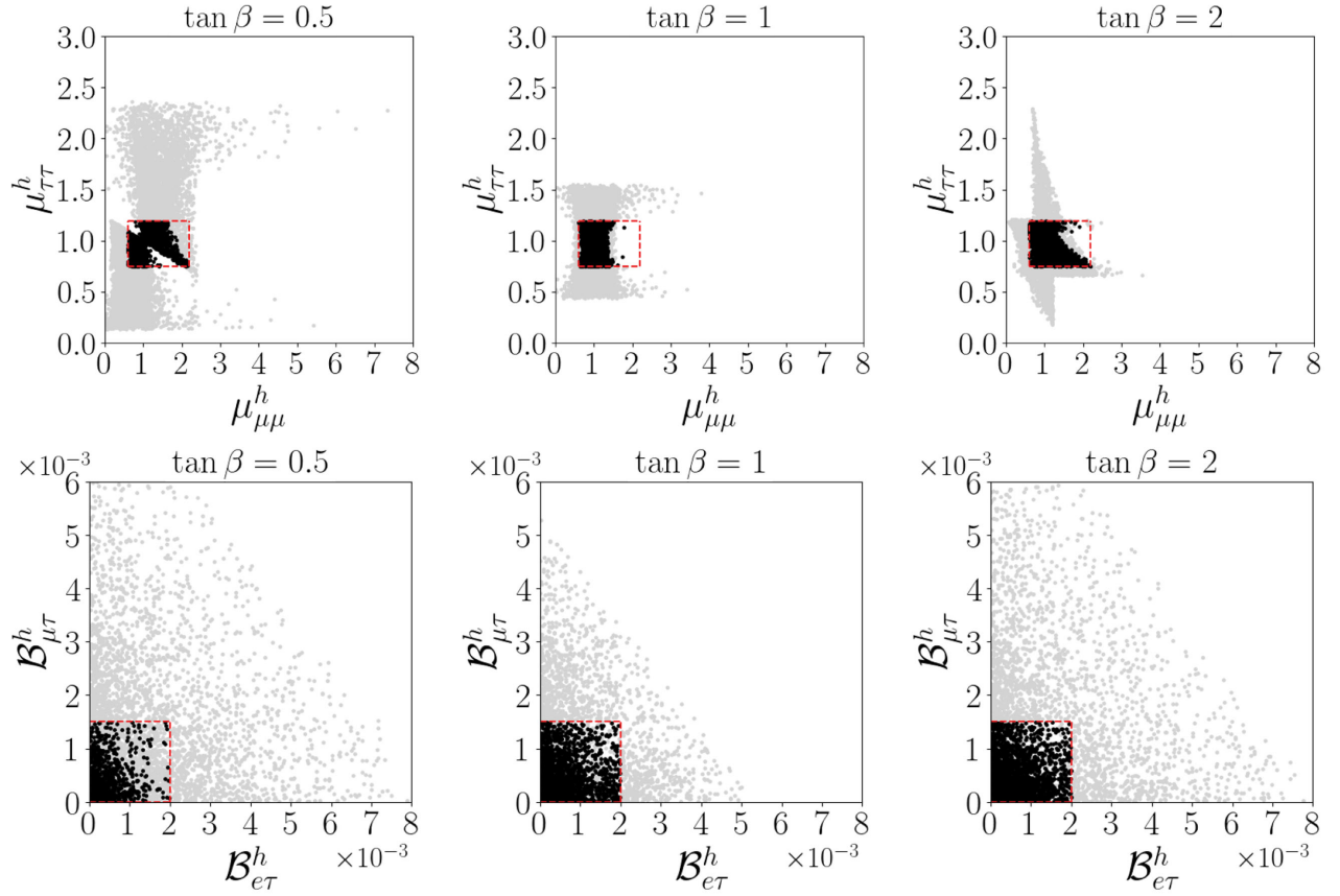
FIG. 3. The impact of \tan\beta on the LFC and LFV decays of h_{\text{SM}} . The color conventions are the same as in Fig. 2.
