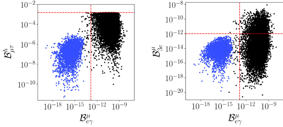
FIG. 6. The distributions of B_{e\gamma}^\mu vs B_{\mu\tau}^h (left) and B_{3e}^\mu (right). The black and blue points correspond to the full and restricted ( \theta_{\max} = \pi/100 ) Yukawa scans, respectively.
