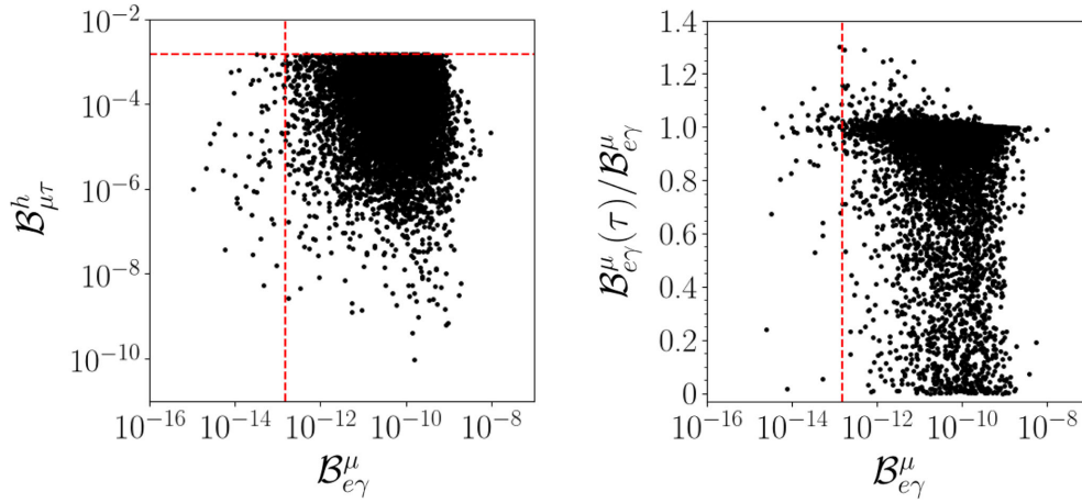
FIG. 5. Left: the results of the full Yukawa scan in the plane \mathcal{B}_{\mu\tau}^h vs \mathcal{B}_{e\gamma}^\mu . Right: the distribution of the ratio \mathcal{B}_{e\gamma}^\mu(\tau)/\mathcal{B}_{e\gamma}^\mu , the contribution of \tau propagator diagram to \mu \rightarrow e\gamma . The red dashed lines show the experimental upper limits.
