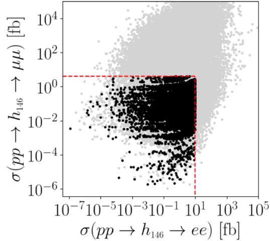
FIG. 8. The distribution of the leptonic signals \sigma(pp \rightarrow h_{146} \rightarrow ee) and \sigma(pp \rightarrow h_{146} \rightarrow \mu\mu) in the CP4 3HDM with scenario B_1 passing all the h_{SM} and \mu \rightarrow e\gamma constraints. The points that satisfy all six new experimental limits for h_{146} are shown by black dots.
