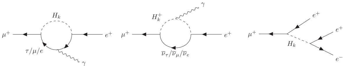
FIG. 1. One-loop Feynman diagrams for \mu^+ \rightarrow e^+ \gamma due to neutral Higgs bosons (left) and charged Higgs bosons (middle). The right diagram shows the tree-level decay of \mu \rightarrow 3e .
