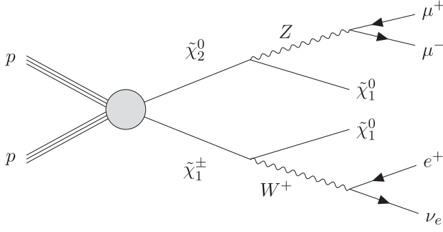
FIG. 4. Leading diagram for the leptonic MSSM signal in Sec. IV A.
