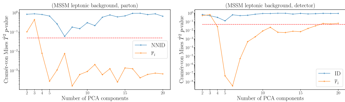
FIG. 18. CvM p values as a function of the number of principal components retained for the SM background of the MSSM leptonic signal in Sec. IV A at parton and detector level.
