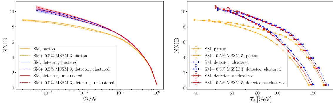
FIG. 15. NNID curves at parton, clustered detector, and unclustered detector level as a function of 2i/N (left panel) and the average distance to the i th neighbor (right panel). The central line represents the median, while the band is the 68% confidence interval.
