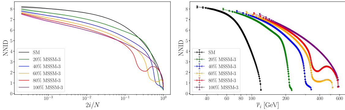
FIG. 22. Parton level NNID curves as a function of 2i/N (left panel) and the average distance to the i th neighbor (right panel) for a variable percentage of SM and MSSM-3 events in the batch, with batch size fixed at 10000 events.
