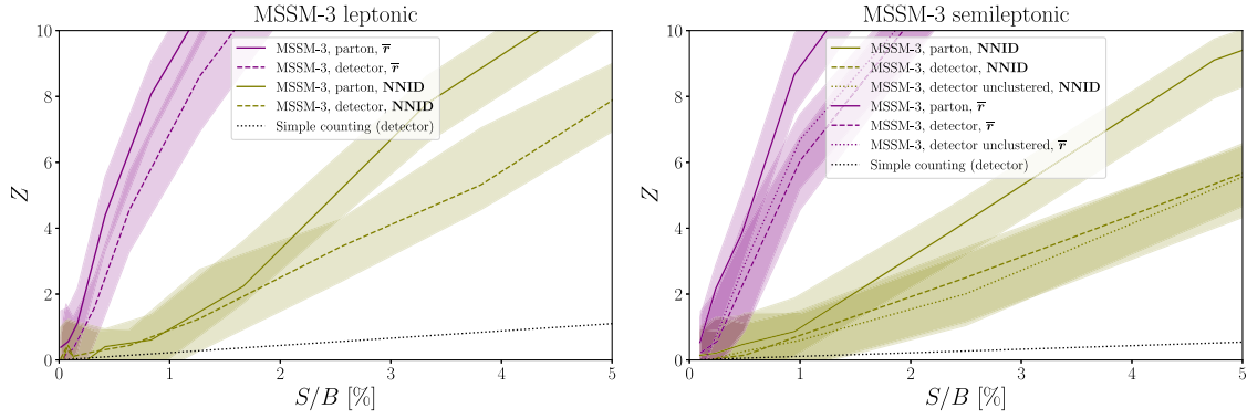
FIG. 21. Significance bands at 68% CL of the new physics test in the leptonic (left) and semileptonic (right) MSSM-3 model as a function of the signal over background rate after all cuts.
