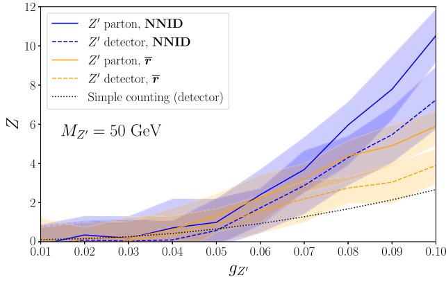
FIG. 14. Significance bands at 68% CL of the new physics test at parton and detector level, as a function of the Z' coupling to leptons. The curves are obtained using the test described in Sec. III A, either using information from the NNID (blue curves) or from \bar{r}_i (orange curves).
