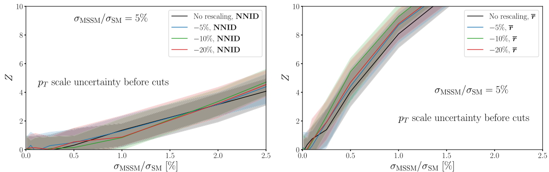
FIG. 20. Impact of a global uniform downscaling of p_T before the event selection on the significance tests with NNID and \bar{r}_i in the leptonic MSSM case.
