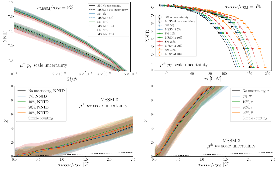
FIG. 10. Similarly to Fig. 9, a uniform rescaling of the muons and antimuons p_T has only a minor impact on the NNID and on the significance of the test.
