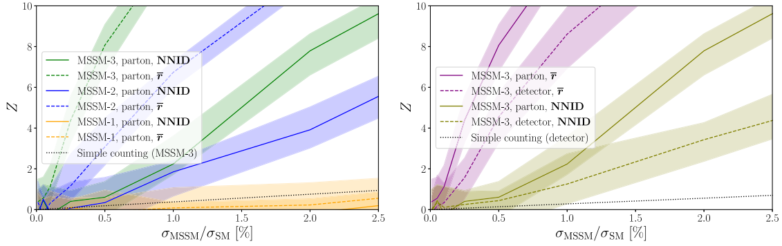
FIG. 6. Left panel: Parton level significance of the NNID and \bar{r}_i new physics search versus the fraction of BSM events in the sample, for the three MSSM leptonic benchmarks described in Sec. IV A. The solid and dashed lines are the median significances and are shown with the corresponding 68% CL band. The black dotted line corresponds to the simple counting significance, Z \sim S/\delta B . Right panel: Comparison of the parton level and detector level significances for the MSSM-3 benchmark model.
