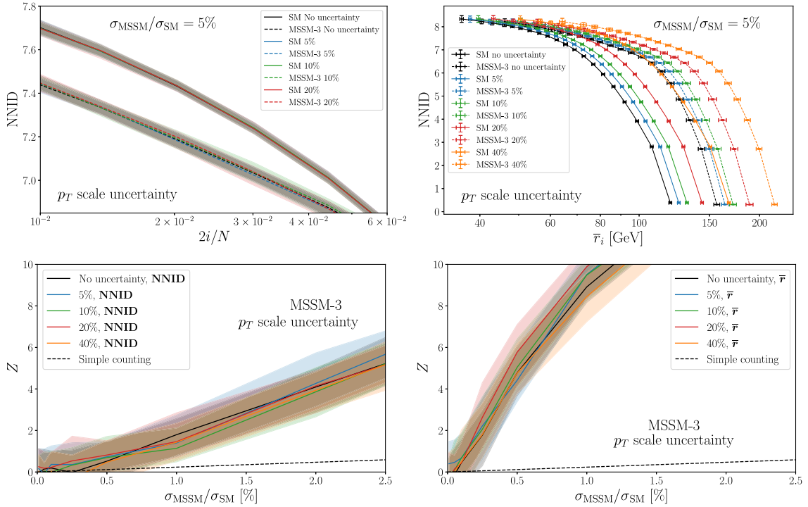
FIG. 8. Constant, uniform rescaling of all particles' p_T leaves the NNID invariant, and thus the significance remains unchanged (left panels). The distances \bar{r}_i get uniformly rescaled, but the significance is still unaltered (right panels). We rescale the p_T by up to 40% in the figure, but we could have further increased this factor with no visible effect. The figure demonstrates the insensitivity of our new physics search to energy scale uncertainties.
