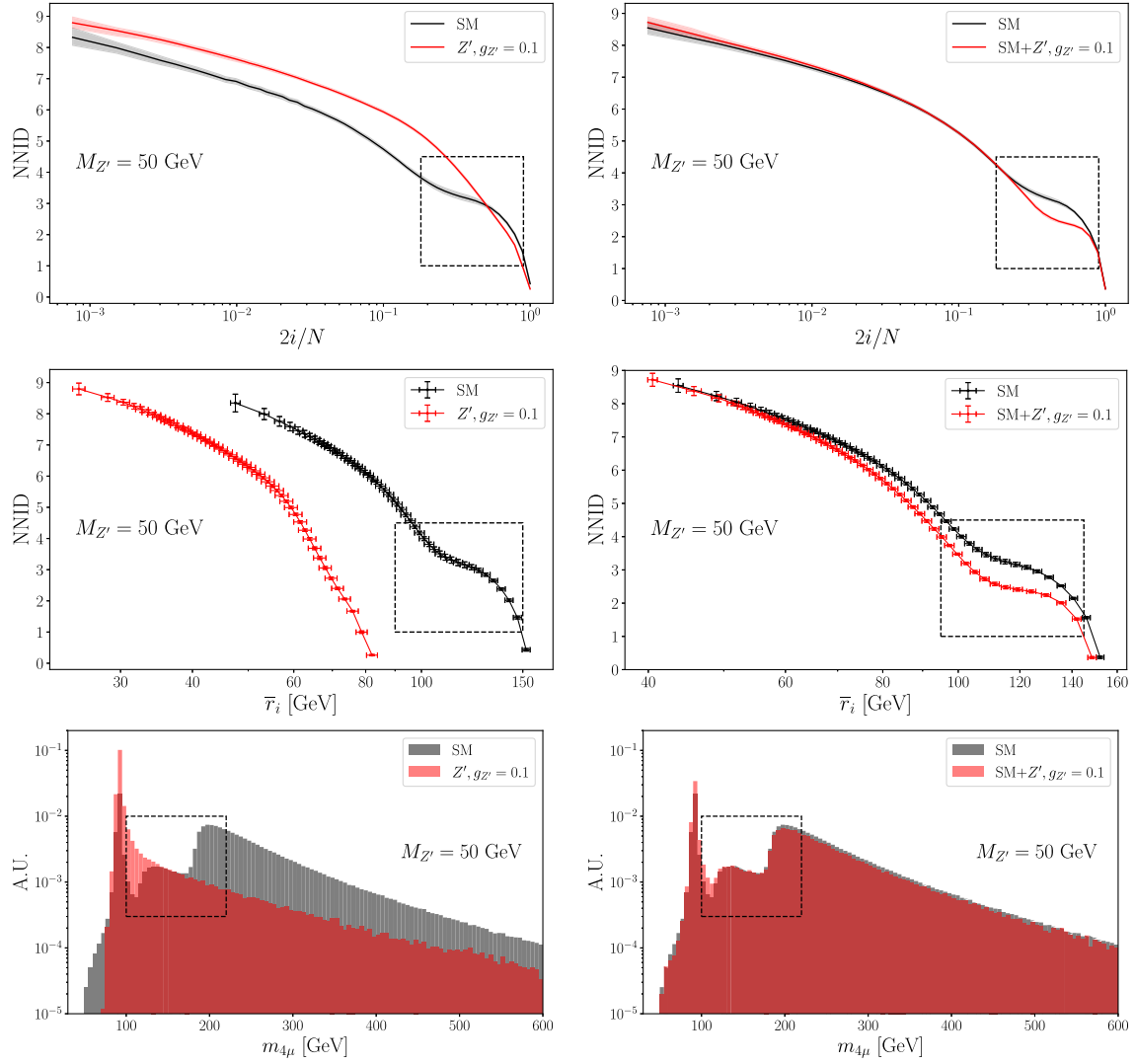
FIG. 13. NNID curves at parton level as a function of 2i/N and \bar{r}_i in the pure SM and pure Z' samples (left). In the right panels we show a comparison between the SM and the SM + Z' samples. The mass of the Z' is fixed to M_{Z'} = 50 GeV with coupling g_{Z'} = 0.1 , and the curves are obtained with a fixed number of SM events N = 2613 for illustrative purposes. The bottom row shows the invariant mass distribution of the four muons in the event. We highlight with a dashed black box the region of the NNID curves corresponding to the two shoulders in the invariant mass distribution of the bottom panels.
