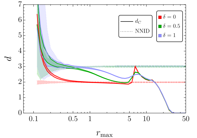
FIG. 2. Comparison of the correlation dimension d_C (solid lines) and the NNID (dotted lines) for a Swiss roll. The NNID is computed at i = 1 and j = 2 and by definition is insensitive to cutting the largest distances in the dataset. The parameter \delta , defined in the text, quantifies the thickness of the Swiss roll. The shaded areas give the 95% CL interval for the two estimators.
