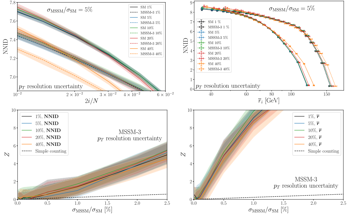
FIG. 11. Robustness of the NNID and the associated statistical test to a Gaussian smearing of all particles' p_T . The figure demonstrates the insensitivity of our new physics search to energy resolution uncertainties.
