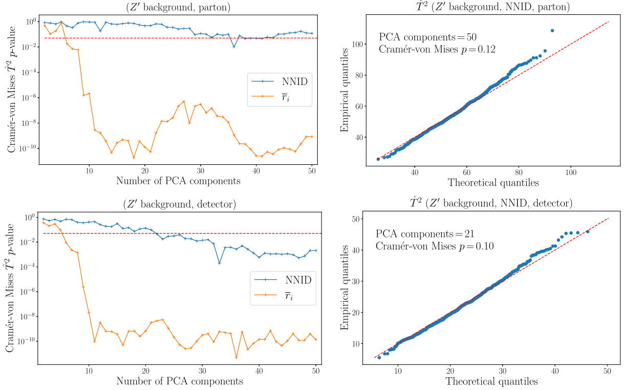
FIG. 17. CvM p value as a function of the number of principal components retained for the SM background of the Z' signal in Sec. IV B. The right panel shows the qualitative agreement at the optimal number of components via a Q-Q plot for the NNID vector.
