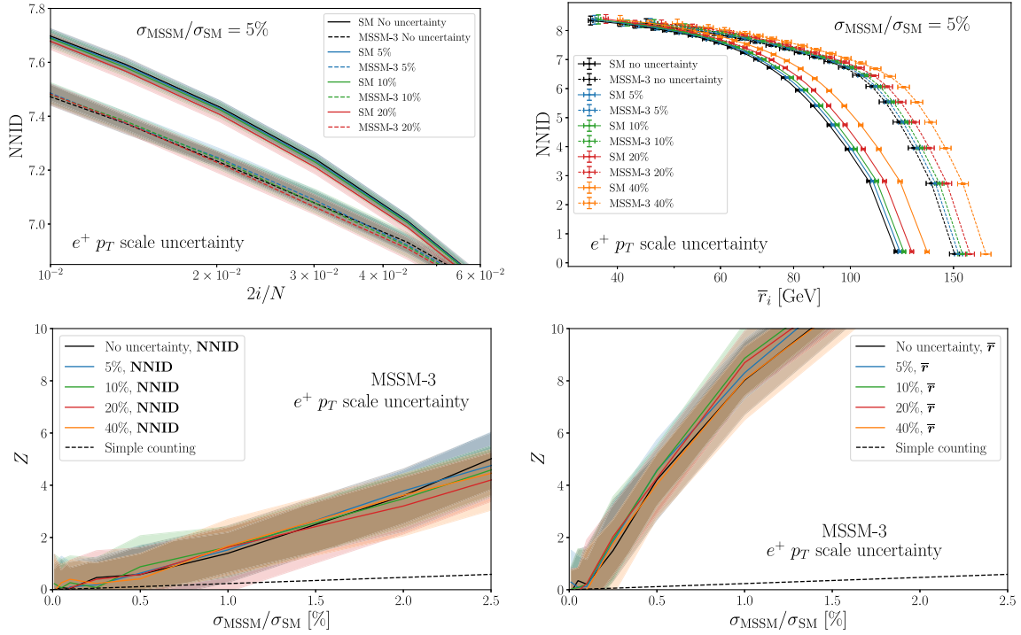
FIG. 9. Uniform rescaling of the positron p_T has only a minor impact on the NNID and on the significance of the test. See the text for more details.
