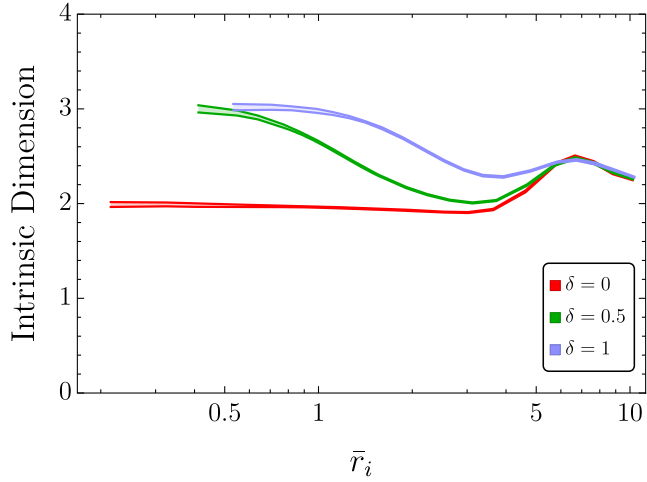
FIG. 3. Intrinsic dimension of a Swiss roll for different choices of the noise \delta , i.e., its thickness. On the x axis we show the average distance of the i th neighbor, on the y axis the NNID calculated at j = 2i . The shaded areas give the 95% CL interval for the estimator. We truncate our lines at the value of \bar{r}_i below which there are no more neighbors.
