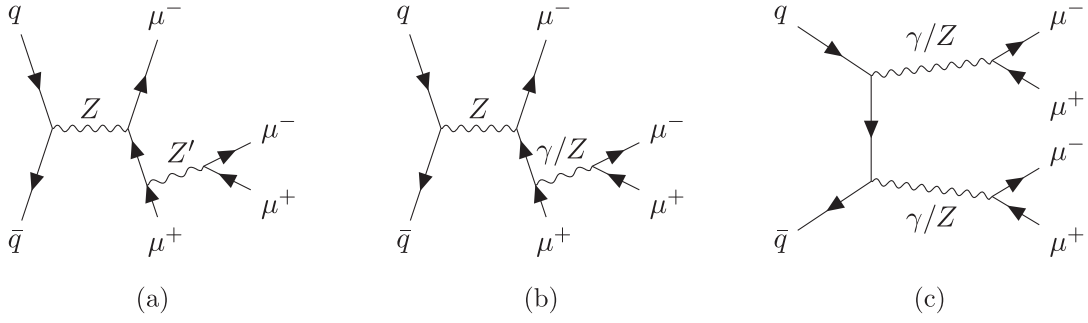
FIG. 12. Dominant production mechanism for the Z' signal in Sec. IV B (a) and leading SM backgrounds (b), (c).
