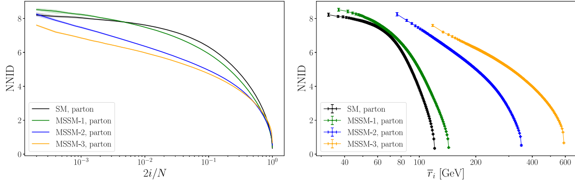
FIG. 5. Parton level NNID curves as a function of 2i/N (left panel) and the average distance to the i th neighbor (right panel) in the SM (black) and in three MSSM-like benchmark models described in the text. The curves are obtained from 100 samples. In the left panel the central line represents the median, while the band is the 68% confidence level. In the right panel we show the 68% confidence level for both axes as error bars.
