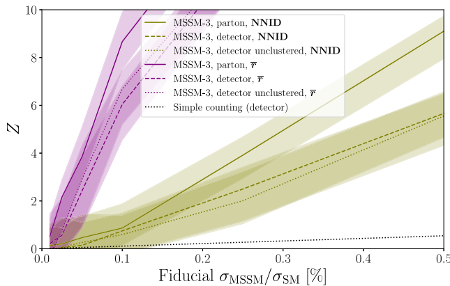
FIG. 16. Significance bands at 68% CL of the new physics test in the semileptonic MSSM-3 model at parton level and detector level (with clustered and unclustered jets), as a function of the ratio between the BSM and SM cross section in the fiducial region.
