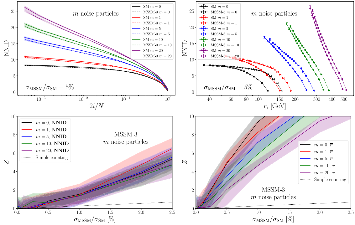
FIG. 7. Top row: NNID curves at detector level in the SM and MSSM-3 benchmark models described in Section IV A with a variable number m of spectator particles (i.e., fictitious particles that are identical in the MSSM-3 and SM samples). Bottom row: the significance of the NNID new physics test for the MSSM-3 benchmark model remains stable if the number m of spectator particles is increased, while the \bar{r}_i test suffers more.
