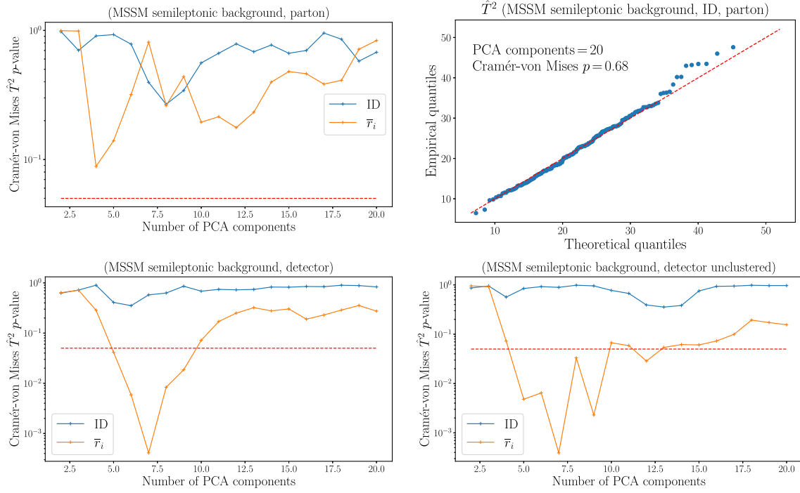
FIG. 19. Q-Q plot corresponding to the optimal number of PCA components for the NNID vectors at parton level (top right), and CvM p value as a function of the number of principal components retained for the SM background of the MSSM semileptonic signal in Sec. IV C.
