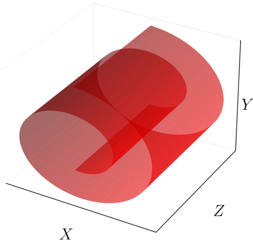
FIG. 1. Sketch of a Swiss-Roll manifold.
