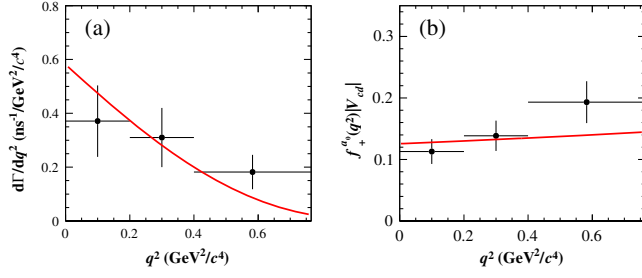
FIG. 3. Fit to the differential decay rate as function of q^2 (a) and projection to the FF f_+^{a_0}(q^2)|V_{cd}| (b). The points with error bars are data. The red solid line is the fit result.
