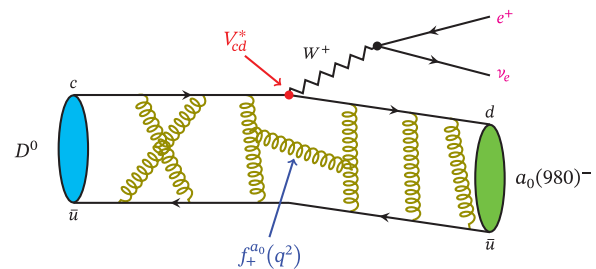
FIG. 1. Decay mechanism diagram of the D^0 \rightarrow a_0(980)^- e^+ \nu_e decay. It illustrates a clear separation of the weak current, W^+ \rightarrow e^+ \nu_e , and strong current, D^0 \rightarrow a_0(980)^- , in SL decay. The transition of D^0 \rightarrow a_0(980)^- is parametrized by the FF f_+^{a_0}(q^2) . The green region represents the hadronization process of the a_0(980)^- , which may form either as a conventional d\bar{u} state or an exotic d\bar{u}s\bar{s} state with the s\bar{s} generated from gluon interactions.
