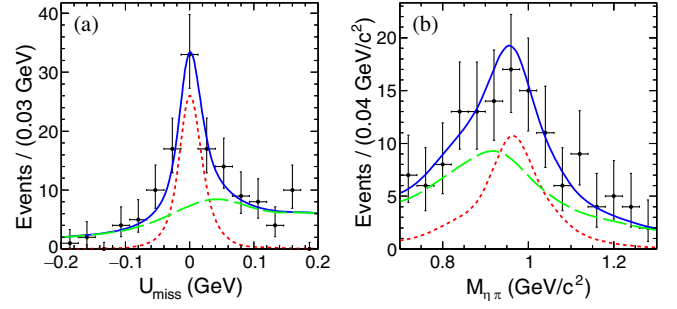
FIG. 2. Projections of the 2D fit on U_{\text{miss}} (a) and M_{\eta\pi^-} (b) for D^0 \rightarrow a_0(980)^- e^+ \nu_e . The points with error bars are data. The (blue) solid curves are the overall fits, the (red) short-dashed lines show the fitted signal shape; the (green) long-dashed lines denote the background shape.
