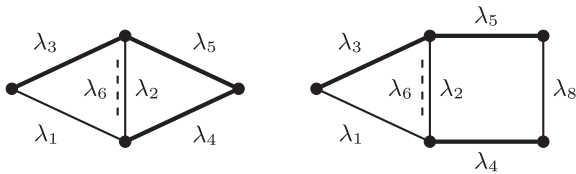
FIG. 2. The graph topologies of master integrals, edges labeled by \lambda_r defined in (22). The dashed line is the delta constraint originating from the exponential factor. The thick lines are remaining delta constraints, while the thin lines are physical propagators.
