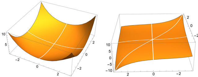
FIG. 1. G_1(x_1)G_1(x_2) (left) and G_2(x_1, x_2) (right).
