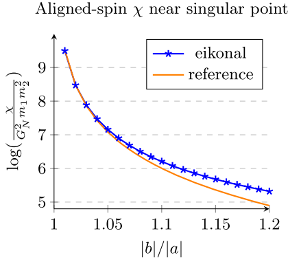
FIG. 4. Aligned-spin \chi near the singular point |b| = |a| . The curve \frac{\beta}{(|b|^2 - |a|^2)^{3/2}} intersects at |b| = 1.02|a| .
