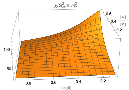
FIG. 3. The eikonal (20) as a function of \frac{|a|}{|b|} and \cos(\theta) = \frac{-a \cdot b}{|a||b|} with numerical errors \sim 10^{-15} .
