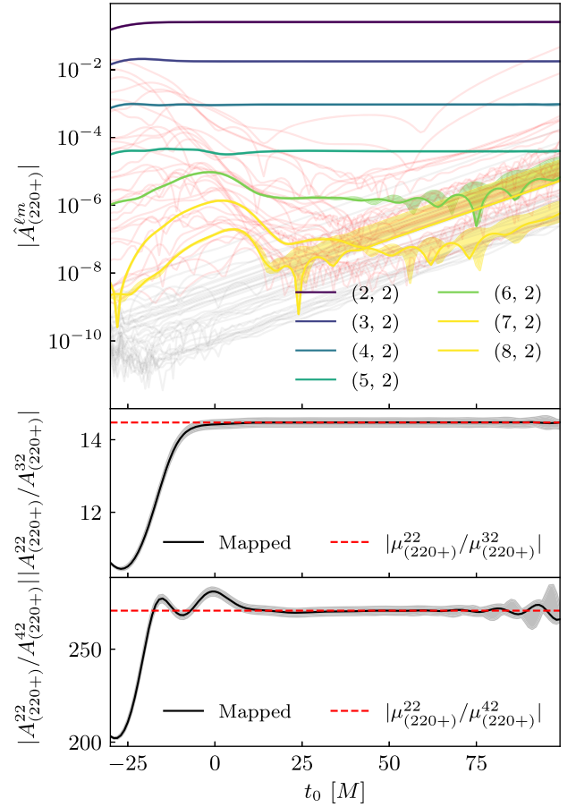
FIG. 5. The magnitudes of the decay-corrected amplitudes, |\hat{A}_{(220+)}^{\ell m}| , obtained from spatial mapping of the (2, 2, 0, +) mode for the 0001 waveform are plotted. The thick colored lines show the spherical modes indicated in the legend that are expected to have large amplitudes. Translucent grey lines indicate odd m modes, and the translucent red lines indicate even m \neq 2 modes. The ratios of selected amplitudes are plotted in the lower panels. The values for the ratios of the spheroidal harmonics predicted by linear PT (expressed in terms of ratios of mode-mixing coefficients) are plotted as horizontal dashed lines. The translucent area surrounding the lines on the three panels indicates the NR uncertainty in the values obtained. The way this is determined is described in Appendix D.
