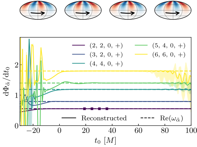
FIG. 4. The top four figures show the real part of the spatial reconstruction of the (2, 2, 0, +) QNM at the start times indicated by squares on the main plot. These demonstrate the rotation of the QNM around the sphere. Main plot: Derivative of the argument \Phi_\alpha of the spatial mismatch (corresponding to the phase shift between the mapped and predicted spatial structures) with respect to ringdown start time t_0 . The solid lines show this quantity for simulation 0001 for the same 5 QNMs (matching colors) used in the left panel of Fig. 3. The shaded regions give an estimate of the error in the reconstructed frequencies and are described in Appendix D. The horizontal dashed lines give the predicted rotation frequencies, which are the real part of the complex QNM frequencies, \omega_\alpha . An animated version of these outcomes showing the rotation around the BH is available at [58].
