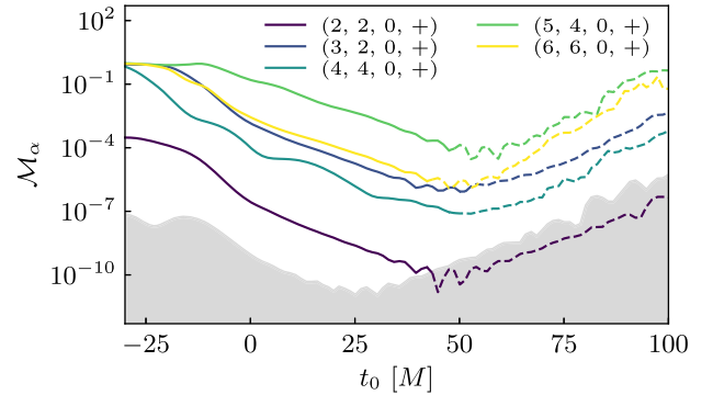
FIG. 14. The spatial mismatch between spatially reconstructed QNMs and the expected spheroidal harmonics. Here, the loudest QNMs for each \ell in simulation 0001 up to \ell = 6 are mapped simultaneously. This is in contrast with the left-hand panel of Fig. 3, where each QNM is spatially mapped individually. The grey region indicates the NR error in the (2, 2, 0, +) mode, and the change in the style of each line from solid to dashed indicates the point where the spatial mismatches first drop below their corresponding error thresholds. Only QNMs and spherical modes with m \in \{2, 4, 6\} are used.
