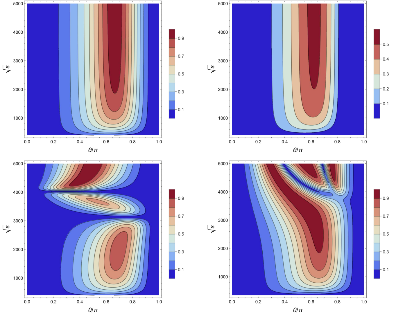
FIG. 4. Contours of the concurrence in the (\sqrt{s}, \theta/\pi) plane. The panel assignments are the same as in Fig. 2 for the entanglement marker.
