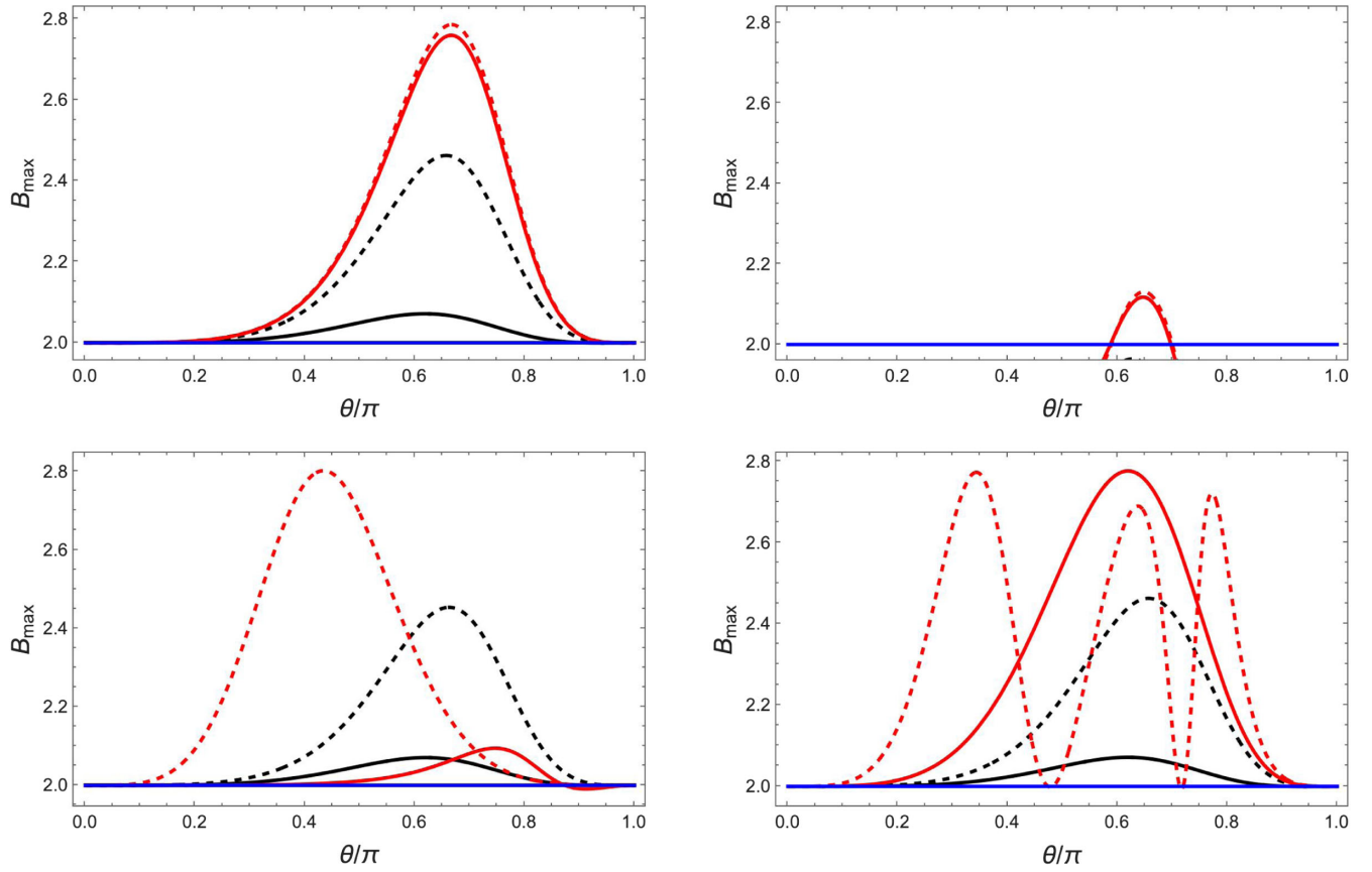
FIG. 7. Angular dependence of the CHSH Bell parameter at fixed center-of-mass energies. The panel assignments are the same as in Fig. 3. The solid black, dashed black, solid red, and dashed red curves correspond to \sqrt{s} = 500 GeV, 1000 GeV, 3000 GeV, and 4500 GeV, respectively. The horizontal blue line marks the classical CHSH bound B_{\max} = 2 .
