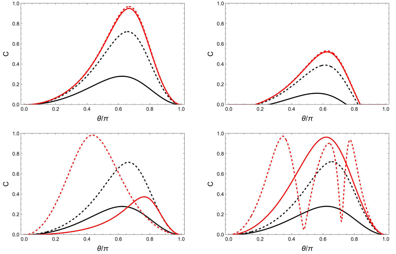
FIG. 5. Angular dependence of the concurrence at fixed center-of-mass energies. The panel assignments are the same as in Fig. 3. The solid black, dashed black, solid red, and dashed red curves correspond to \sqrt{s} = 500 GeV, 1000 GeV, 3000 GeV, and 4500 GeV, respectively.
