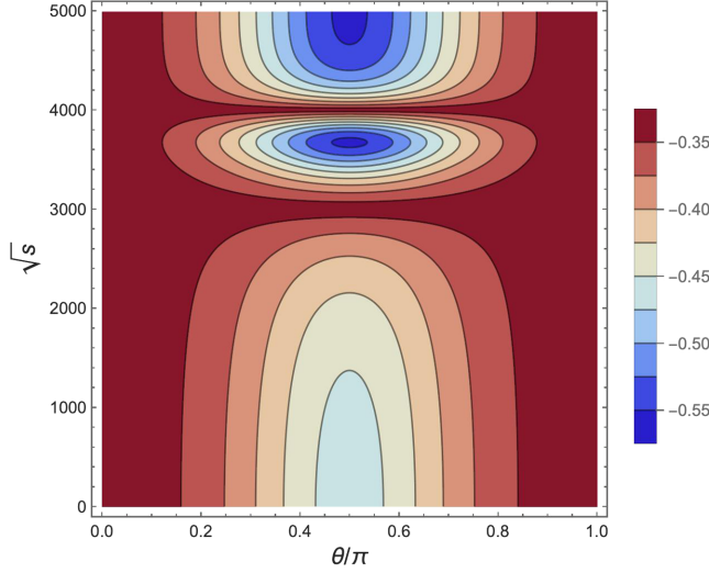
FIG. 9. Contour plot of the entanglement marker obtained from (B11) with parameters in (B22).
