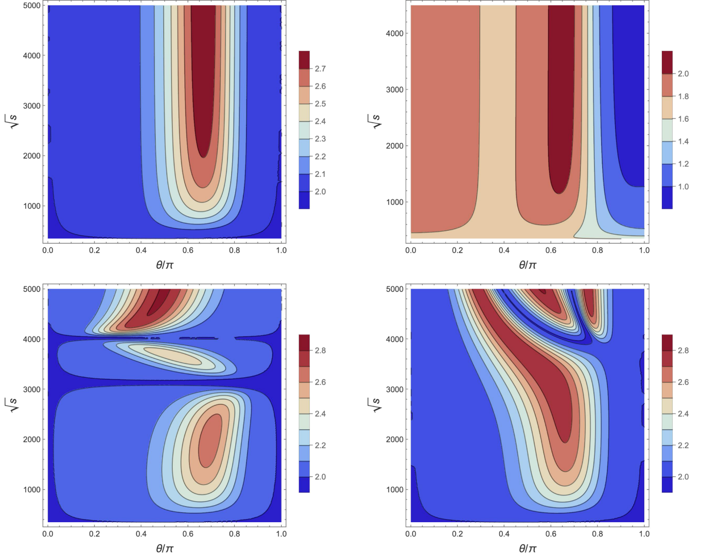
FIG. 6. Contours of the CHSH Bell parameter in the (\sqrt{s}, \theta/\pi) plane. The panel assignments are the same as in Fig. 2 for the entanglement marker.
