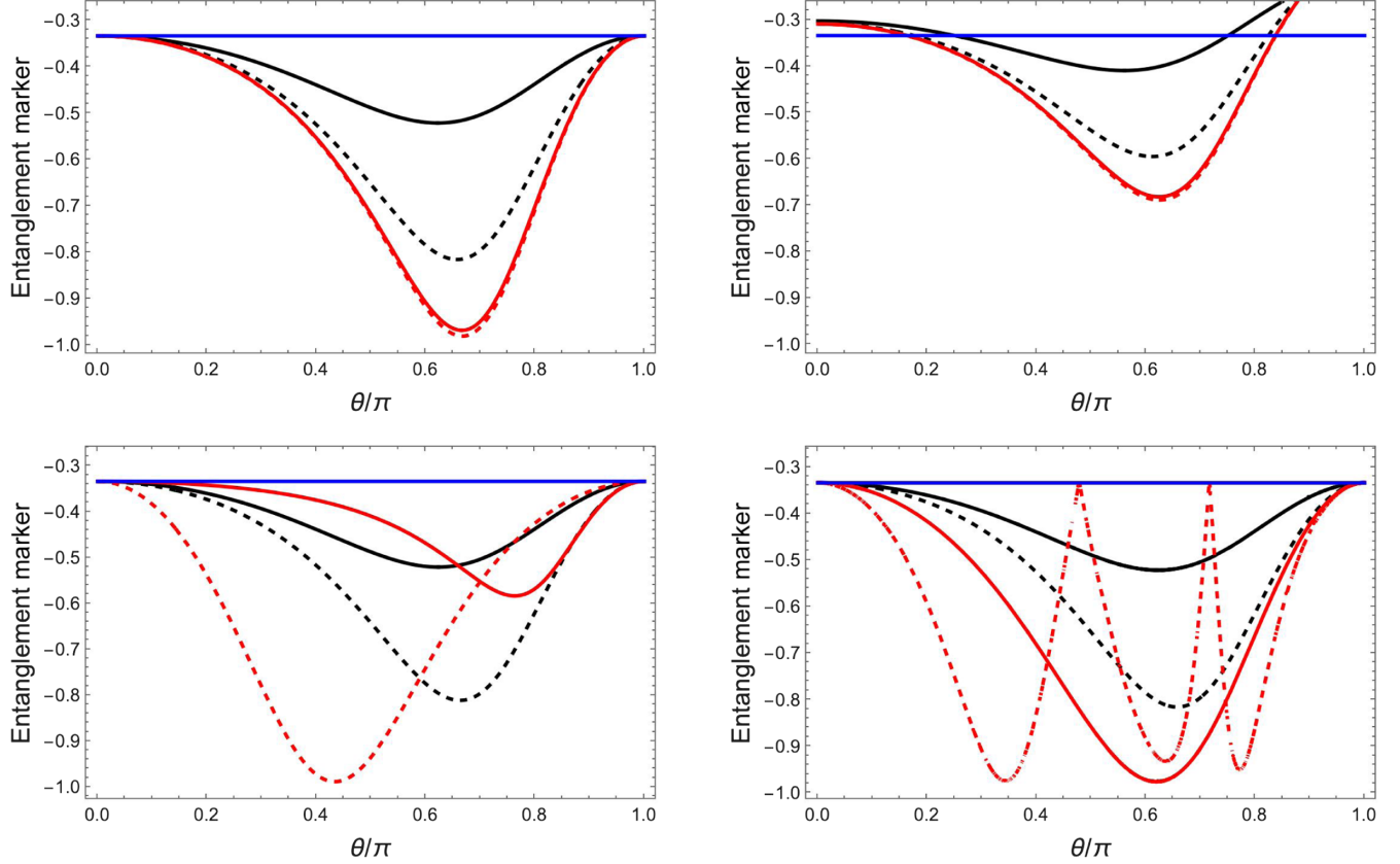
FIG. 3. Angular dependence of the entanglement marker at fixed center-of-mass energies for the SM (top left), the scalar-mediator model (top right), the U(1)_{B-L} model (bottom left) and RS model. The solid black, dashed black, solid red, and dashed red curves correspond to \sqrt{s} = 500 GeV, 1000 GeV, 3000 GeV, and 4500 GeV, respectively. The horizontal blue line indicates the threshold below which the state is entangled.
