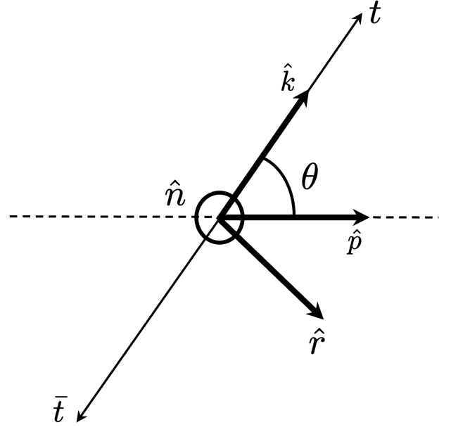
FIG. 1. Orthonormal basis (\hat{r}, \hat{n}, \hat{k}) in the t\bar{t} rest frame, defined with respect to the top-quark direction \hat{k} and beam direction \hat{p} .
