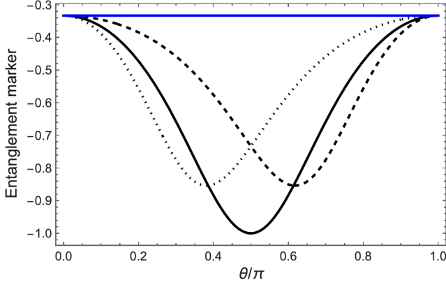
FIG. 8. Angular dependence of the entanglement marker for several representative choices of chiral couplings. The blue horizontal line denotes the separability bound, D_{\min} = -1/3 . The solid curve corresponds to vectorlike couplings P = Q , ( g_R^e = g_L^e = g_R^t = g_L^t = 1 ), while the dashed and dotted curves illustrate the cases P > Q ( g_R^e = g_R^t = 3, g_L^e = g_L^t = 1 ) and P < Q ( g_R^e = g_R^t = 1, g_L^e = g_L^t = 3 ), respectively. The minimum shifts according to Eq. (A17), demonstrating that its angular position is determined by the relative strengths of the left- and right-chiral couplings.
