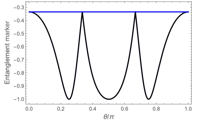
FIG. 10. Entanglement marker obtained by retaining only the first KK graviton in the massless-top limit, with the SM amplitudes omitted. The blue horizontal line denotes the separability bound, D_{\min} = -1/3 , while the black curve shows the entanglement marker induced by the first KK graviton. The disconnected entangled regions are already present for a single spin-2 KK mode, demonstrating that they originate from the characteristic angular dependence of the spin-2 exchange.
