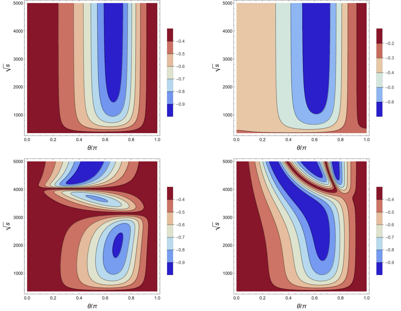
FIG. 2. Contours of the entanglement marker in the (\sqrt{s}, \theta/\pi) plane. The top panels show the SM (left) and the scalar-mediator model (right), while the bottom panels show the U(1)_{B-L} model (left) and the RS model (right).
