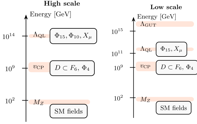
FIG. 2. Schematic distribution of the field masses and relevant energy scales of the theory. The three main scales of the theory are shown: the electroweak scale ( M_Z ), the scale of spontaneous CP violation ( v_{CP} \sim \langle \phi_4^0 \rangle ), and the quark-lepton unification scale ( \Lambda_{QL} \sim \langle \phi_{15}^0 \rangle ). The matter content consists of the SM fields, embedded in three copies of F_{QL} \sim (4, 2, 0)_{PS} , F_{uv} \sim (4, 1, 1/2)_{PS} , and F_{de} \sim (4, 1, -1/2)_{PS} , together with the Higgs doublet H \sim (1, 2, 1/2)_{PS} . The theory also contains a vectorlike down quark D \subset F_6 \sim (6, 1, 0)_{PS} responsible for (i) correcting the M_d = M_e relation for the two heaviest generations and (ii) solving the strong CP problem à la Nelson-Barr. The scalar sector includes \Phi_{15} , responsible for breaking SU(4)_C \rightarrow SU(3)_C \otimes U(1)_{B-L} , and \Phi_4 , whose VEV triggers spontaneous CP violation. In the high-scale \Lambda_{QL} scenario (left panel), \Phi_{10} breaks U(1)_{B-L} \otimes U(1)_R \rightarrow U(1)_Y with \langle \phi_{10}^0 \rangle of order the quark-lepton unification scale. Then, the hierarchy between the quark-lepton unification scale and the electroweak scale ( \Lambda_{QL}/M_Z \sim 10^{12} ) generates active neutrino masses via the type I seesaw mechanism, consistently with neutrino data. In turn, the gap between the quark-lepton unification scale and the Planck scale ( \Lambda_{QL}/M_{Pl} \sim 10^{-5} ) accounts for the observed down-quark mass through nonrenormalizable operators. In the low-scale \Lambda_{QL} scenario (right panel), v_{CP} \ll \Lambda_{QL} = \mathcal{O}(10^{11}) GeV, which is consistent with SO(10) grand unification at \Lambda_{GUT} \gtrsim 10^{15} GeV, and consistent down quark masses if these are generated by physics mediated at the GUT scale. In this scenario, neutrinos are expected to get mass via the inverse seesaw mechanism.
