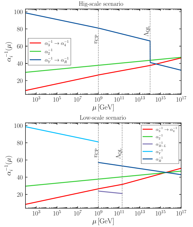
FIG. 3. One-loop running of the gauge couplings in the two quark-lepton-unification scenarios. The upper panel corresponds to high-scale quark-lepton unification, \Lambda_{QL} = 10^{14} GeV, while the lower panel corresponds to low-scale quark-lepton unification, \Lambda_{QL} = 2 \times 10^{11} GeV. The lower panel running points toward an SO(10) -like unification scale \Lambda_{GUT} \simeq 3 \times 10^{15} GeV. Details of the gauge-coupling renormalization group equations are given in Appendix C.
