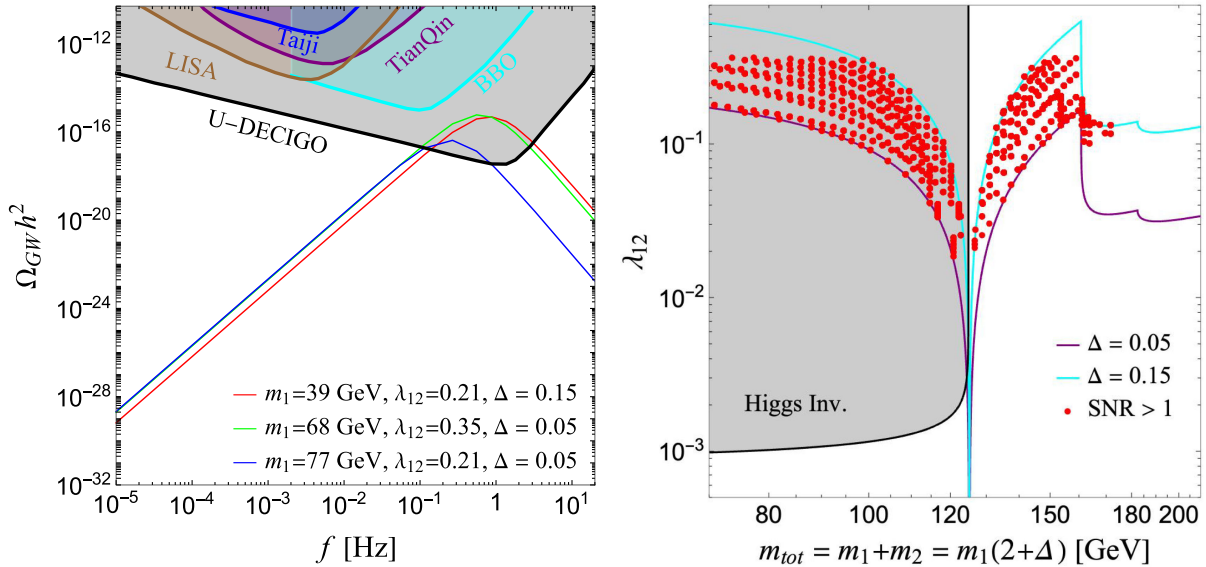
FIG. 3. Left: A representative gravitational wave spectrum is shown in comparison with the sensitivity curve of several GW detectors (obtained by scanning over the parameter \lambda_\phi to maximize the signal). Right: Red dots represent regions of parameter space that yield strongly first-order phase transitions with a GW signal-to-noise ratio \text{SNR} > 1 . The cyan and purple lines indicate regions consistent with relic abundance constraints for \Delta = 0.15 and 0.05 . The shaded region represents constraints from the Higgs invisible decay.
