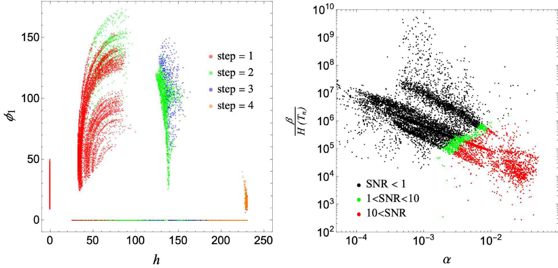
FIG. 4. Final phase points in multistep phase transitions (left) and the corresponding SNR, \alpha , and \beta/H(T_n) values across different model parameters (right). Red points indicate parameter regions where SNR > 10.
