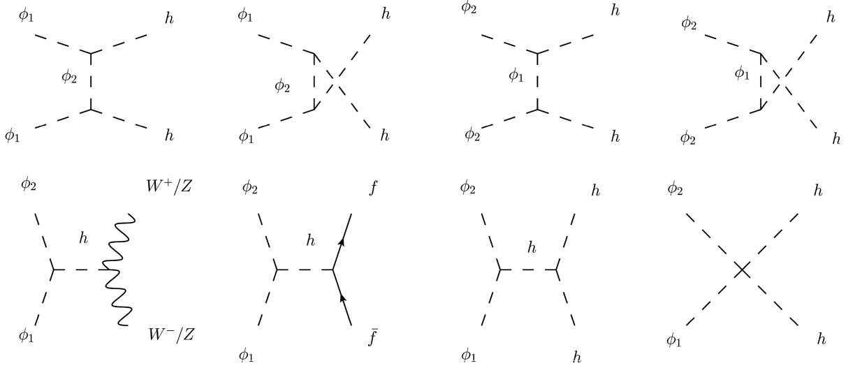
FIG. 2. Feynman diagrams for the annihilation processes \phi_i \phi_j \rightarrow \text{SM SM} .
