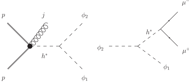
FIG. 5. Feynman diagrams for productions and decays of DM partner \phi_2 at the HL-LHC.
