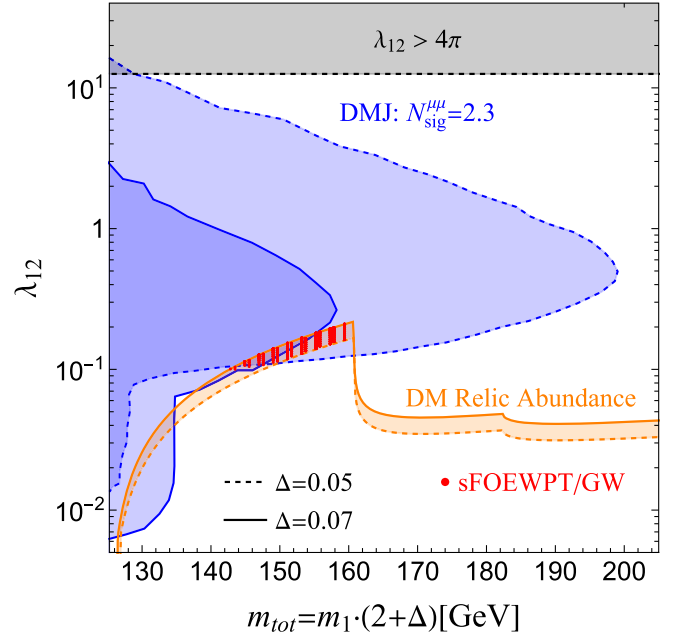
FIG. 6. Expected sensitivities at the future HL-LHC to the scalar iDM model in the parameter space determined by \lambda_{12} and m_{\text{tot}} = m_1 + m_2 = m_1 \cdot (2 + \Delta) , with an integrated luminosity of \mathcal{L} = 3 \text{ ab}^{-1} and a center-of-mass energy of \sqrt{s} = 14 \text{ TeV} , where the mass splitting \Delta = 0.05 (dashed) and 0.07 (solid). The projected sensitivity for the displaced muon-jets method with 2.3 signals is depicted by the blue dashed (solid) contour lines. The dashed (solid) orange line and the orange-shaded region depict the parameter space consistent with the observed Dark Matter relic abundance for \Delta = 0.05 ( \Delta = 0.07 ) and \Delta ranging from 0.05 to 0.07. The red points labeled “sFOEWPT/GW” within this orange-shaded area highlight the regions of strongly FOEWPT with GWs to be explored in forthcoming GW observatories for \Delta \in [0.05, 0.07] . Additionally, the gray-shaded region identifies areas where \lambda_{12} surpasses 4\pi .
