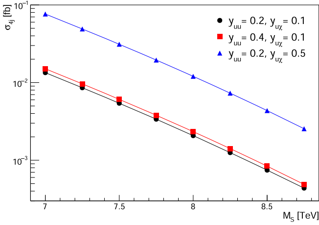
FIG. 2. pp \rightarrow S_{uu} \rightarrow u\chi \rightarrow u(Wb) \rightarrow u(jjb) cross section as a function of M_S for three Yukawa coupling scenarios.
