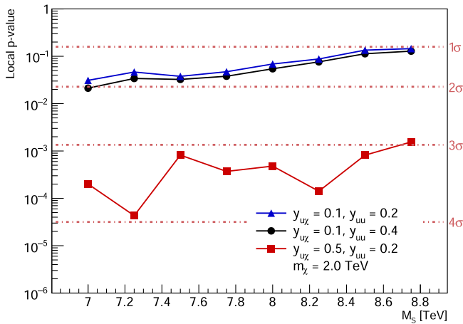
FIG. 9. Local p -value for \chi \rightarrow Wb and m_\chi = 2 TeV, comparing three different Yukawa coupling combinations.
