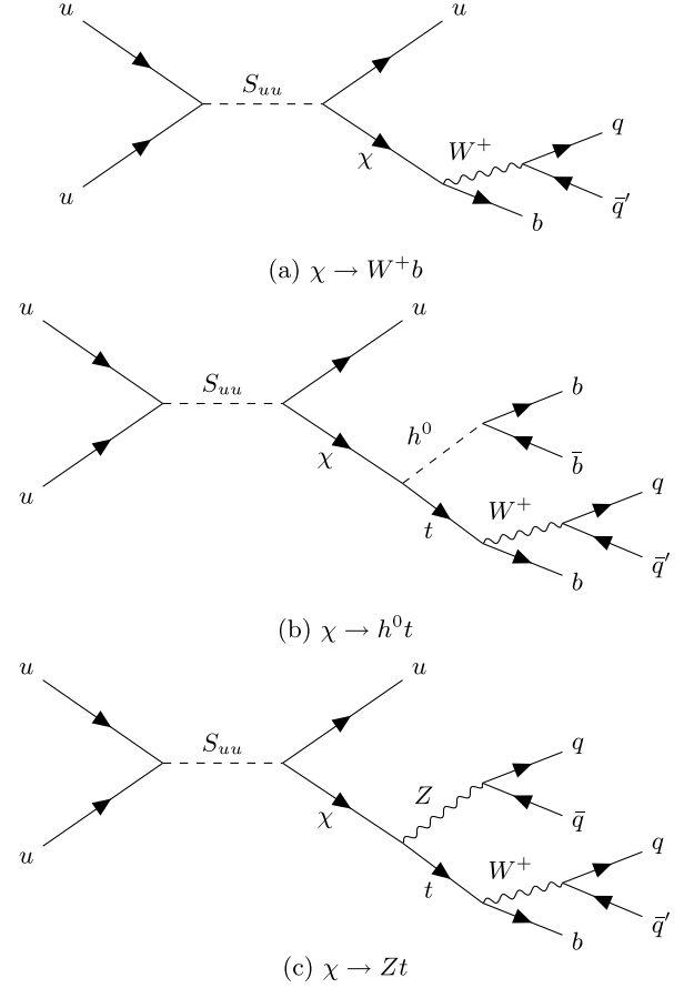
FIG. 1. The Feynman diagrams of the S_{uu} \rightarrow u\chi decay modes in fully hadronic final states.
