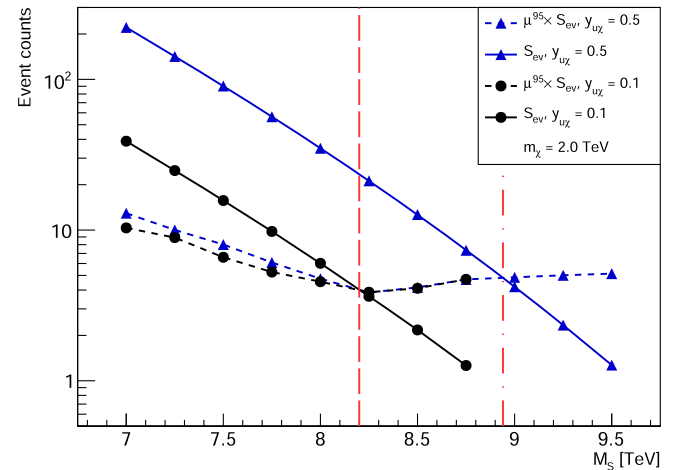
FIG. 6. 95% CL upper limits on \mu^{95} \times S_{\text{ev}} for \chi \rightarrow Wb , comparing y_{u\chi} = 0.1 and 0.5 at fixed y_{uu} = 0.2 .
