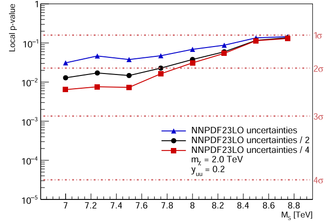
FIG. 10. Local p -value for \chi \rightarrow Wb , y_{uu} = 0.2 and m_\chi = 2 TeV, comparing different PDF uncertainty scenarios.
