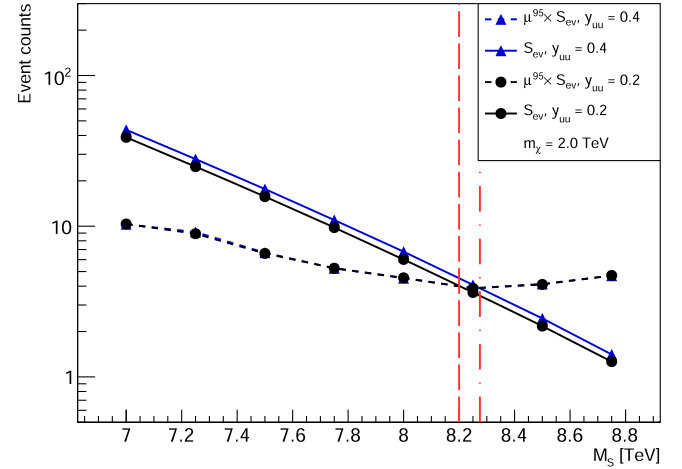
FIG. 5. 95% CL upper limits on \mu^{95} \times S_{\text{ev}} for \chi \rightarrow Wb , comparing y_{uu} = 0.2 and 0.4 at m_\chi = 2 TeV.
