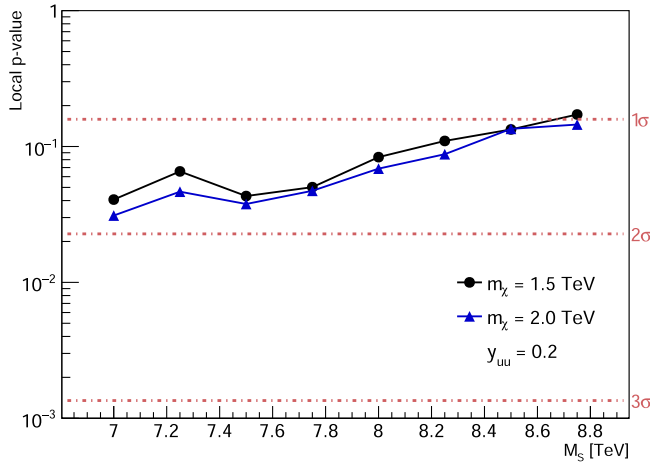
FIG. 8. Local p -value and y_{uu} = 0.2 , comparing m_\chi = 1.5 and 2 TeV.
