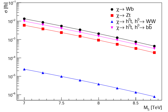
FIG. 3. Fully hadronic cross sections for different \chi decay modes in S_{uu} \rightarrow u\chi at \sqrt{s} = 13.6 TeV, for y_{uu} = 0.2 and y_{u\chi} = 0.1 .
