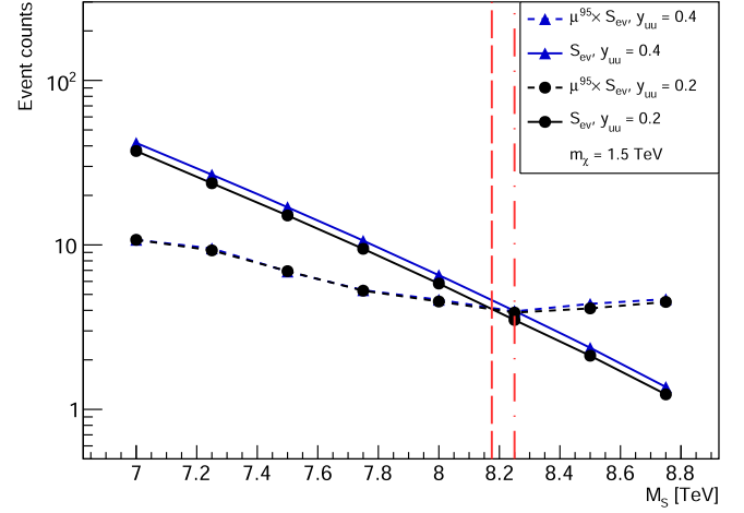
FIG. 4. 95% CL upper limits on \mu^{95} \times S_{\text{ev}} for \chi \rightarrow Wb , comparing y_{uu} = 0.2 and 0.4 at m_\chi = 1.5 TeV.
