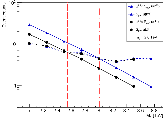
FIG. 7. 95% CL upper limits on \mu S_{ev} comparing \chi \rightarrow h^0 t and \chi \rightarrow Z t at y_{uu} = 0.2 and m_\chi = 2 TeV.
