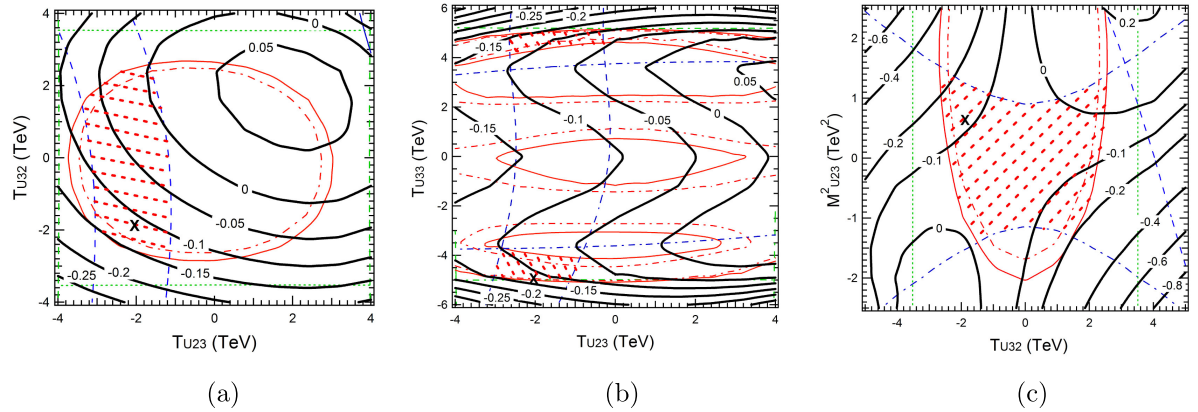
FIG. 8. Contour plots of \text{DEV}(\text{c}) around the benchmark point P1 in the parameter planes of (a) T_{U23} - T_{U32} , (b) T_{U23} - T_{U33} , and (c) T_{U32} - M_{U23}^2 . The parameters other than the shown ones in each plane are fixed as in Table II. The “X” marks P1 in the plots. The definitions of the red hatched regions and the bound lines are the same as those in Fig. 7.
