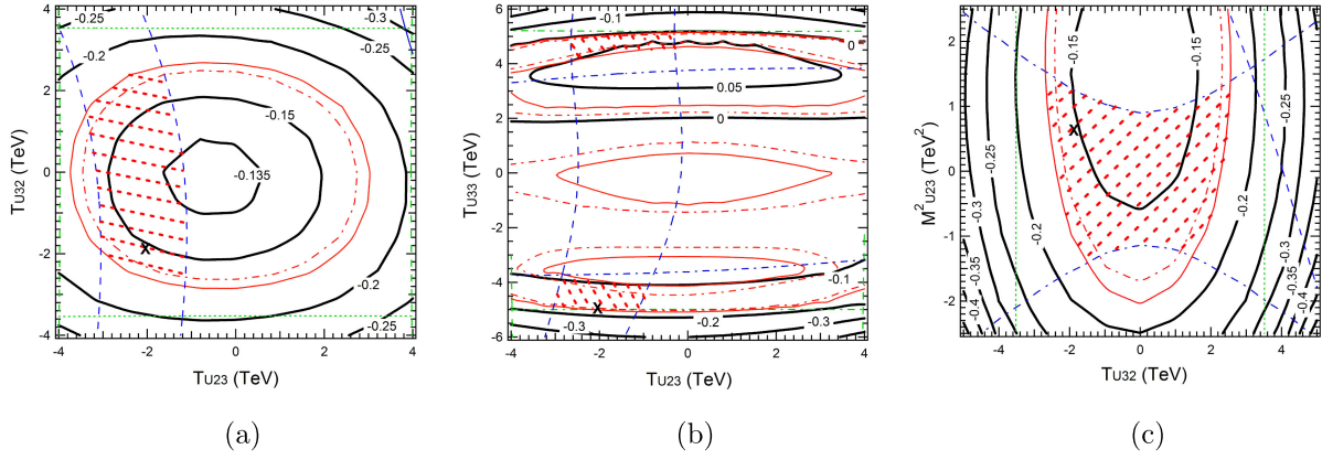
FIG. 7. Contour plots of \text{DEV}(\text{b}) around the benchmark point P1 in the parameter planes of (a) T_{U23} - T_{U32} , (b) T_{U23} - T_{U33} , and (c) T_{U32} - M_{U23}^2 . The parameters other than the shown ones in each plane are fixed as in Table II. The “X” marks P1 in the plots. The red hatched region satisfies all the constraints in Appendix A and also all the expected sparticle mass limits and (m_{A^0}, \tan \beta) limit at 95% CL from a negative search for sparticles and the heavier MSSM Higgs bosons H^0, A^0, H^\pm in the future HL-LHC experiments [43–49]. The red solid lines, green dashed lines, green dotted lines, green dash-dotted lines, blue solid lines, blue dashed lines, and blue dash-dotted lines show the m_{h^0} bound, vacuum stability bound for T_{U23} , T_{U32} , T_{U33} , B(b \rightarrow s\gamma) bound, B(B_s \rightarrow \mu^+\mu^-) bound, and m_{\tilde{u}_1} bound, respectively. Just for reference, the red dash-dotted lines show the m_{h^0} bounds for a hypothetical case that the total theoretical error is \pm 2 GeV instead of \pm 3 GeV; i.e., the contours of m_{h^0} (GeV) = 125.09 + (0.48 + 2) = 127.57 and m_{h^0} (GeV) = 125.09 - (0.48 + 2) = 122.61 . We see that only a small part of the red hatched region is excluded by this hypothetical m_{h^0} bounds.
