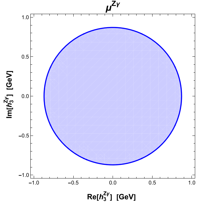
FIG. 3. Allowed region for the real and imaginary parts of the CP -violating form factor h_3^{Z\gamma} at the 95% CL, derived from the signal strength \mu^{Z\gamma} = 1.3_{-0.5}^{+0.6} reported by the ATLAS Collaboration [65].
