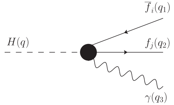
FIG. 2. Kinematic configuration and momentum assignments for the HZ\gamma vertex.
