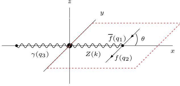
FIG. 6. Kinematic configuration and momentum assignments for the H \rightarrow \bar{f}f\gamma decay.
