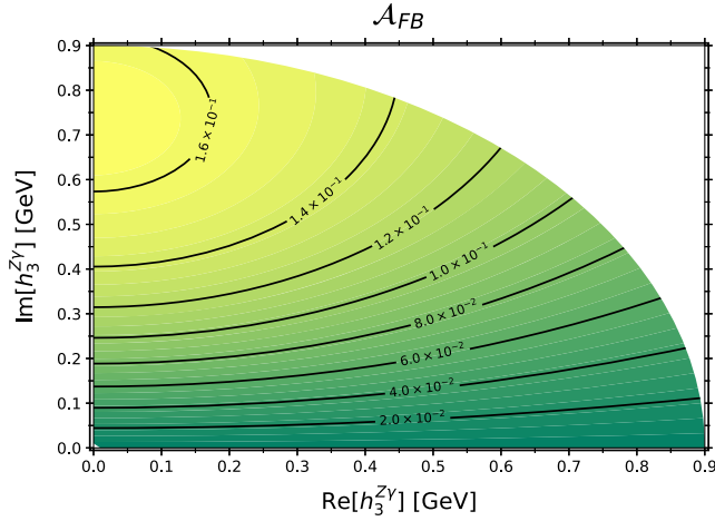
FIG. 5. Forward-backward asymmetry ( \mathcal{A}_{FB} ) in the allowed positive values of the real and imaginary parts of the CP -violating form factor h_3^{Z\gamma} .
