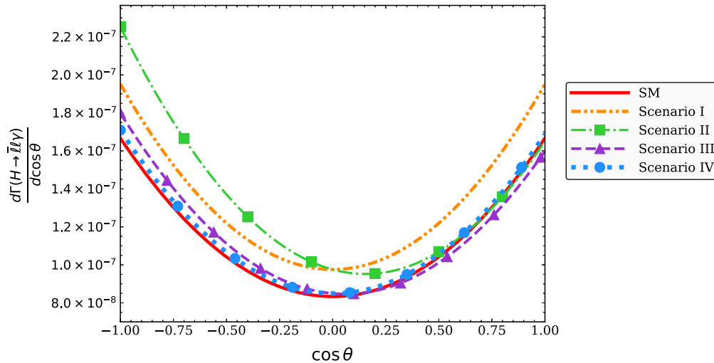
FIG. 4. Differential partial width of the H \rightarrow Z\gamma \rightarrow \bar{\ell}\ell\gamma decay as a function of \cos\theta for the SM and the benchmark scenarios defined in Table I. The CP -conserving form factor h_1^{Z\gamma} is fixed to its SM electroweak value.
