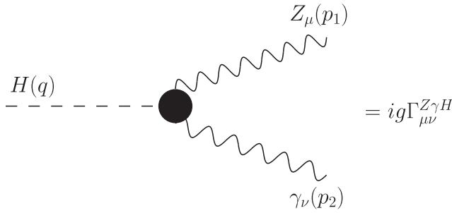
FIG. 1. The HZ\gamma vertex function. The Feynman diagrams in this work are created with JaxoDraw [38].
