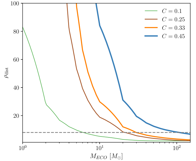
FIG. 6. Minimum detectable SNR that enables distinguishing an ECO merger signal from a BBH merger with matches obtained using PhenomDTaper. The gray dashed line shows the detectability threshold of 8. For masses \gtrsim 35M_{\odot} the distinguishability SNR is always lower than the detectability threshold for C \leq 0.33 .
