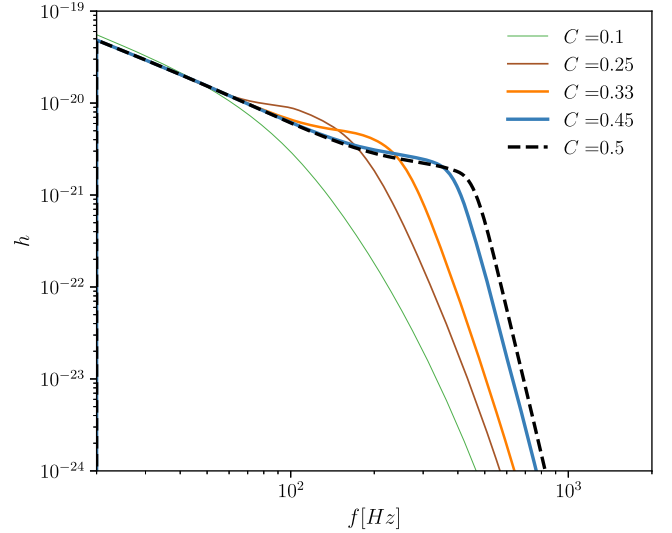
FIG. 3. Same as Fig. 2 with the amplitude parametrized by compactness. We show the amplitude for four different values of the compactness parameter, going from lower to higher values represented by progressively thicker lines. We also show that for C = 0.5 PhenomDECO reproduces the BBH amplitude as shown by the black dashed line.
