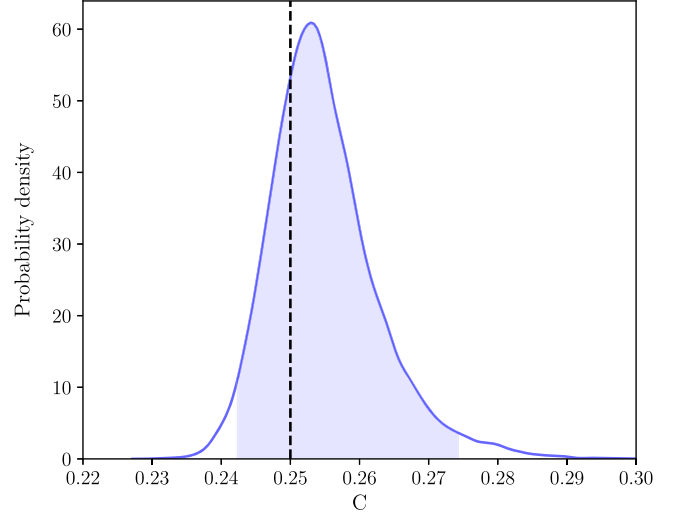
FIG. 9. Posterior probability distribution of compactness obtained using PhenomDECO as the recovery waveform, for an injected waveform generated with PhenomDECO at C = 0.25 .
