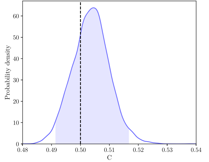
FIG. 8. Posterior probability distribution of compactness obtained using PhenomDECO as the recovery waveform, for an injected waveform generated with PhenomDECO at C = 0.5 .
