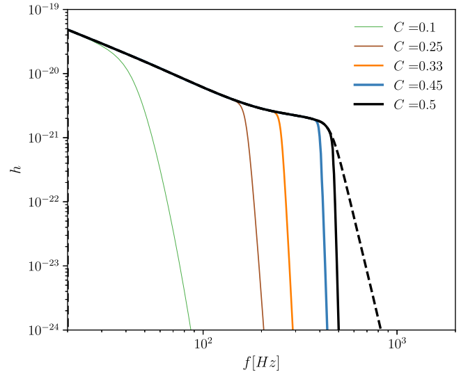
FIG. 2. Frequency domain amplitude from PhenomD for an equal-mass BBH of M_{\text{tot}} = 40M_\odot is shown in dashed black. Modified amplitude for ECO binaries of the same total mass with compactness C = 0.1, 0.25, 0.33, 0.45 are shown by lines of increasing thickness. Even at C = 0.5 (solid black line), the BBH amplitude is not fully reproduced.
