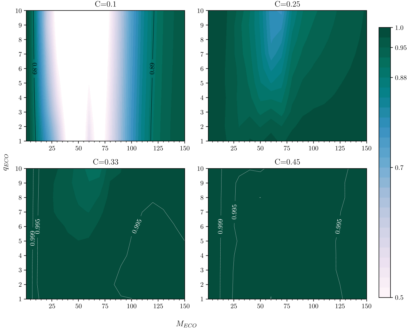
FIG. 5. Fitting factor contours obtained by optimizing the match between PhenomDTaper and PhenomD over the q - M - \chi_{\text{eff}} parameter space for different ECO total masses ( x axis) and mass ratio ( y axis); top left : C = 0.1 , top right : C = 0.25 , bottom left : C = 0.33 , bottom right : C = 0.45 and colour bar on right shows the value of the fitting factors. The black contours on the top left panel enclose the region of q - M space for nonspinning ECOs that would be interesting in residual tests, if such ECOs exist in nature.
