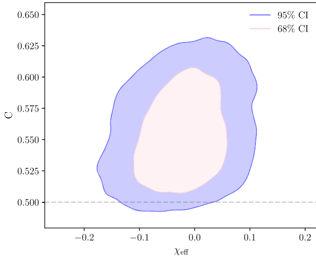
FIG. 11. Marginalized two-dimensional posterior probability distribution of compactness C and effective spin \chi_{\text{eff}} for GW150914 using PhenomDECO.
