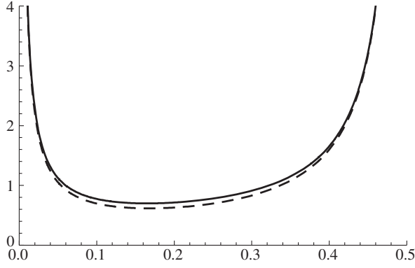
FIG. 1. Numerical comparison between -2iB_{2M}(1)/\lambda^2 (thick plot) and -2iB'_{2M}(1)/\lambda^2 (dashed plot) as functions of \delta = \gamma - 1/2 for 0 < \delta < 1/2 .
