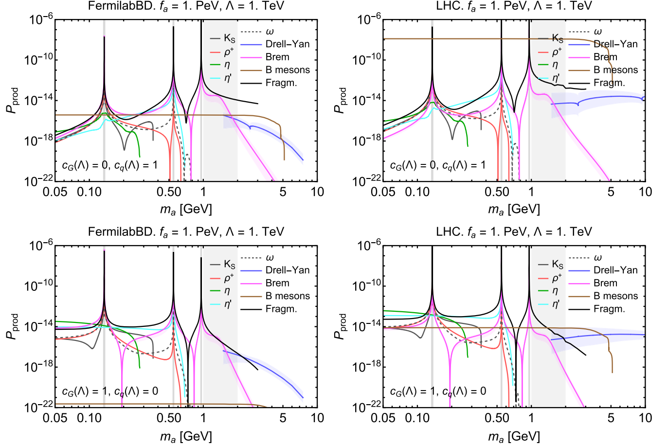
FIG. 7. Production probabilities of the axionlike particles at FermilabBD and LHC facilities. The ALP models are defined by the Lagrangian (8) at the scale \Lambda = 1 TeV, corresponding to the traditional choice in the literature [1,2,23]. Top panel: ALPs with the universal coupling to quarks [ c_q = 1 , c_G = 0 in Eq. (8)]. Bottom panel: ALPs coupled to gluons ( c_q = 0 , c_G = 1 ). The peaks are explained by the resonant contribution of the mixing with m^0 = \pi^0, \eta, \eta' mesons, whereas the dips are caused by the interference between these contributions and the direct interaction terms. The gray bands show the vicinities of the masses of m^0 where the description of phenomenology based on the mixing breaks down and the domain m_a \gtrsim 1 GeV where the description of the ALP phenomenology is incomplete due to lack of knowledge about excited pseudoscalar mesons (remind Sec. IV A).
