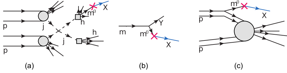
FIG. 2. Diagrams of various production channels of a particle X via the mixing with a neutral meson m^0 : the fragmentation of partons in the deep-inelastic collisions (a), decays of heavy mesons m' \rightarrow X + Y , with Y being some Standard Model state (b), and proton bremsstrahlung (c). The red cross indicates the mixing vertex.
