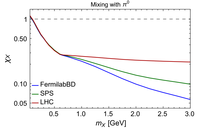
FIG. 3. The yield (31) of particles X mixing with \pi^0 produced per proton collision via the fragmentation and decays of secondary mesons, for various facilities—Fermilab Beam Dump (FermilabBD), SPS, and LHC. The yield is normalized by the amount of the corresponding mesons, which we report in Eq. (29). The quick decrease of the yield in the mass domain m_X \lesssim m_\rho is caused by closing secondary decays of heavier mesons ( \rho^0, \eta, \eta', \omega, K_S ) into X after reaching the kinematic threshold. Here and below, we use PYTHIA8 tunes are described in Sec. VA 1.
