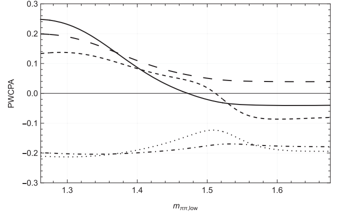
FIG. 1. Predictions of the quasinormalized PWCPAs A_{CP,l}|_{\eta_l=\eta_l^{(4)}} for B^\pm \rightarrow \pi^+ \pi^- \pi^\pm as a function of the invariant mass m_{\pi\pi, \text{low}} . The solid, dotted, dashed, dash-dotted, and long-dashed lines correspond to l = 0, 1, 2, 3 , and 4, respectively.
