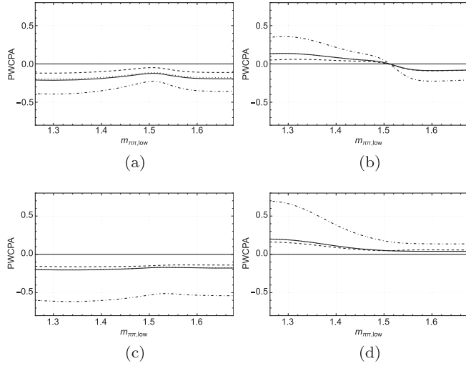
FIG. 2. Comparisons of various definitions of PWCPAs, where the solid, dotted, dashed, and dot-dashed lines correspond to A_{CP,l}|_{\eta_l=\eta_l^{(4)}} , A_{CP,l}|_{\eta_l=\tilde{\eta}_l} , \hat{A}_{CP,l} , and \hat{A}_{CP,l} , respectively. (a), (b), (c), and (d) correspond to l = 1, 2, 3 , and 4 , respectively. Note that A_{CP,l}|_{\eta_l=\eta_l^{(4)}} and A_{CP,l}|_{\eta_l=\tilde{\eta}_l} almost coincide with each other. The l = 0 case is not presented here because all the aforementioned four definitions of PWCPAs coincide for l = 0 , which are the same as the solid line in Fig. 1.
