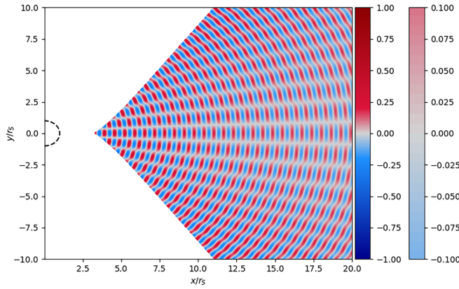
FIG. 4. Difference of oscillation probability \Delta P_{f \rightarrow f'} (charged minus uncharged) for a mass difference of 1%.
