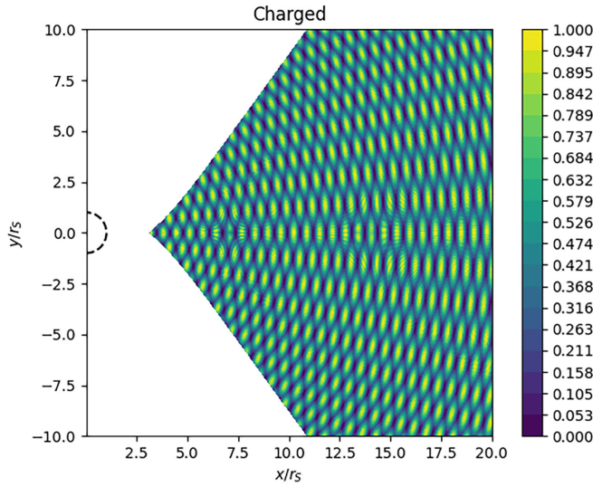
FIG. 3. Oscillation probability for a nearly maximal charge r_Q = 0.49r_S and a mass difference of 1%.
