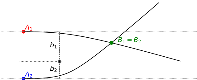
FIG. 2. Four phases interfere at the intersection point after scattering; two flavors on each trajectory.
