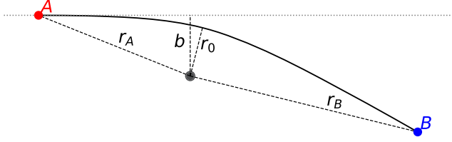
FIG. 1. The source is located at the point A, at the distance r_A from the compact object, and the detector is located at the point B, at the distance r_B from the compact object. b is the impact parameter and the closest approach distance is denoted by r_0 .
