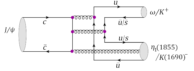
FIG. 1. A schematic diagram for J/\psi decaying into a light meson ( \omega/K ) and a hybrid state [ \eta_1(1855)/K(1690) ].
