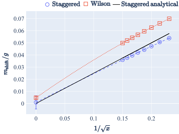
FIG. 4. Additive mass renormalization m_{\text{shift}}/g as a function of the lattice spacing 1/\sqrt{x} , extracted from the zero crossing of the electric field density for staggered and Wilson fermions. Dashed lines indicate quadratic continuum extrapolations. The solid black line represents the analytical prediction for staggered fermions with periodic boundary conditions from Ref. [46].
