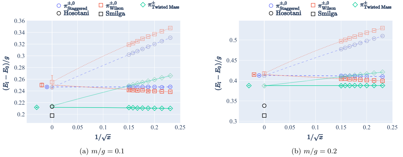
FIG. 6. Scaling behavior of the energy gap (E_l - E_0)/g of the pion for the three different fermion discretizations. Faint lines show quadratic fits to the data obtained at fixed lattice mass, while bold lines show purely quadratic fits for data at fixed renormalized mass. As in previous figures, some of the extrapolated values are offset from zero for clarity. Analytical estimates from Ref. [49] (Hosotani) and Ref. [48] (Smilga) for the pion mass are included for comparison. Note that the energy gap does not directly correspond to the pion mass without accounting for additional systematic effects.
