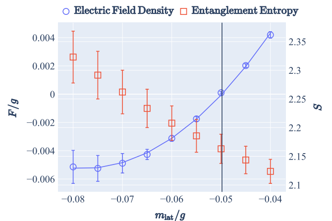
FIG. 3. Electric field density F/g and entanglement entropy S as functions of the lattice mass m_{\text{lat}}/g for Wilson fermions at the smallest lattice spacing 1/\sqrt{x} = 0.15 . The first zero crossing of F/g , indicated by the black vertical line, can be used to determine the additive mass renormalization on the lattice.
