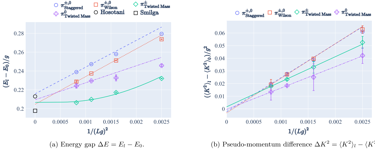
FIG. 9. Finite-volume scaling of energy gaps (a) and pseudo-momentum differences (b) at fixed renormalized mass m_\pi/g = 0.1 . Lines show fits in 1/Lg : a quadratic fit is used for staggered and Wilson fermions and for the neutral pion in the twisted mass formulation, while an exponential fit is applied for the charged pion in the twisted mass case. The infinite-volume extrapolations are compared to analytical predictions for the pion mass from Refs. [48,49]. The momentum gap extrapolates to zero, as expected.
