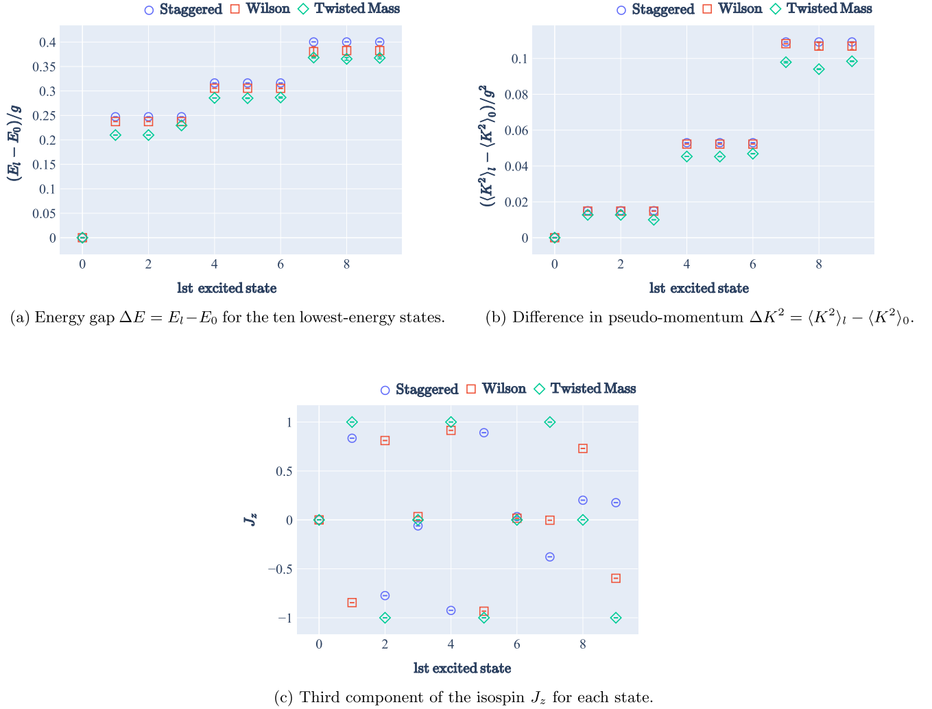
FIG. 7. Key observables for the ten lowest-energy states of the massive two-flavor Schwinger model, computed using a variational ground state search with staggered, Wilson, and twisted mass fermions. Panels show (a) the energy gap relative to the ground state, (b) the pseudo-momentum gap, and (c) the third component of the isospin J_z . The explicit isospin breaking in the twisted mass formulation gives rise to distinct features, which are discussed in the main text.
