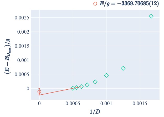
FIG. 1. Convergence of the ground state energy for twisted mass fermions at maximal twist as a function of bond dimension D , for N = 200 , Lg = 30 , and \mu/g = 0.1 . Shown is the difference between the computed energy at a given bond dimension and the value at the maximum bond dimension D_{\max} . The final extrapolated value is indicated by a red circle, with its numerical value shown in the legend.
