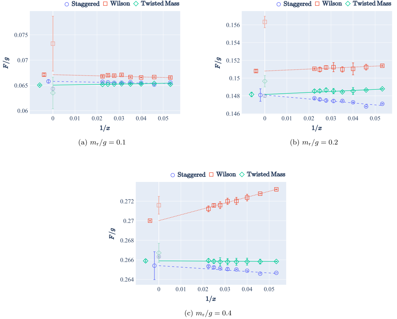
FIG. 5. Scaling behavior of the electric field density F/g at fixed renormalized mass m_r/g . Bold lines indicate purely quadratic fits for all three fermion discretizations; the continuum extrapolation points are again horizontally offset for clarity. Faint markers show the previously obtained extrapolations at fixed lattice mass. Note the significantly smaller y-axis scale compared to Fig. 2.
