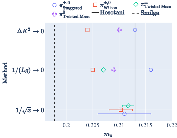
FIG. 11. Pion mass results from various fermion discretizations and extraction methods for fermion mass m/g = 0.1 . Shown (from top to bottom) are results from dispersion relation fits at fixed lattice spacing 1/\sqrt{x} = 0.273 and fixed volume Lg = 30 ; finite-volume scaling results at the same lattice spacing; and continuum extrapolations performed in the thermodynamic limit. Horizontal lines indicate analytical predictions from Refs. [48,49]. The charged pion mass from the dispersion relation for twisted mass fermions lies well below the plot range at m_\pi/g = 0.171 .
