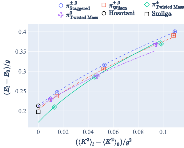
FIG. 8. Dispersion fits at finite lattice spacing for the three fermion discretizations, using excitation energy and pseudo-momentum estimates. Staggered and Wilson fermions yield degenerate pion states, while twisted mass fermions show isospin splitting due to lattice artifacts. Extrapolations to zero momentum are compared to analytical predictions for the pion mass from Refs. [48,49].
