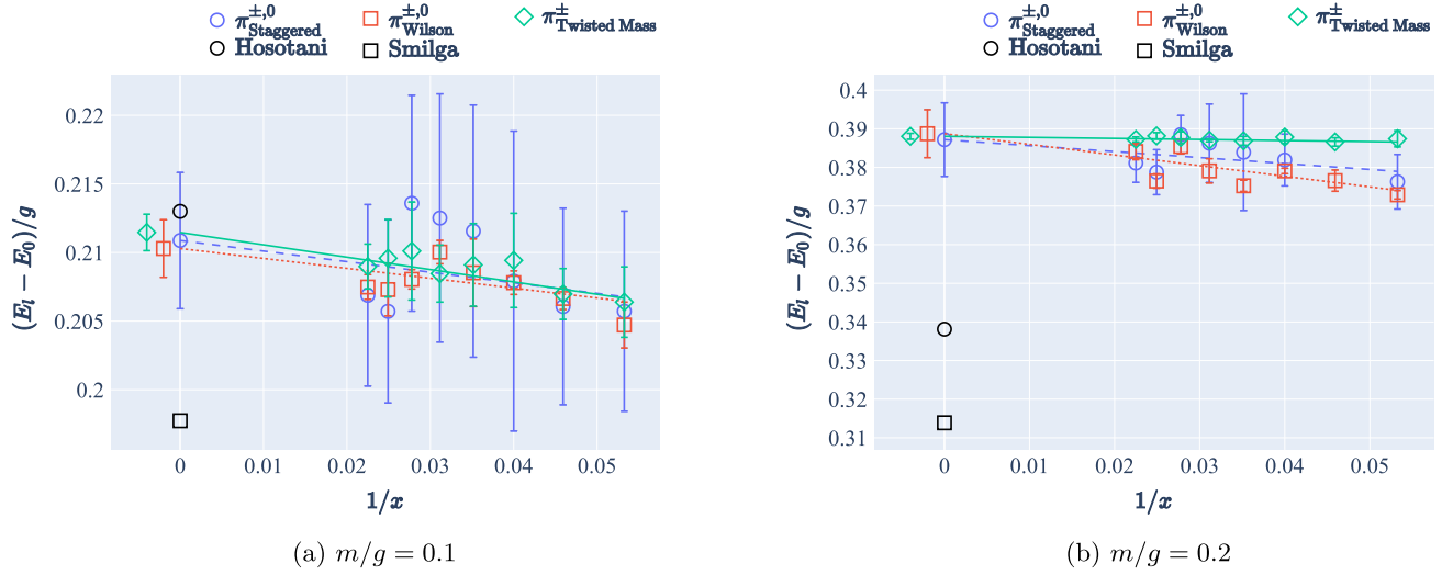
FIG. 10. Combined continuum and finite-volume extrapolation of the pion mass for staggered, Wilson, and twisted mass fermions, including mass renormalization. Each data point represents a volume-extrapolated result at fixed lattice spacing, obtained from simulations at Lg = 20 - 35 . The continuum limit is extracted via a purely quadratic fit in 1/\sqrt{x} . Analytical predictions from Refs. [48,49] are shown for comparison.
