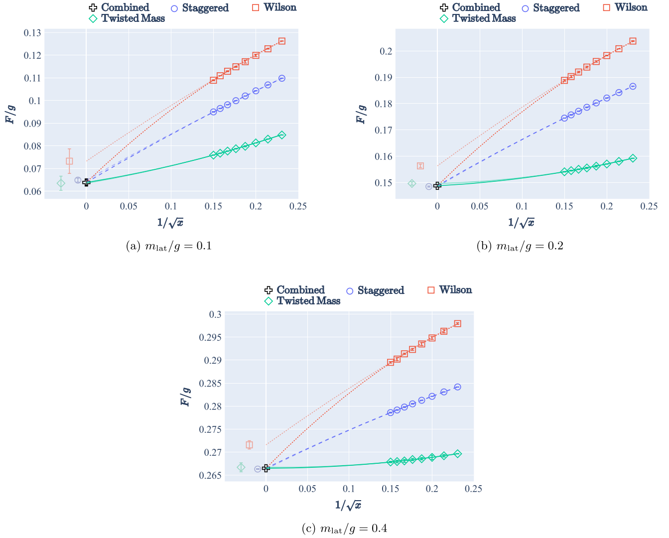
FIG. 2. Scaling behavior of the electric field density F/g as a function of the lattice spacing 1/\sqrt{x} . Faint lines show individual quadratic fits for each fermion discretization, while bold lines represent the combined fit with a shared continuum limit. The continuum extrapolation points from the individual fits are horizontally offset from zero for better visibility.
