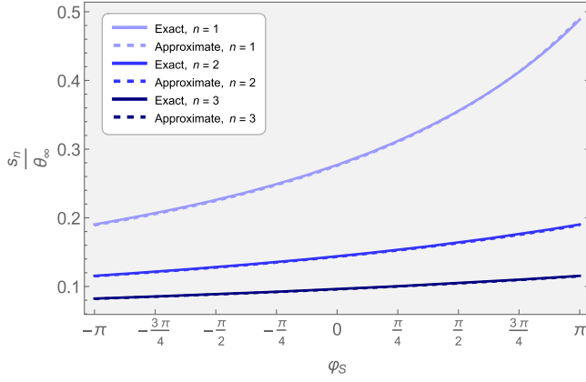
FIG. 3. Relative angular position of the first three higher-order images for an extremal Kerr black hole. The horizontal axis is the source azimuth \varphi_S , while the vertical axis shows the image angular separation from the shadow edge, normalized by \theta_\infty . Each curve corresponds to a certain n (number of loops executed around the black hole before reaching the observer), so that n = 1 is the outermost member of the image sequence and larger n accumulate toward \theta_\infty . As indicated in the legend, the solid curves represent the approximate results, see Eq. (62), while the dashed curves represent the exact results, see Eq. (65).
