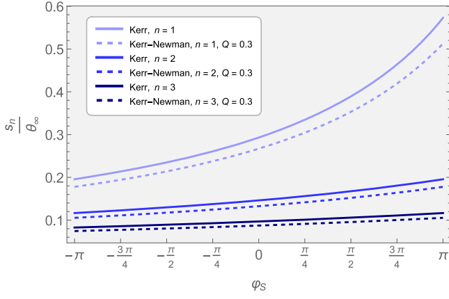
FIG. 6. Relative angular position of the first three higher-order images for extremal Kerr and Kerr-Newman black holes. Each curve corresponds to a certain n .
