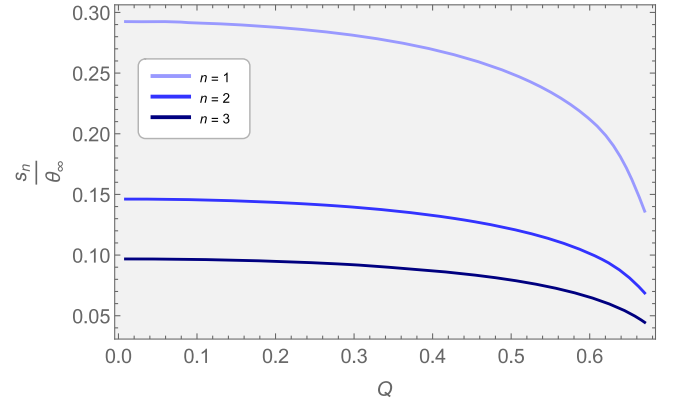
FIG. 10. Relative angular position of the first three higher-order images for extremal Kerr-Sen as a function of the charge Q . We set \varphi_S = 0 .
