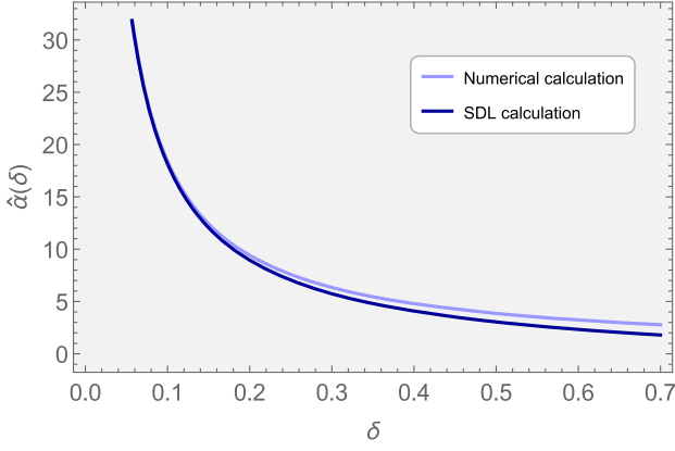
FIG. 2. Deflection angle for equatorial prograde photon trajectories in the extremal Kerr spacetime, shown as a function of \delta . The light blue curve is the result of a numerical calculation, while the dark blue curve is the analytic strong deflection limit approximation, labeled SDL in the legend, given by Eq. (51). As expected, for small values of \delta , the SDL curve agrees well with the numerical result.
