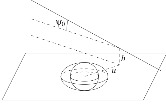
FIG. 11. Geometrical parametrization of an incoming quasiequatorial photon trajectory in the asymptotically flat region. The parameter u is the minimum distance between the black hole and the projection of the asymptotic trajectory onto the equatorial plane. The quantity h is the height of the photon above or below the equatorial plane at that point, while \Psi_0 is the inclination angle of the asymptote with respect to the equatorial plane. Reproduced from Ref. [24].
