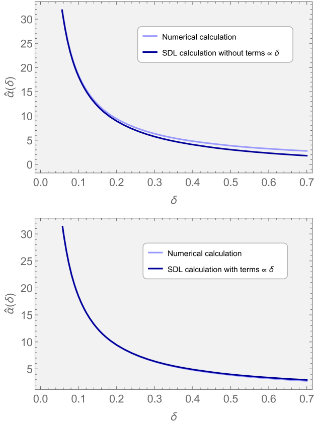
FIG. 4. Comparison between the exact deflection angle, computed numerically, and its strong deflection limit approximation (labeled SDL in the legend). We show both the SDL expression retaining only the 1/\delta , \log \delta , and constant terms (dark blue curve, top panel), and the improved SDL including the next-to-leading corrections (dark blue curve, bottom panel).
