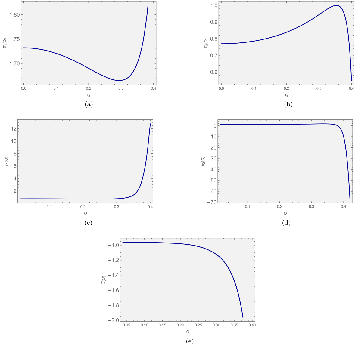
FIG. 5. Dependence of the strong-deflection-limit coefficients on the charge Q for an extremal KerrNewman black hole. The panels show (a) \bar{\alpha}_1 , (b) \bar{\alpha}_2 , (c) \bar{c}_1 , (d) \bar{c}_2 , and (e) \bar{b} as functions of Q .
