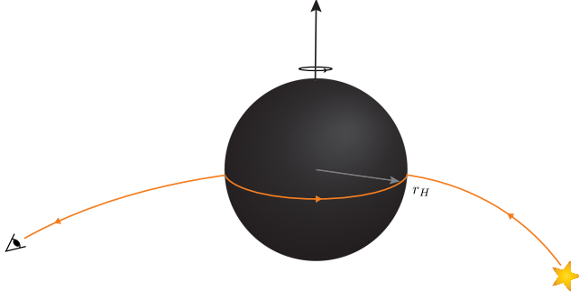
FIG. 1. Schematic representation of the extremal prograde lensing configuration considered in this work. The black surface denotes the degenerate event horizon, whose radius r_H coincides with the critical radius of the prograde circular photon orbit. The orange curve represents a photon trajectory in the equatorial plane that winds close to the horizon before escaping to a distant observer.
