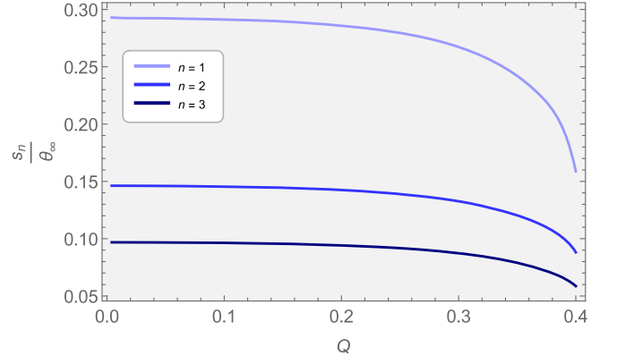
FIG. 7. Relative angular position of the first three higher-order images for extremal Kerr-Newman as a function of the charge Q . We set \varphi_S = 0 .
