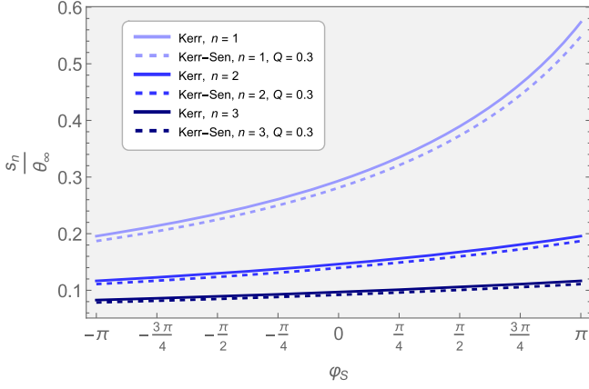
FIG. 9. Relative angular position of the first three higher-order images for extremal Kerr and Kerr-Sen black holes. Each curve corresponds to a certain n .
