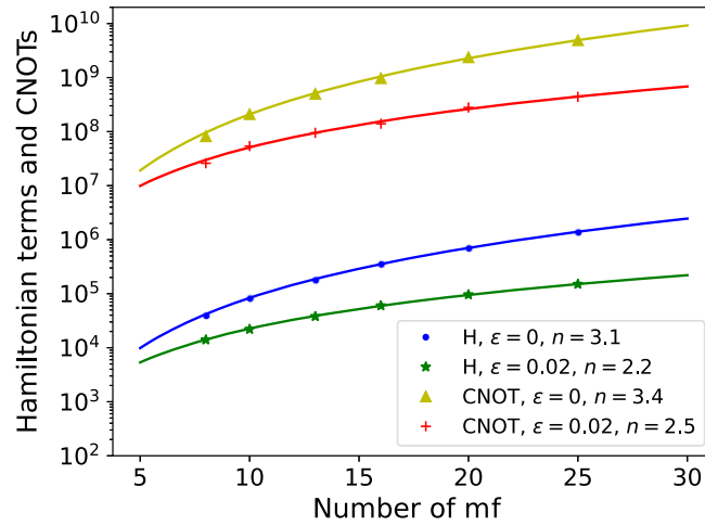
FIG. 6. Summary scaling of the number of Hamiltonian terms (lower two lines) and total count of CNOT gates (upper two lines) with the number of encoded z momentum fractions (mf). We also show the sensitivity to whether a cutoff on the Hamiltonian matrix element module |V| \geq \epsilon|V_{\max}| is (or is not, by setting \epsilon = 0 ) applied. The scaling is polynomial with the exponent n indicated in the legend.
