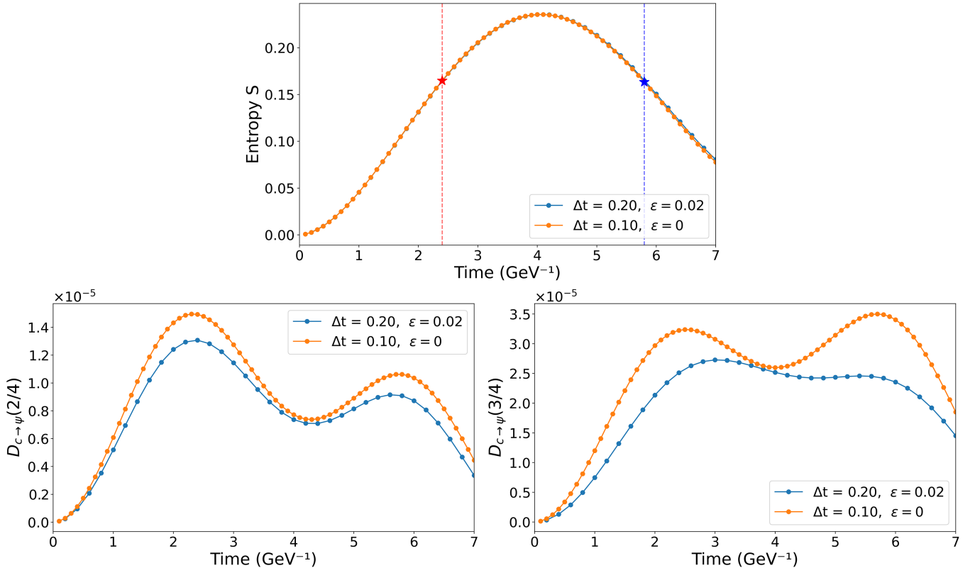
FIG. 9. Shannon entropy (upper plot) and fragmentation functions at z = 2/4 (lower left) and z = 3/4 (lower right) as functions of evolution time for different values of the Hamiltonian matrix element size cutoff \epsilon . Parameters correspond to configurations 2 and 3 of Table V with \Delta t as indicated in the legends. As can be seen, with our modest number of modes, the fragmentation function still shows oscillations with time which one would expect to be more damped should one have access to a larger quantum memory allowing for further particles and longitudinal momentum partitions.
