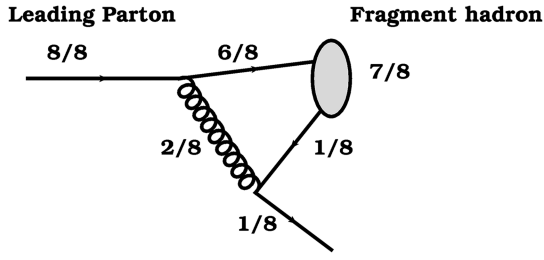
FIG. 3. Illustration of the maximum momentum carried by the fragmented meson. The initial parton, taken here to be a c quark, must divide its momentum at the first splitting. The gluon then becomes a quark-antiquark pair, each with the minimum momentum representable in the grid ( z = 1/8 ). This means that the maximum momentum fraction carried by the meson is z = 7/8 .
