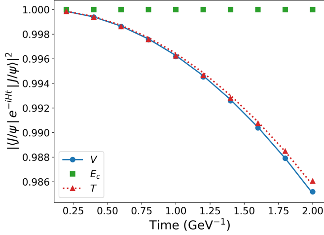
FIG. 10. Data points: plot of |\langle U \rangle|^2 in the J/\psi variational state of Eq. (9) from the simulation, for various pieces of the Hamiltonian (free only, E_c ; V vertices only, V ; total Hamiltonian, T ). The calculation is conducted for the SU(2) group and a grid of four momentum points. The quark and antiquark momenta add up to z = 3/5 . Lines: quadratic fit as per Eq. (E3), yielding \Delta E = \sqrt{-a} \simeq 61 MeV.
