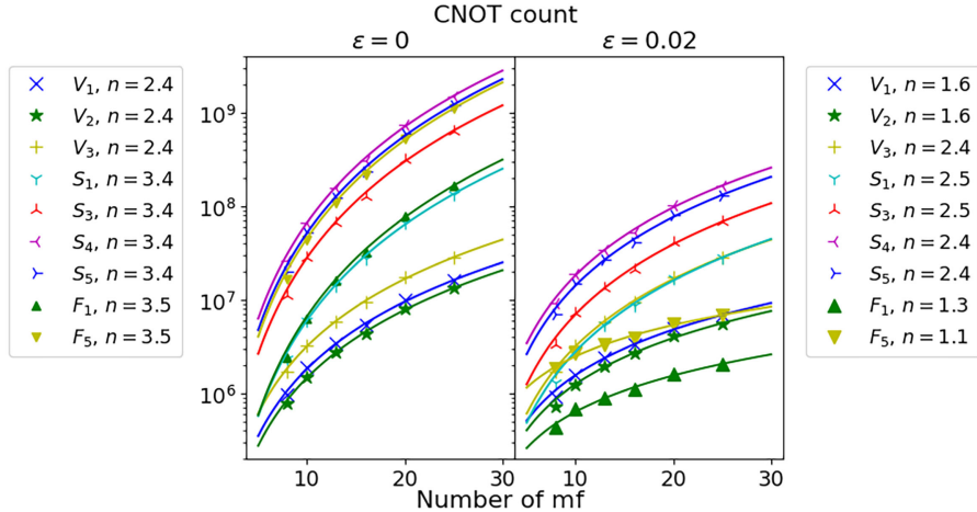
FIG. 5. Scaling with the number of encoded momentum fractions (mf) of the number of CNOT gates needed to account for all the possible momentum modes affecting each of the indicated terms of the Hamiltonian. The right plot forces an infrared cutoff to the potential matrix elements, with |V| \geq \epsilon|V_{\max}| , with \epsilon = 0.02 , while the computation of the left plot is conducted with \epsilon = 0 and thus is only cut off by the grid's volume. The exponents n of the polynomial-scaling law are also given in the legends. The \epsilon size cutoff barely affects the term V_3 whose scaling with N is not modified.
