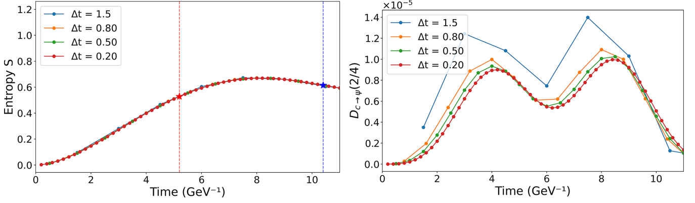
FIG. 8. Shannon entropy (left) and fragmentation function at z = 2/4 (right) as functions of evolution time for different values of the time-step size. Parameters correspond to configuration 1 of Table V. Good convergence with the Trotter time step \Delta t can be appreciated.
