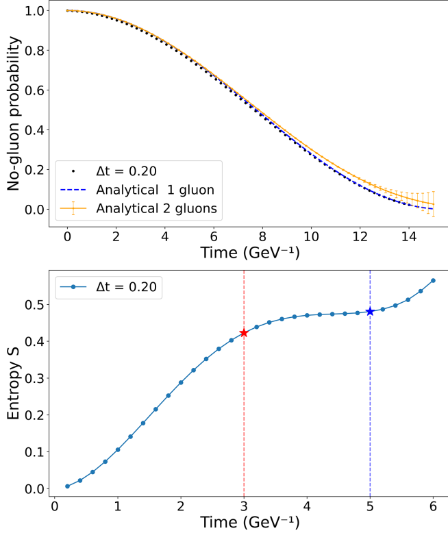
FIG. 1. SU(2) simulation with up to four particles in an (N = 8) k^+ grid. Upper plot: the probability (vs time) for an initial c quark with maximum grid momentum to not be accompanied by a bremsstrahlung gluon for H restricted to V_1 interactions with a simulated quantum memory able to hold one or two gluons. Lower plot: the entropy S(t) increases with the average number of modes populated by radiation from the initial parton for H restricted to the kinetic terms and V interactions. Ideally, D_j^h is to be extracted around saturation (maximum entropy); given that errors (upper plot) increase with time, we extract it when a plateau is found (between the red and blue vertical lines).
