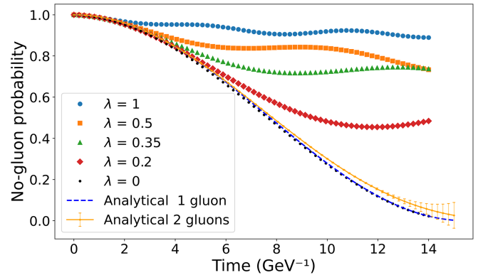
FIG. 7. Probability that an initial quark with maximum longitudinal momentum is not accompanied by a gluon when it evolves under \exp\{-i\Delta t(V_1 + \lambda E_c)\} . Also plotted is the analytically tractable prediction of Eq. (E1) for the extreme case of \lambda = 0 . The first minimum of the physical \lambda = 1 curve sets the time at which fragmentation functions are measured. This is of interest for the systematic uncertainty induced by the truncation of the Fock space to a finite number of particles.
