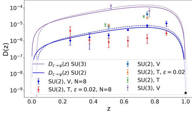
FIG. 2. Fragmentation function of a c quark to a J/\psi meson. T denotes the total Hamiltonian ( V the vertex-type terms only); the k^+ momentum lattice size is set to N = 4 (or N = 8 if indicated). The reference lines are the NRQCD computation at leading order [21] and next-to-leading order [22] (dashed). The symbols stem from our classical simulation of what the quantum computer would find, as in Fig. 1, for various J/\psi momentum fractions z . The uncertainty raisers span only the time interval for D extraction (lower plot of Fig. 1). By construction of the numerical grid, the end-point value D(1) = 0 vanishes as it must.
