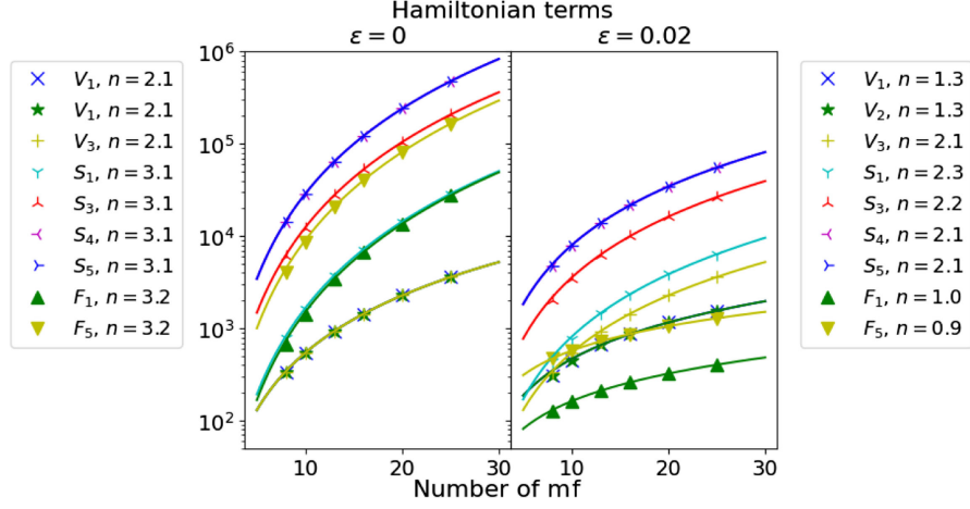
FIG. 4. Scaling of the number of Hamiltonian terms of each type (potential V , fork F , seagull S ) with the number of encoded momentum fractions (mf), fitting the n exponent of Eq. (D1). The right plot only includes interactions with |V| \geq \epsilon|V_{\max}| , with \epsilon = 0.02 , to save computational time from terms of size below the noise level. The dominating polynomial-scaling exponents n are indicated. The \epsilon size cutoff barely affects the term V_3 whose scaling with N is not modified, because it tends to be numerically large. For other terms there can be substantial gains in execution times.
