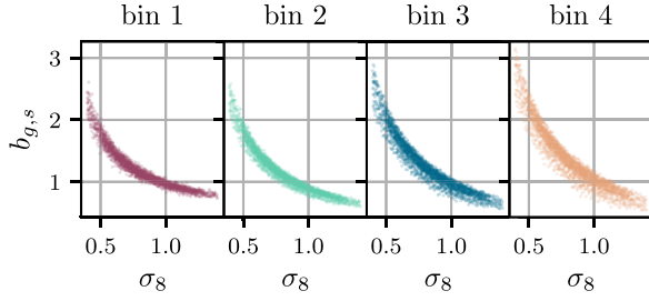
FIG. 5. Scatter plot depicting the source galaxy bias b_{g,s} we find for the 2500 unique cosmologies of the COSMOGRIDV1 by fitting the source galaxy number count histogram to a reference BUZZARD simulation of fixed cosmology.
