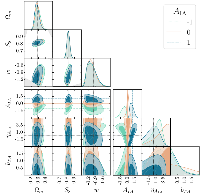
FIG. 25. Marginal posterior probability densities for COSMOGRIDV1 internal mocks of varying intrinsic alignment amplitude A_{IA} . For the intrinsic alignment parameters, the axis limits mark the prior boundaries from Table I. In all cases, the inference pipeline accurately recovers the true parameters.
