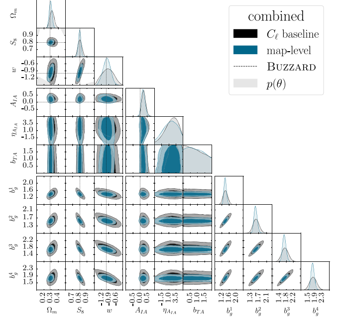
FIG. 21. Like Fig. 12 combined, but for all parameters.
