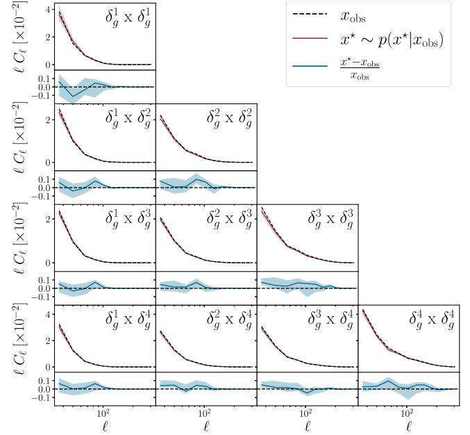
FIG. 9. Comparison between the power spectrum of one BUZZARD simulation (dashed line) to samples from the PPD [see Eq. (20)] derived from map-level galaxy clustering analysis. The solid lines show the mean of the posterior predictive samples, and the shaded regions indicate the 95% credible interval.
