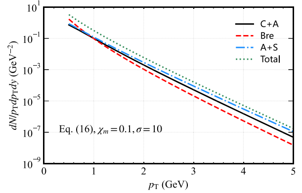
FIG. 8. Hard thermal photon spectrum as a function of transverse momentum p_T for the C + A, bremsstrahlung (Bre), A + S channels, and total yield, calculated with \chi_m = 0.1 , \sigma = 10 , and MHD solution.
