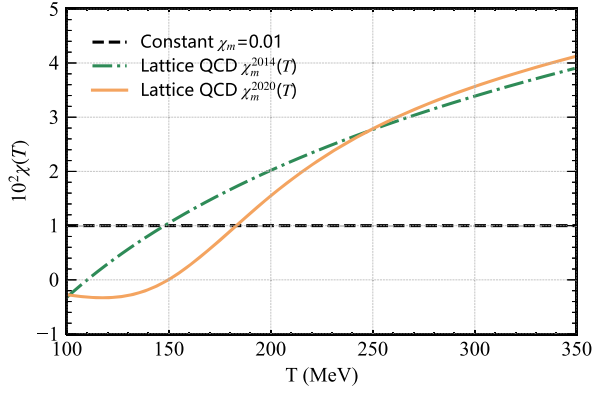
FIG. 3. Temperature dependence of the magnetic susceptibility \chi_m(T) for three prescriptions: constant \chi_m = 0.01 , the 2014 lattice QCD result [Eq. (21)], and the 2020 lattice QCD parametrization [Eq. (22)], over 100 \leq T \leq 350 MeV.
