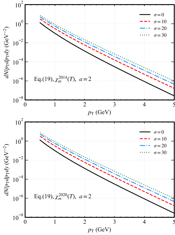
FIG. 11. Total thermal photon production spectra as a function of transverse momentum. Upper panel: results with \chi_m^{2014}(T) for \sigma = 0, 10, 20, 30 and a = 2 . Lower panel: results with \chi_m^{2020}(T) for the same \sigma and a = 2 .
