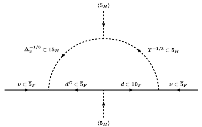
FIG. 3. One-loop neutrino mass generating diagram in the 15_H extension, when the SU(5) symmetry breaking is accomplished with representations 24_H and 5_H .
