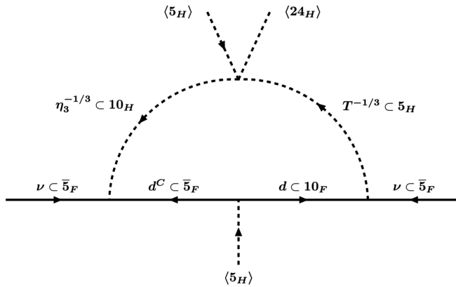
FIG. 2. One-loop neutrino mass generating diagram within the 10_H extension, when the SU(5) symmetry breaking is accomplished with representations 24_H and 5_H .
