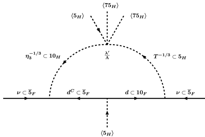
FIG. 4. One-loop neutrino mass generating diagram in the 10_H extension, when the SU(5) symmetry breaking is accomplished with representations 75_H and 5_H .
