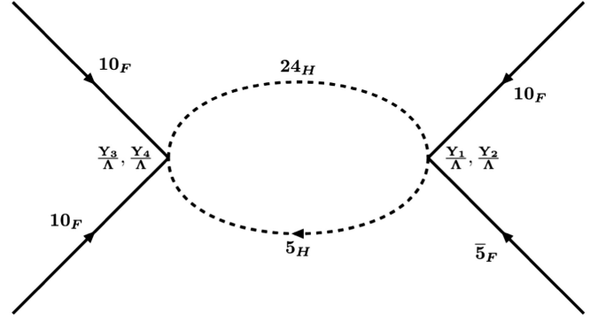
FIG. 1. One-loop level proton decay inducing diagram that utilizes d = 5 operators at each vertex, as indicated.
