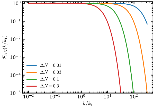
FIG. 1. Finite-duration transfer kernel associated with a smooth hyperbolic tangent mass transition. The instantaneous approximation is recovered in the unresolved regime k\Delta N/k_1 \ll 1 , whereas modes that resolve the internal transition structure are exponentially filtered.
