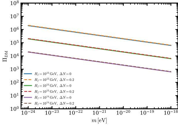
FIG. 6. Impulse strength required for the longitudinal vector sector to account for the full observed dark matter abundance, obtained from Eq. (59). Solid curves correspond to the sharp-transition approximation, while dashed curves include finite-duration effects with \Delta N = 0.2 .
