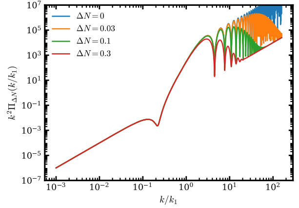
FIG. 4. Dimensionless longitudinal spectral shape k^2\Pi_{\Delta N}(k/k_1) for impulse strength \Pi = 30 . Finite transition duration preserves the enhanced non-slow-roll amplification while removing the ultraviolet oscillatory structure inherited from the instantaneous approximation.
