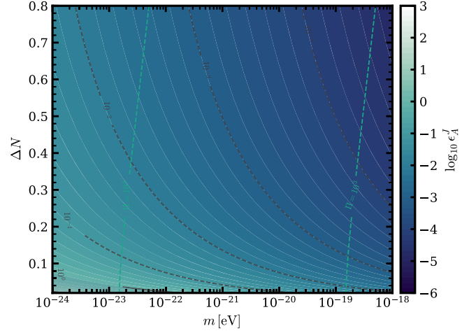
FIG. 16. Derivative-sensitive transition-stress constraint evaluated for H_I = 10^{14} GeV. The quantity \epsilon_A^J estimates the stress scale associated with varying J over a finite interval \Delta N . The figure identifies the region where the sector generating the time-dependent vector mass contributes non-negligibly to the inflationary energy budget.
