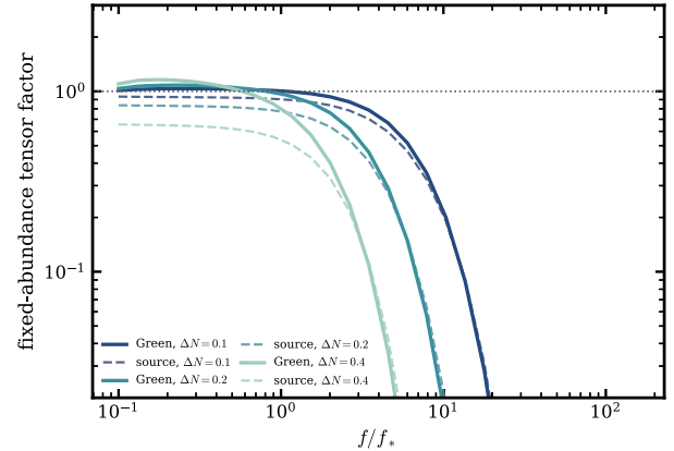
FIG. 14. Finite-width tensor calculation including an explicit radiation-era retarded Green's-function integration. Solid curves show the fully time-integrated tensor calculation including the Green's kernel and radiation-era transfer functions, while dashed curves retain only the source convolution. Both calculations incorporate the same finite-width filtering on the two vector spectra after imposing the relic abundance constraint.
