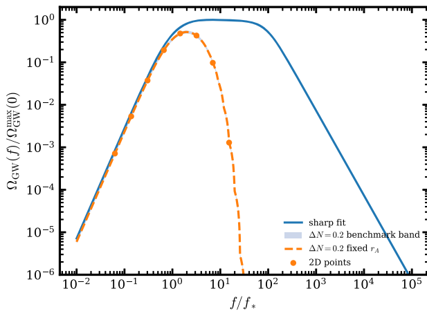
FIG. 9. Induced gravitational-wave spectrum as a function of f/f_* normalized relative to the sharp-transition r_A = 1 amplitude. The dashed curve and points correspond to the \Delta N = 0.2 transverse-traceless source integration, while the shaded region denotes the finite-width source-kernel uncertainty interval.
