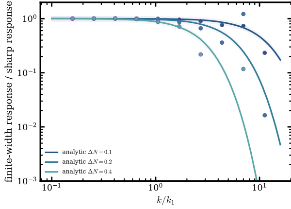
FIG. 12. Numerical validation of the finite-width envelope approximation. Points correspond to direct numerical solutions of Eq. (77) in the small-impulse regime normalized against a narrow-transition reference solution. Solid curves denote the analytic prediction \mathcal{F}_{\Delta N}^2 , while the shaded region indicates ten percent deviations.
