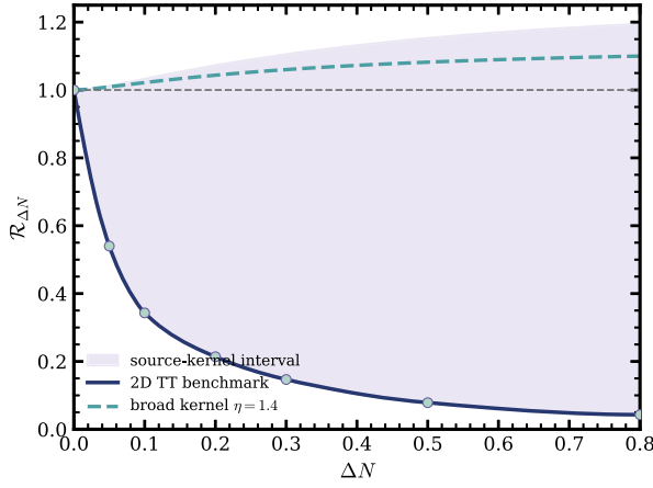
FIG. 8. Residual tensor-shape factor \mathcal{R}_{\Delta N} = \mathcal{C}_{\Delta N} / \mathcal{A}_{\Delta N}^2 evaluated after imposing fixed relic abundance. The shaded band indicates the source-level interval bounded by the broad positive kernel and the full transverse-traceless numerical calibration. The points denote the discrete transverse-traceless calibration values used in normalizing the finite-width gravitational-wave predictions.
