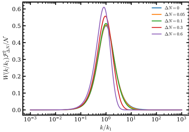
FIG. 7. Momentum-space contribution to the abundance integral. Finite transition duration shifts the dominant support away from modes that fully resolve the transition, thereby reducing sensitivity of the relic-density calculation to the ultraviolet structure present in the sharp-transition spectrum.
