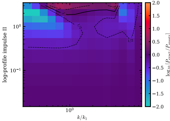
FIG. 13. Finite-impulse mode diagnostic for a resolved logarithmic transition with width \Delta N = 0.2 . The color scale denotes the exact numerical mode power divided by the smooth impulse approximation. The labeled contours indicate factors of two and separate the controlled impulse regime from the nonlinear resolved mass-ramp region where the q_N^2 contribution becomes dynamically significant.
