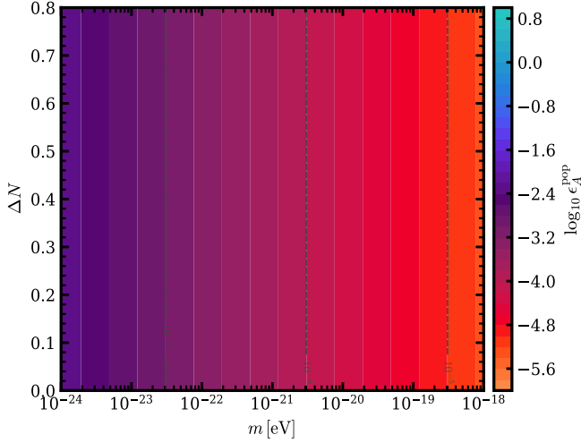
FIG. 15. Spectator-sector population constraint for the relic-density-saturating case r_A = 1 at H_I = 10^{14} GeV. Contours indicate the parameter \epsilon_A^{\text{pop}} after imposing the abundance constraint. The physically allowed spectator regime corresponds to \epsilon_A^{\text{pop}} \ll 1 .
