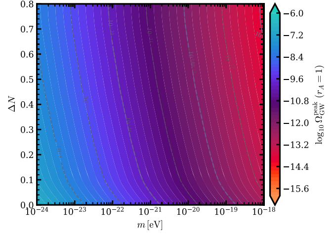
FIG. 10. Peak gravitational-wave energy density after imposing relic-density saturation for the vector dark matter component, corresponding to r_A = 1 . The vector mass determines the characteristic frequency through Eq. (62), while finite-duration effects enter through the residual source-shape factor \mathcal{R}_{\Delta N} .
