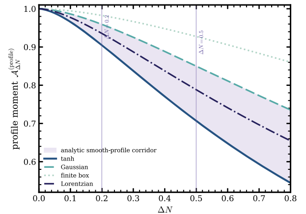
FIG. 3. Dependence of the abundance moment on the choice of transition profile. The shaded band represents smooth analytic transition families, while the solid curve corresponds to the hyperbolic tangent profile used in the main numerical analysis. The instantaneous limit is recovered for \Delta N \rightarrow 0 for all normalized smooth profiles.
