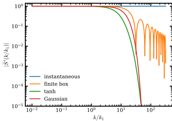
FIG. 2. Comparison of profile-transform envelopes for transitions sharing the same characteristic width. Instantaneous transitions exhibit no ultraviolet suppression, finite box profiles generate oscillatory power-law behavior, while analytic profiles such as hyperbolic tangent or Gaussian transitions suppress high resolved modes exponentially or faster.
