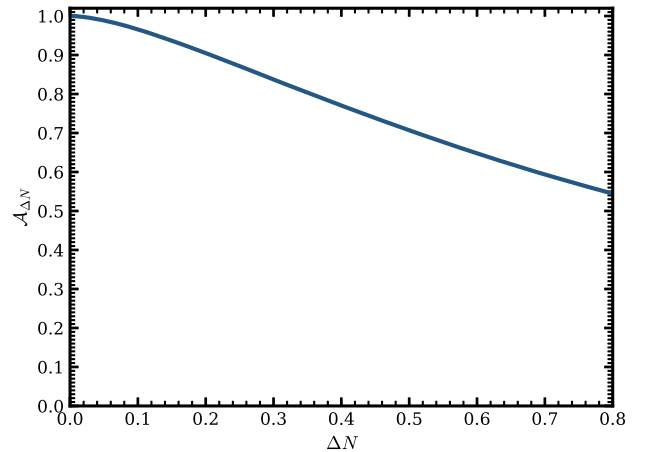
FIG. 5. Profile-dependent abundance moment \mathcal{A}_{\Delta N} entering the relic-density integral, computed from Eq. (53). The sharp-transition normalization is recovered for \Delta N \ll 1 , while increasing transition duration produces a smooth monotonic suppression of the abundance contribution.
