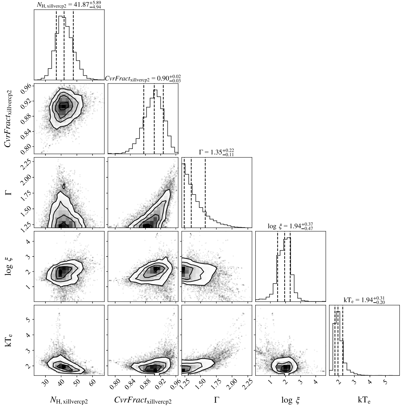
FIG. 12. Corner plot for the free parameter pairs for interval 8 after the MCMC run.
