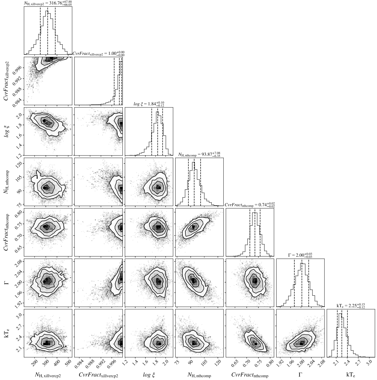
FIG. 11. Corner plot for the free parameter pairs for interval 5 after the MCMC run.
