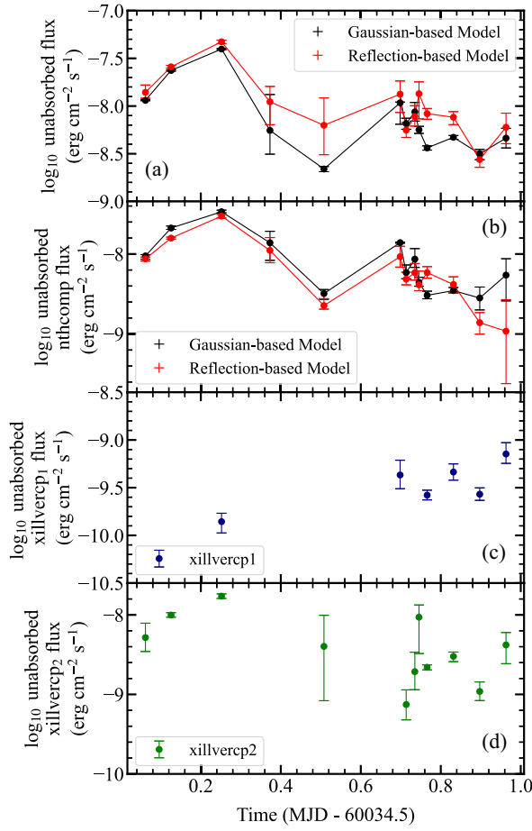
FIG. 7. Evolution of the unabsorbed flux for two different models. Fluxes are measured by cflux in XSPEC. The Gaussian-based model is shown in black, and the reflection-based model is in red. (a) Total unabsorbed flux. Total flux of reflection-based model is calculated from cflux of the other components. (b) Unabsorbed flux of the continuum component nthcomp . (c) Unabsorbed flux of the neutral reflection component xillvercp1 (in blue). (d) Unabsorbed flux of the ionized reflection component xillvercp2 (in green).
