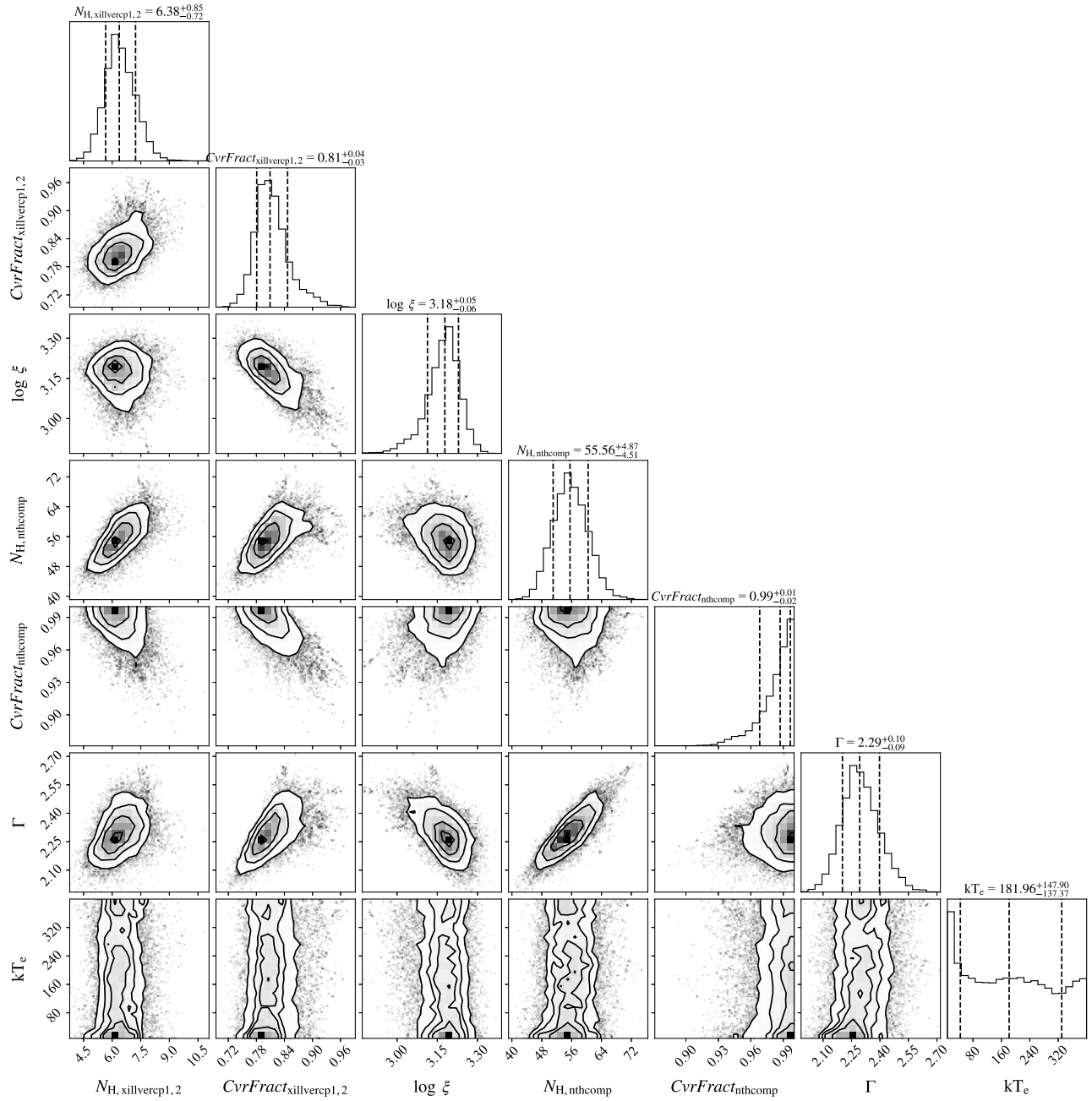
FIG. 13. Corner plot for the free parameter pairs for interval 10 after the MCMC run.
