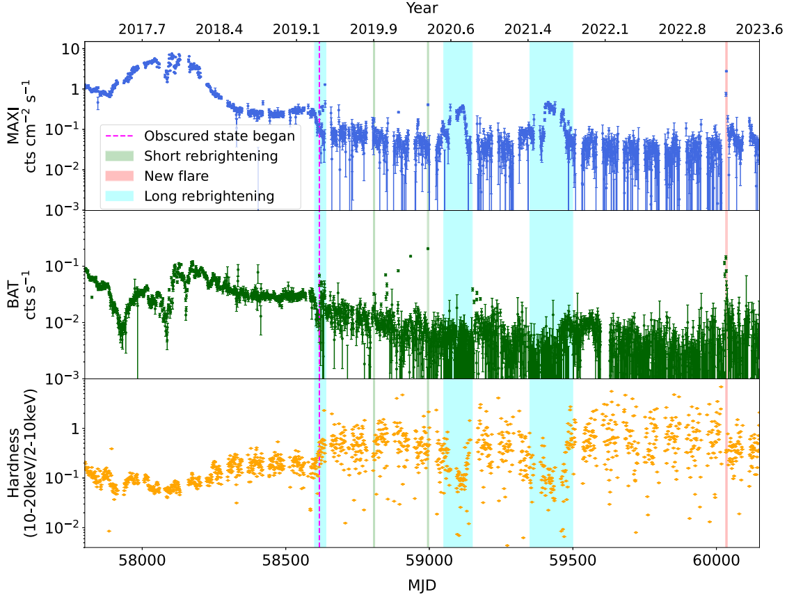
FIG. 1. Top panel: MAXI 2–20 keV flux of the source between MJD 57800 and MJD 60150. Center panel: BAT 15–150 keV flux. Bottom panel: MAXI hardness ratio (10–20 keV / 2–10 keV). The onset of the obscured state is marked by the magenta dashed line. The cyan- and green-shaded regions indicate the long and short rebrightening events reported by Athulya and Nandi [22], respectively. The pink-shaded region marks the new flare analyzed in this work observed by NICER and Swift on MJD 60034.
