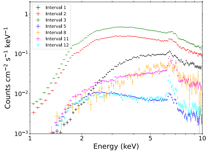
FIG. 3. Typical spectra for our observations. Different colors stand for different intervals (black, red, green, blue, orange, magenta, and cyan for intervals 1, 2, 3, 5, 8, 11, and 12, respectively). The sequence is according to the number shown in Fig. 2.
