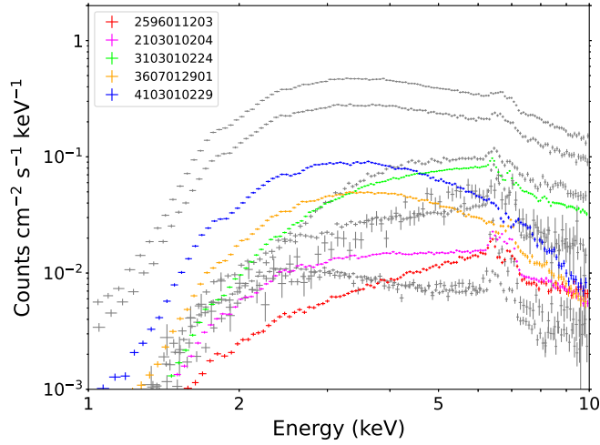
FIG. 9. Comparison of five previously reported flares from Athulya and Nandi [22] with five representative spectra. The spectra of our study are shown in gray. The spectrum from flare peak of the rebrightening phases are ObsID 2596011203 (red, long rebrightening), ObsID 2103010204 (magenta, short rebrightening), ObsID 3103010224 (green, short rebrightening), ObsID 3607012901 (orange, long rebrightening), and ObsID 4103010229 (blue, long rebrightening). The order of ObsID is based on time of rebrightening in Fig. 1.
