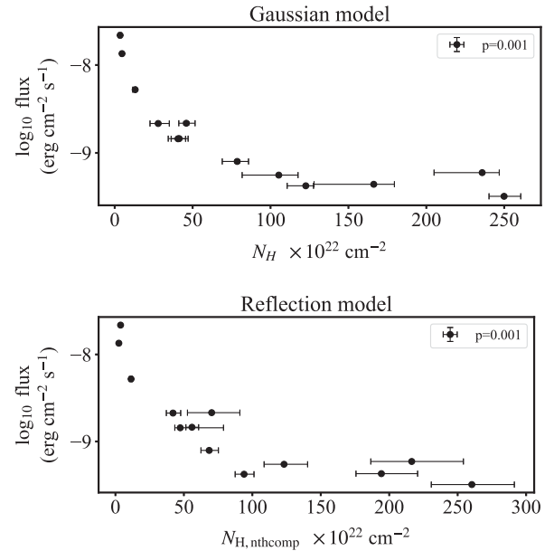
FIG. 8. Pearson correlation coefficient test for the relation between the observed x-ray flux and column density of the local absorber N_H . Upper panel: Relation between N_H and observed flux for the Gaussian-based model. Lower panel: Relation between N_{H,3} for nthcomp and observed flux for reflection-based model.
