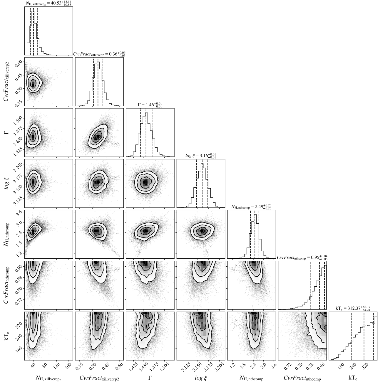
FIG. 10. Corner plot for the free parameter pairs for interval 2 after the MCMC run.
