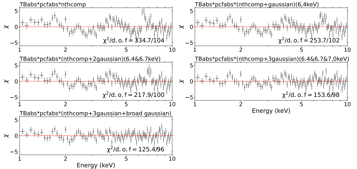
FIG. 4. Examples of spectral residuals for interval 9. The residuals are shown in black. The upper left panel shows the residual when fitting data with a baseline model, TBabs*pcfabs*nthcomp , which reveals prominent residuals at 6.4, 6.7, and 7.0 keV. The line energies were allowed to vary within \pm 0.05 keV. For each narrow line, the line width was fixed at \sigma = 0.01 keV. The broad Gaussian component was fixed at 6.4 keV with \sigma > 0.1 keV.
