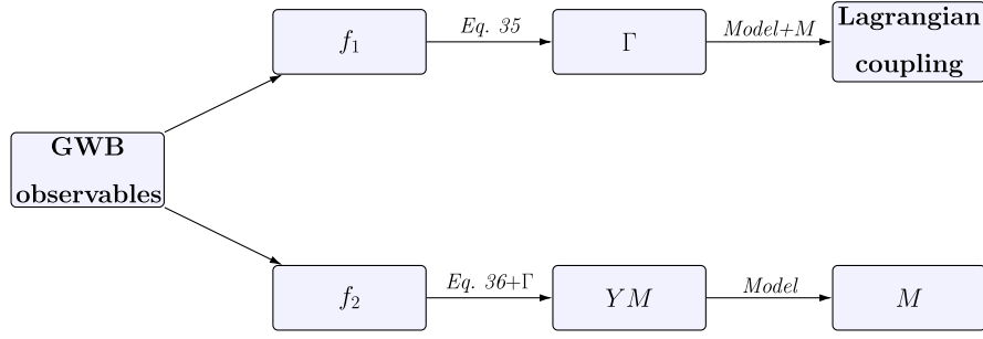
FIG. 5. Schematic showing how gravitational-wave-background observables can be mapped onto particle-physics parameters. The characteristic frequency f_1 , associated with the end of early matter domination, determines the decay rate \Gamma through Eq. (35). For a freely propagating GWB, the characteristic frequency f_2 , associated with the onset of early matter domination, determines the product Y_i M through Eq. (36) once \Gamma is known. Separating Y_i M into the particle mass M and initial abundance Y_i , and relating \Gamma to an underlying Lagrangian coupling, require specification of the particle model and production mechanism.
