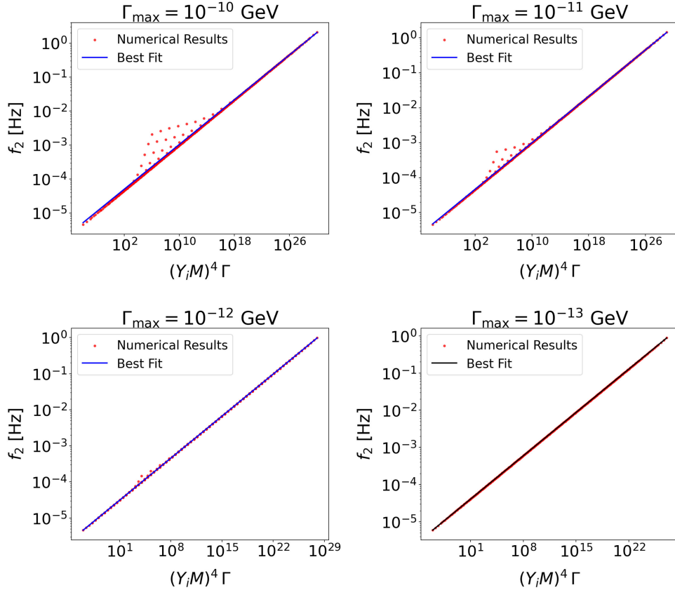
FIG. 7. Scan of f_2 for different maximum decay rates \Gamma = 10^{-10}, 10^{-11}, 10^{-12}, 10^{-13} (ordered left to right, top to bottom). The maximum \Gamma that gives early matter domination is approximately \Gamma_{\text{max}} = 10^{-10} GeV. We can see that values of gamma close to this bound do not lie on the best fit line; it is not until 2 orders of magnitude below that this can be seen as a good fit.
