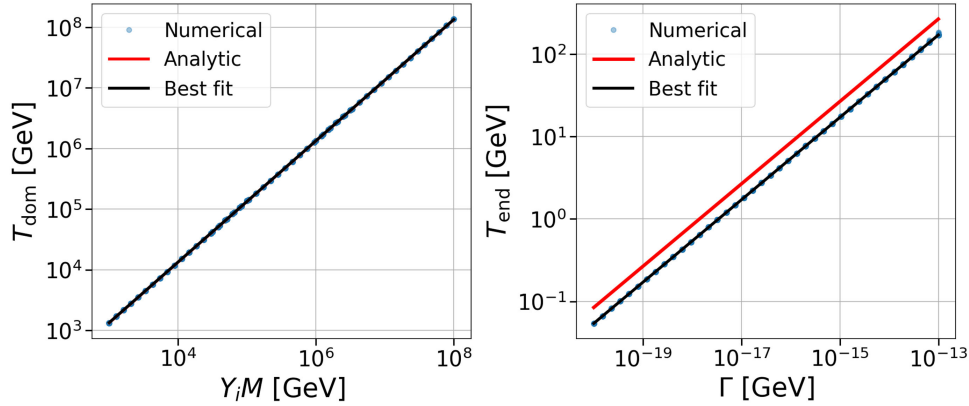
FIG. 2. Scan for early matter domination by a heavy long-lived BSM particle. Parameters T_i = 100M and scanned over the \Gamma, M, Y_i parameter space. We fixed g_X = 1 ; however this is larger independent of the results as is the initial temperature so long as the species begins as relativistic. As with the analytical estimate the domination temperature is determined by the product of mass and initial abundance, and the final temperature is determined by the decay rate, however with slightly reduced prefactors. Further discussion is given in the text.
