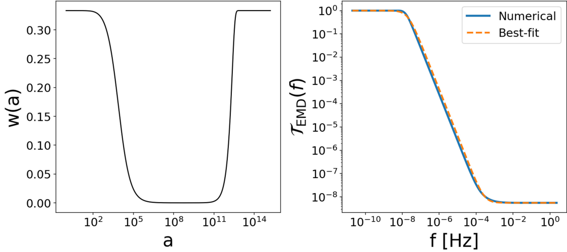
FIG. 6. Benchmark evolution of the dilution factor \mathcal{T}_{\text{EMD}} in Eq. (30) of the main text for the initial parameters Y_i = 10^{-2} , M = 10^6 GeV, and \Gamma = 10^{-18} GeV. Left panel: evolution of the equation-of-state parameter. Right panel: numerical evaluation of the dilution factor \mathcal{T}_{\text{EMD}}(f) as a function of frequency together with the corresponding best-fit function, demonstrating excellent agreement between the numerical result and the fit.
