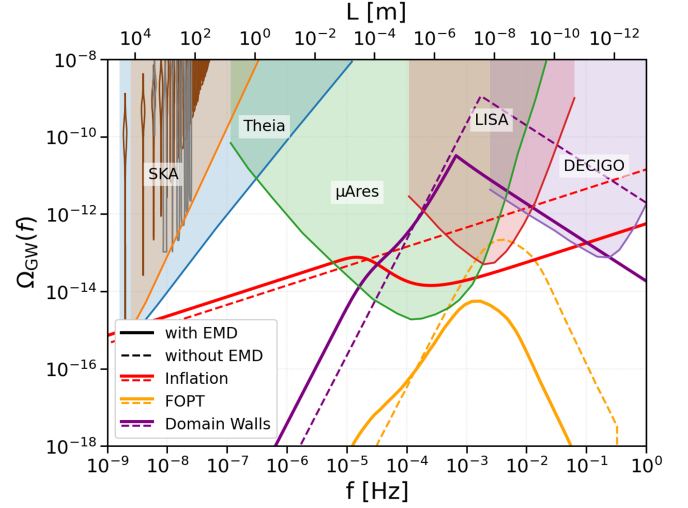
FIG. 3. Benchmark GWBs with (solid lines) and without (dashed lines) an early matter-dominated era. Results are shown for inflationary (red), first-order phase transitions (orange), and domain wall (purple). The shaded regions indicate the projected sensitivity of each detector, with the corresponding experiments labeled. Parameters for each benchmark are shown in Table II. The upper x axis indicates the location of the first feature for a particle with decay length L .
