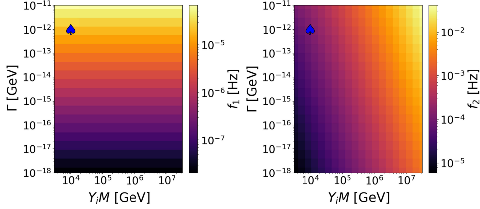
FIG. 4. Scan of the characteristic frequencies over decay rate and product of mass and initial abundance recording the frequencies of the best fit parameters. We can see that f_1 is solely dependent on the decay rate corresponding to the end of early matter domination and that f_2 has a main dependence on Y_i M and a mild dependence on the decay rate. The benchmark used in Fig. 3 is denoted by the blue spade. Further discussion is given in the text.
