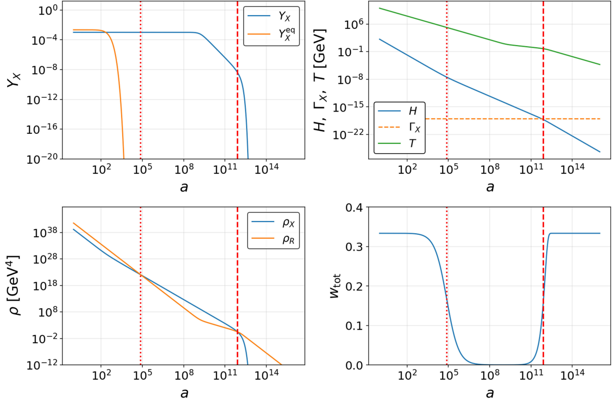
FIG. 1. Benchmark result for early matter domination by a heavy long-lived BSM particle. Plots show the evolution of the abundances (top left), the Hubble parameter and temperature (top right), the physical energy densities (bottom left) and the equation of state parameter (bottom right). The dotted and dashed red vertical lines mark the beginning and end of the early matter-dominated era, respectively. Parameters are M_X = 10^8 GeV, Y_i = 10^{-3} , \Gamma = 10^{-18} GeV. We fixed g_X = 1 ; however this is independent of the results. Discussion of results is given in the text.
