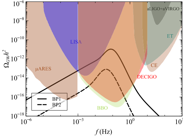
FIG. 5. Gravitational wave spectrum for benchmark points satisfying DM relic as given in Table II.
