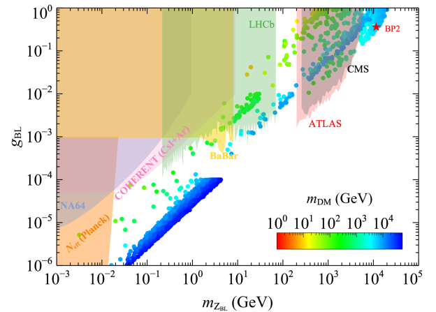
FIG. 4. Correct DM relic parameter space in g_{BL} - m_{Z_{BL}} plane. Constraints from CMS [25], ATLAS [26], LHCb [24], NA64 [27], BABAR [28], COHERENT [29], N_{\text{eff}} (Planck) [30] are shown with different shaded regions.
