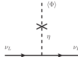
FIG. 1. Tree-level Dirac neutrino mass.
