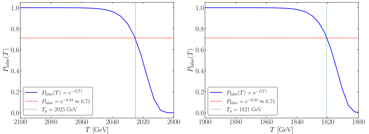
FIG. 7. False vacuum fraction P_{\text{false}}(T) = e^{-I(T)} as a function of temperature for BP1 (left) and BP2 (right). The red dashed line marks the percolation threshold P_{\text{false}} = e^{-0.34} \approx 0.71 . The vertical green dotted line indicates T_p .
