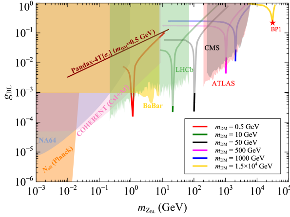
FIG. 3. Correct DM relic parameter space in g_{BL} - m_{Z_{BL}} plane for six choices of DM masses shown with different colored lines. Constraints from CMS [25], ATLAS [26], LHCb [24], NA64 [27], BABAR [28], COHERENT [29], N_{\text{eff}} (Planck) [30] are shown with different shaded regions.
