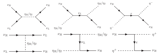
FIG. 6. Diagrams contributing to the thermalization of \nu_R .
