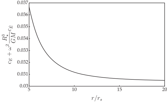
FIG. 3. Estimated evolution of c_E + \omega^2 R_*^3 / (GM) c_E as a function of the orbital length scale r . Here, c_E and c_E are computed for the AP4 EoS with GM/R_* \simeq 0.153 . We set \omega = (GM/r^3)^{1/2} and \mu = 1/r , so that the logarithmic scale dependence of c_E is evaluated at the orbital scale.
