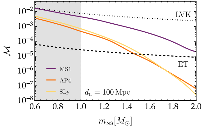
FIG. 8. Mismatch \mathcal{M} between a template that includes the dynamical tidal phase ( \Lambda_{8\text{PN}} \neq 0 ) and one that neglects it ( \Lambda_{8\text{PN}} = 0 ), as a function of the individual neutron star mass m_{\text{NS}} , for an equal-mass, nonspinning binary at d_L = 100 Mpc. Horizontal dashed lines indicate the systematic-bias threshold 1/(2\rho^2) for LVK O4 and ET, respectively. Colored lines correspond to different EoS. Systems above the ET threshold are those for which omitting the dynamical tide induces a statistically significant bias in the inference of the static Love number.
