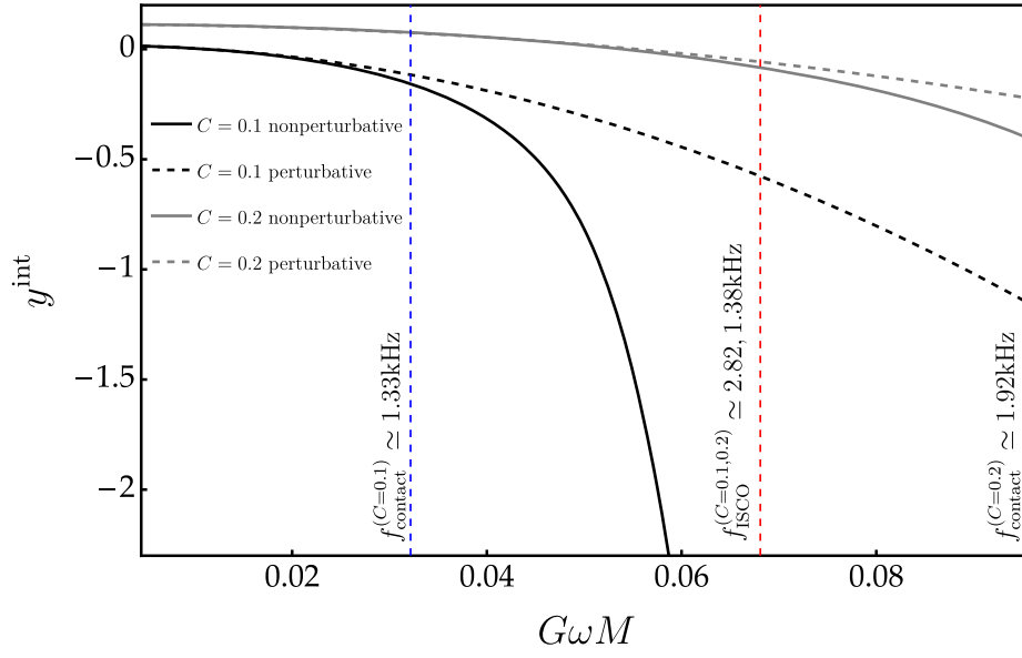
FIG. 9. Comparison between the nonperturbative (solid) and the perturbative results (dashed) for y^{\text{int}} given in Eq. (32), for a neutron star with AP4 EoS and two representative values of compactness, C = 0.1 (black) and C = 0.2 (gray), as functions of the frequency. The blue and red dashed vertical lines mark the contact frequency in Eq. (76) and the ISCO frequency in Eq. (77), respectively.
