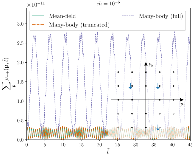
FIG. 1. Evolution of the total occupation number of right-handed neutrino states on the two-dimensional momentum grid with n_{\max} = 2 , modeled by the mean-field (solid green), truncated many-body (dash-dotted orange) and exact many-body (dashed purple) equations, for \tilde{m} = 10^{-5} . The initial configuration, shown in the lower right corner, has three left-handed (blue downarrow) neutrinos with momenta \mathbf{n}_3 = (1, -2) , \mathbf{n}_{15} = (-1, 1) , and \mathbf{n}_{17} = (1, 1) .
