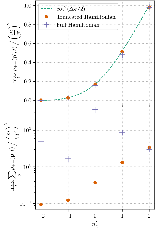
FIG. 5. Top : maximum right-handed helicity occupation number in the test momentum bin, in many-body calculations with the forward (orange dots) and full (purple crosses) Hamiltonians, for the different initial configurations shown on Fig. 4. The occupation number is normalized by (m/|\mathbf{p}'|)^2 , which is different for each calculation. The green dashed line is the mean-field prediction in Eq. (59), in perfect agreement with the truncated Hamiltonian calculation. Bottom : maximum total right-handed helicity occupation number, showing the enhancement of helicity conversion when using the full many-body Hamiltonian. We use the same normalization factor as in the top panel.
