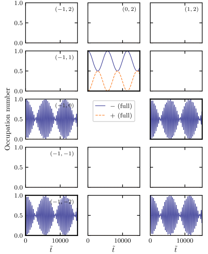
FIG. 10. Same as Fig. 7, but for the peculiar configuration discussed in Figs. 8 and 9. The results are shown for \tilde{m} = 5 \times 10^{-4} . We only display the panels where order unity occupation numbers are reached; there are also \propto \tilde{m}^2 left-handed populations in the bins (\pm 2, -1) .
