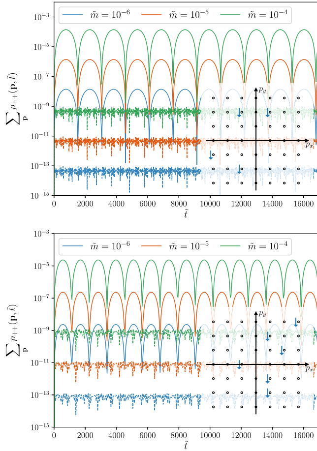
FIG. 11. Evolution of the total occupation number of right-handed states for various values of the mass parameter for the configurations shown in the bottom right corners. Solid (dashed) lines correspond to full (truncated) many-body calculations.
