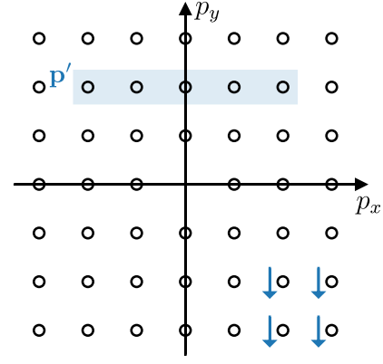
FIG. 4. Initial configurations considered for the calculations in Sec. III C. There are initially 5 occupied momentum states with left-handed neutrinos: 4 in the bottom right corner, on or close to the direction (+1, -1) , and a fifth one that will change from calculation to calculation. This fifth momentum state, denoted \mathbf{p}' , is located in the blue band, and has coordinates (n'_x \in [-2, 2], n'_y = 2) .
